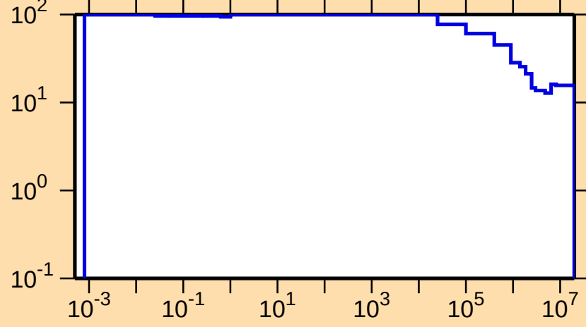
\Delta\sigma/\sigma vs. E for ^{227}\text{Th}(n,\text{nonel.})
