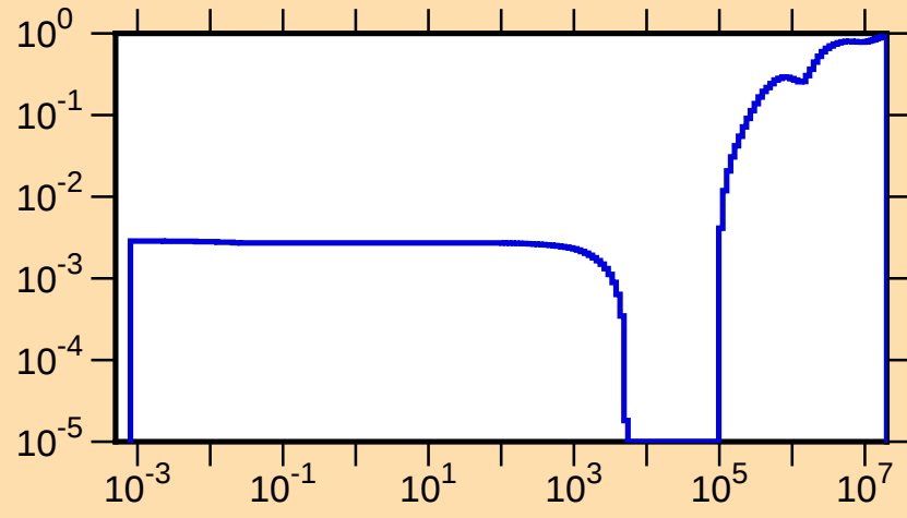
\mu vs. E for ^{234}\text{Th}(\text{mt251})
