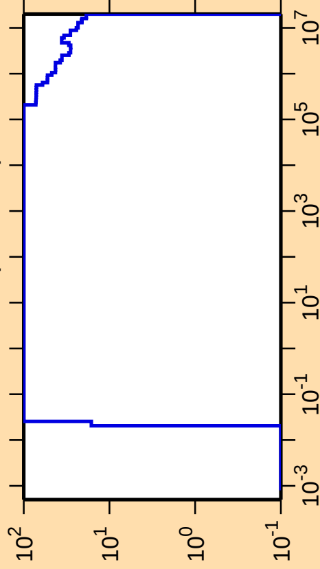
\Delta\sigma/\sigma vs. E for ^{234}\text{Th}(n,\text{nonel.})
