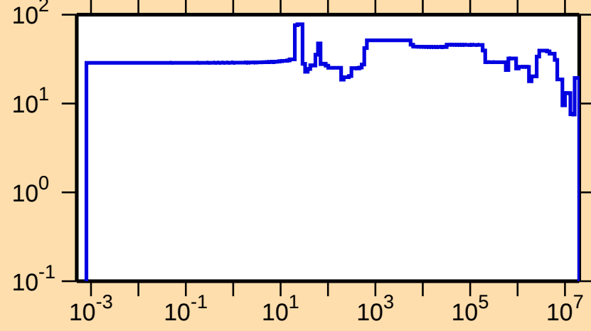
\Delta\sigma/\sigma vs. E for ^{234}\text{Th}(n,\text{el.})
