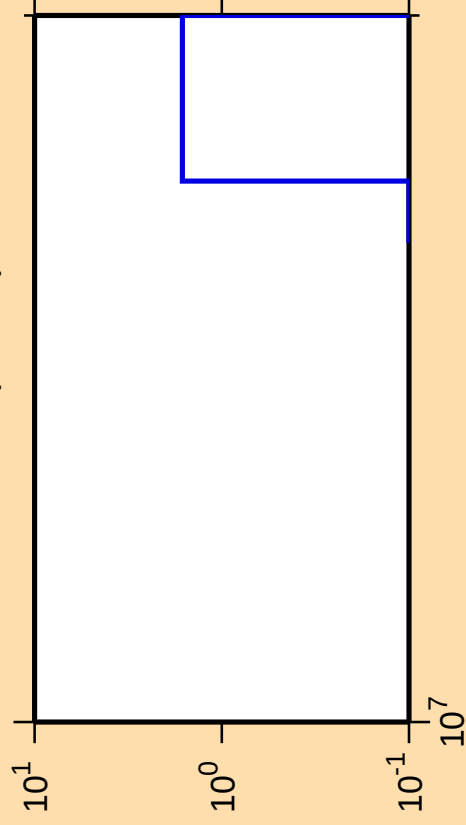
\Delta\sigma/\sigma vs. E for ^{234}\text{Th}(n,3n\alpha)
