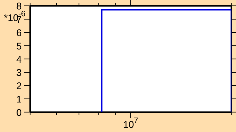
\sigma vs. E for ^{234}\text{Th}(n,d)
