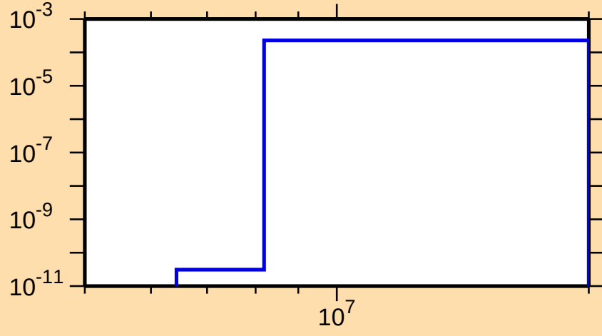
\sigma vs. E for ^{234}\text{Th}(n,p)
