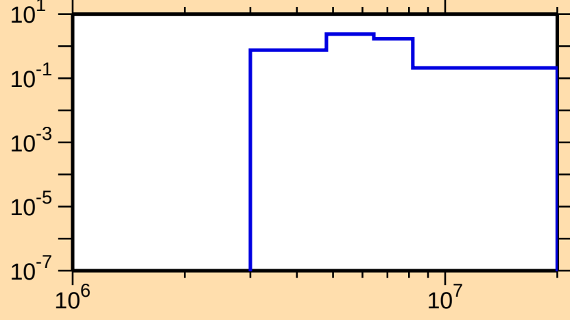
\sigma vs. E for ^{234}\text{Th}(n,n\text{cont.})
