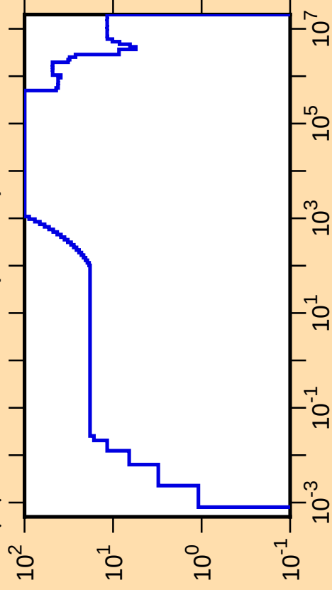
\Delta\mu/\mu vs. E for ^{238}\text{Th}(\text{mt251})
