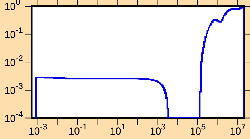
\mu vs. E for ^{238}\text{Th}(\text{mt251})
