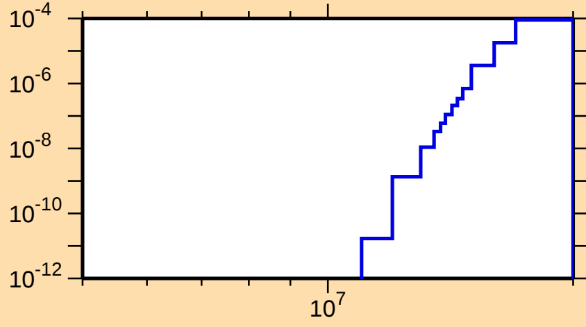
\sigma vs. E for ^{238}\text{Th}(n,d)
