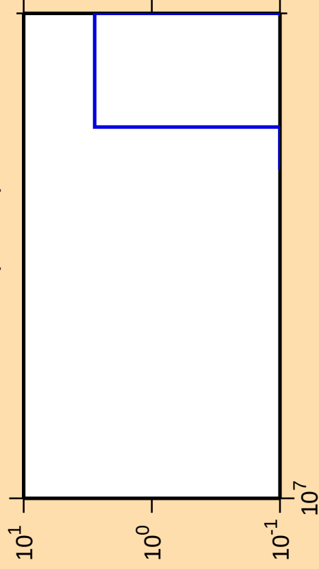
\Delta\sigma/\sigma vs. E for ^{238}\text{Th}(n,3n\alpha)
