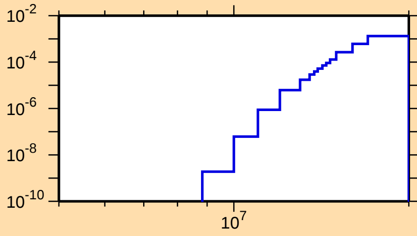
\sigma vs. E for ^{238}\text{Th}(n,p)
