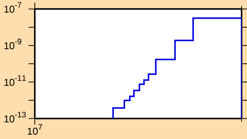
\sigma vs. E for ^{238}\text{Th}(n,2n\alpha)
