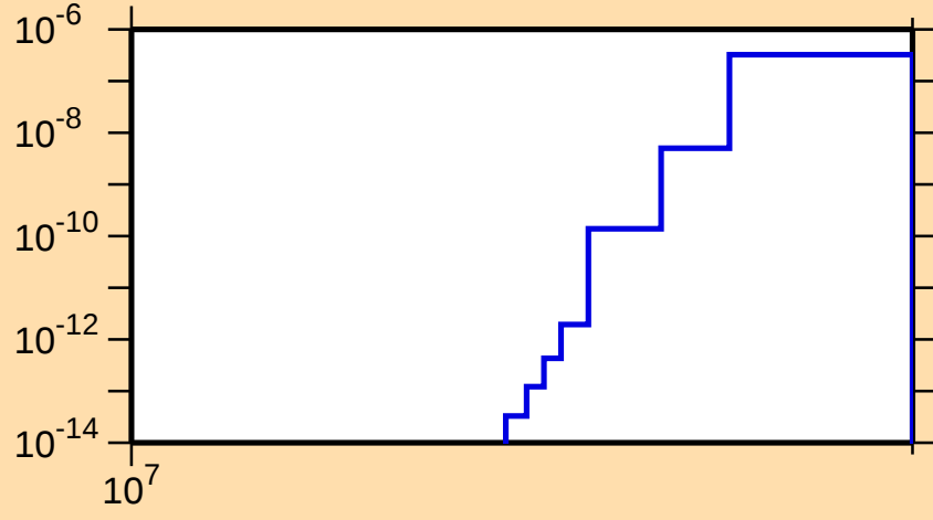
\sigma vs. E for ^{238}\text{Th}(n,\text{nt})
