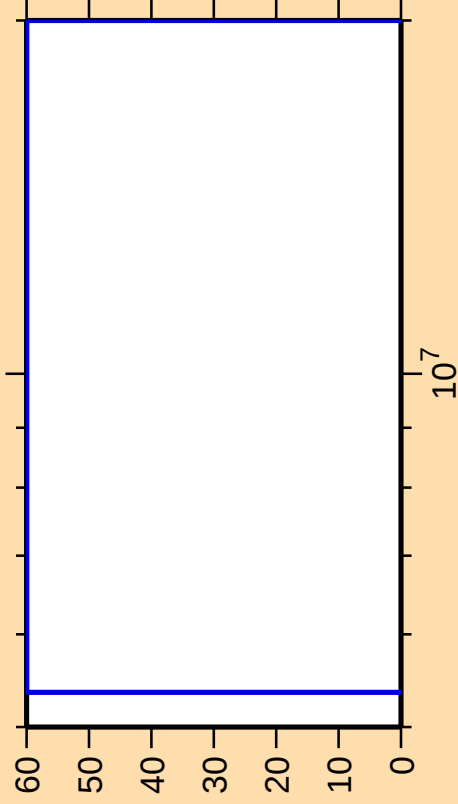
\Delta\sigma/\sigma vs. E for ^{238}\text{Th}(n,2n)
