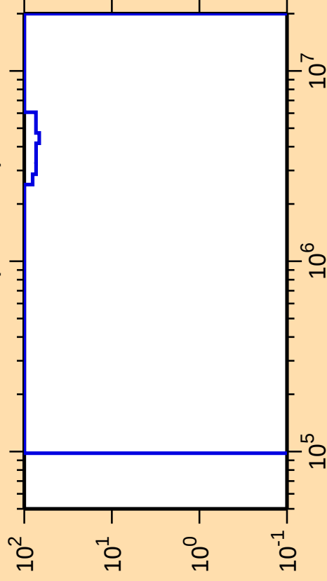
\Delta\sigma/\sigma vs. E for ^{238}\text{Th}(n,\text{ncont.})
