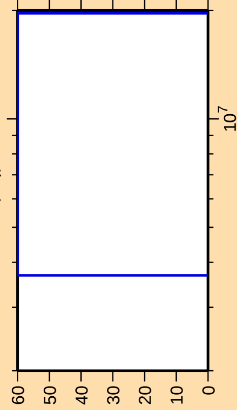
\Delta\sigma/\sigma vs. E for ^{238}\text{Th}(n,\gamma)
