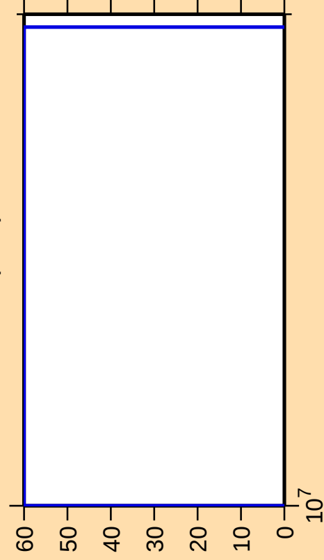
\Delta\sigma/\sigma vs. E for ^{238}\text{Th}(n,\text{nt})
