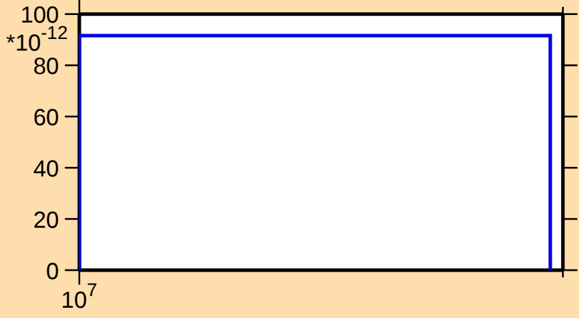
\sigma vs. E for ^{238}\text{Th}(n,\text{nd})
