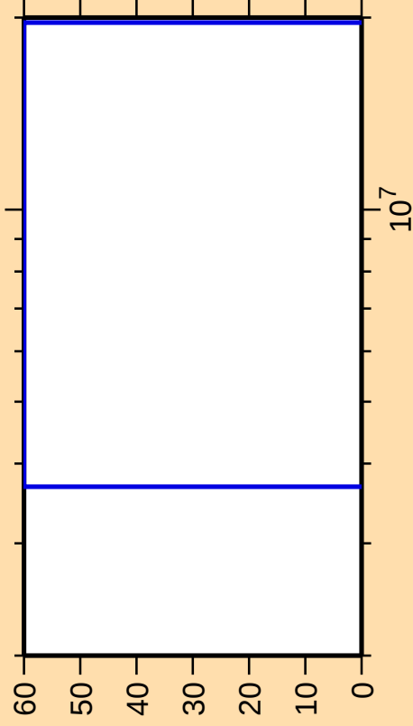
\Delta\sigma/\sigma vs. E for ^{238}\text{Th}(n,n\text{cont.})
