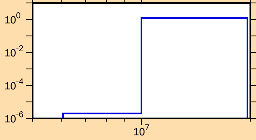
\sigma vs. E for ^{238}\text{Th}(n,3n)
