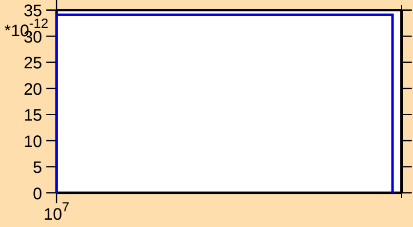
\sigma vs. E for ^{238}\text{Th}(n,2np)
