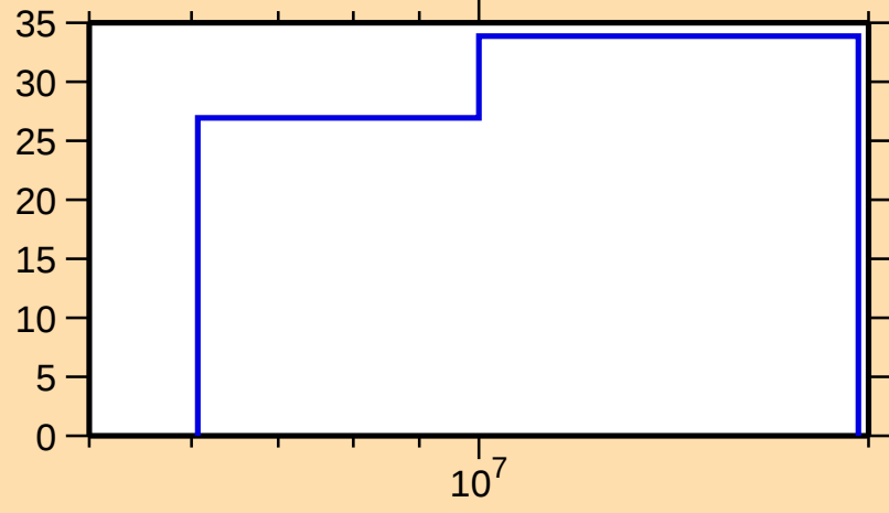
\Delta\sigma/\sigma vs. E for ^{238}\text{Th}(n,\text{tot.})
