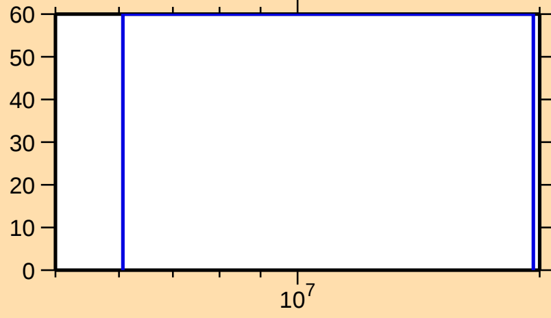
\Delta\sigma/\sigma vs. E for ^{238}\text{Th}(n,\gamma)
