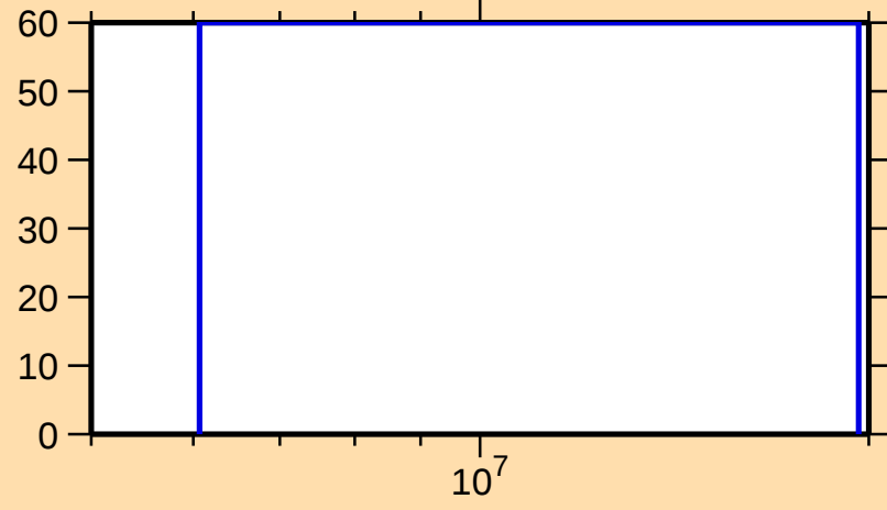
\Delta\sigma/\sigma vs. E for ^{238}\text{Th}(n,p)
