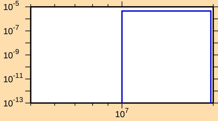
\sigma vs. E for ^{238}\text{Th}(n,t)
