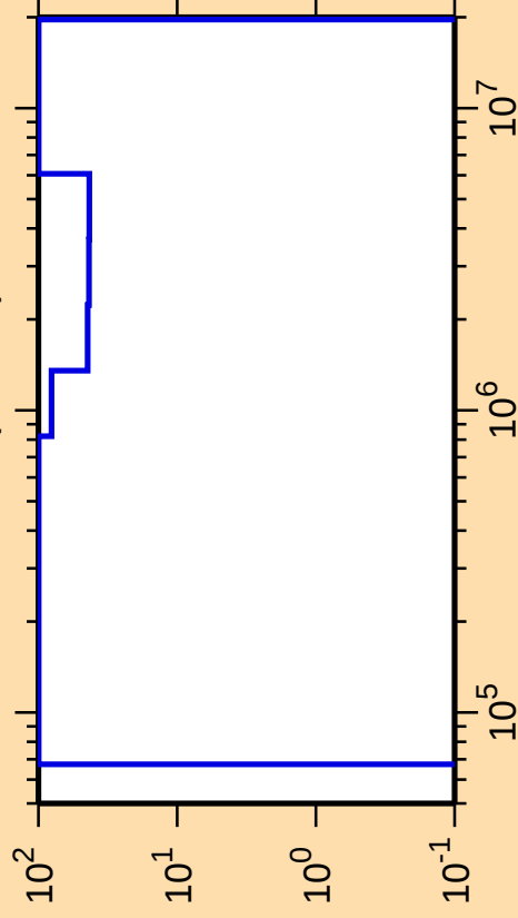
\Delta\sigma/\sigma vs. E for ^{238}\text{Th}(n,\text{inel.})
