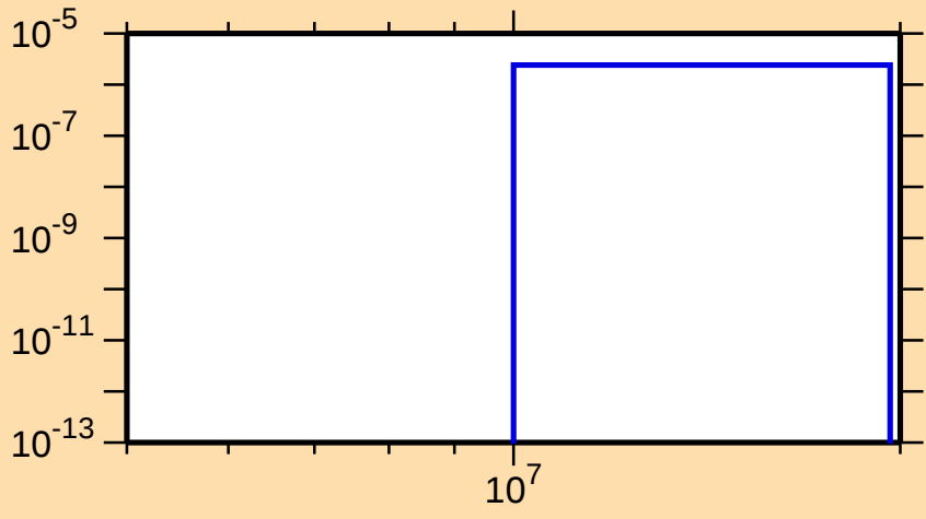
\sigma vs. E for ^{238}\text{Th}(n,d)
