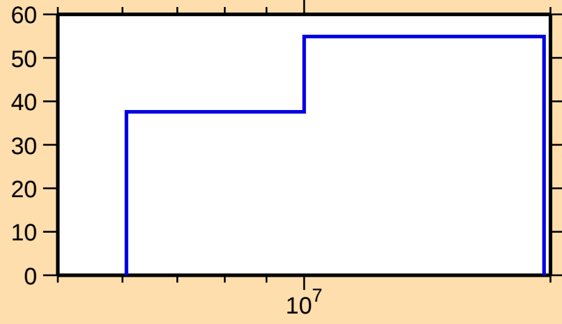
\Delta\sigma/\sigma vs. E for ^{238}\text{Th}(n,\text{el.})
