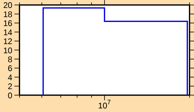
\Delta\sigma/\sigma vs. E for ^{238}\text{Th}(n,\text{nonel.})
