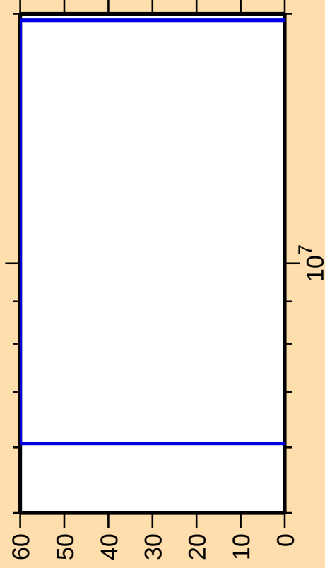
\Delta\sigma/\sigma vs. E for ^{238}\text{Th}(n,p)
