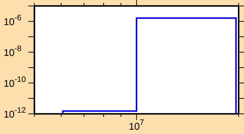
\sigma vs. E for ^{238}\text{Th}(n,\alpha)
