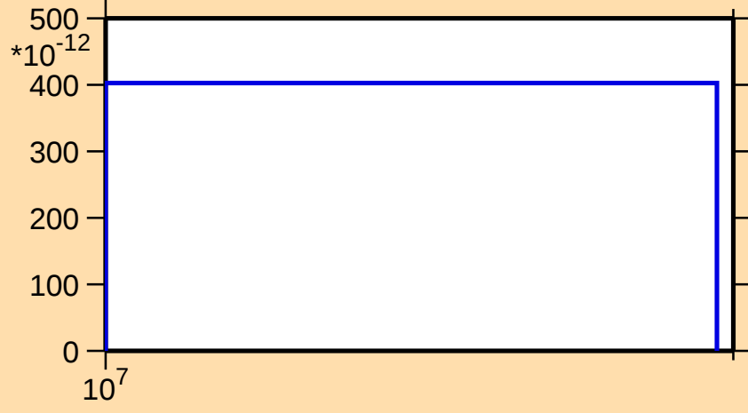
\sigma vs. E for ^{238}\text{Th}(n,2n\alpha)
