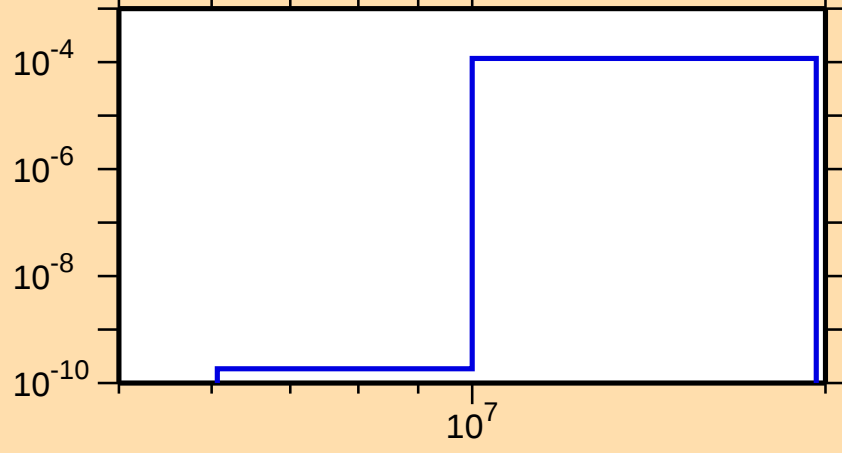
\sigma vs. E for ^{238}\text{Th}(n,p)
