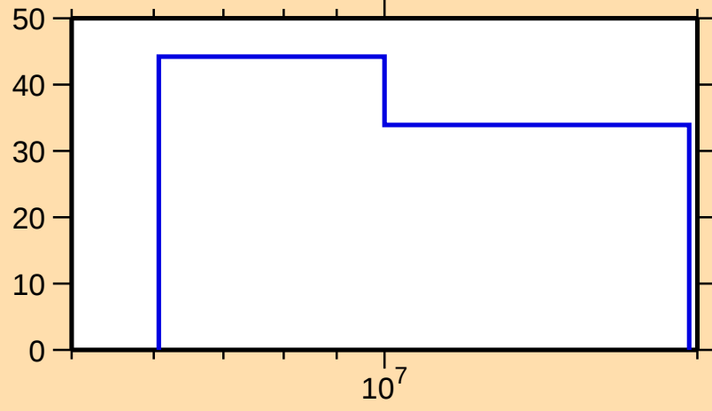
\Delta\sigma/\sigma vs. E for ^{238}\text{Th}(n,n_1)
