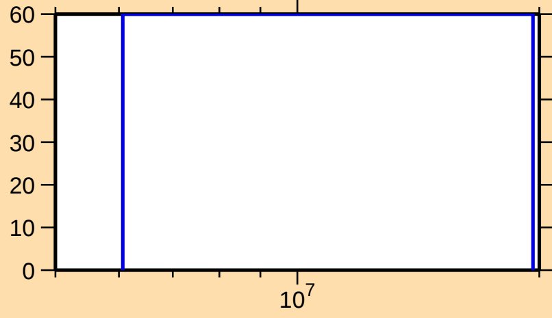
\Delta\sigma/\sigma vs. E for ^{238}\text{Th}(n,n\text{cont.})
