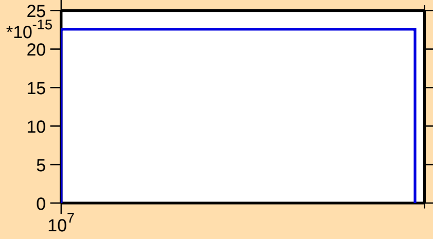
\sigma vs. E for ^{238}\text{Th}(n,3n\alpha)
