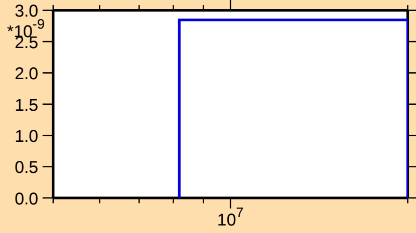
\sigma vs. E for ^{238}\text{Th}(n,\text{nt})
