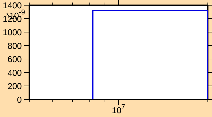
\sigma vs. E for ^{238}\text{Th}(n,n\alpha)
