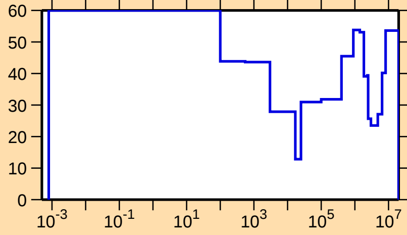
\Delta\sigma/\sigma vs. E for ^{238}\text{Th}(n,el.)
