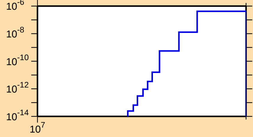
\sigma vs. E for ^{228}\text{U}(\text{n},\text{nd})
