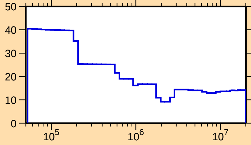
\Delta\sigma/\sigma vs. E for ^{228}\text{U}(\text{n,nonel.})
