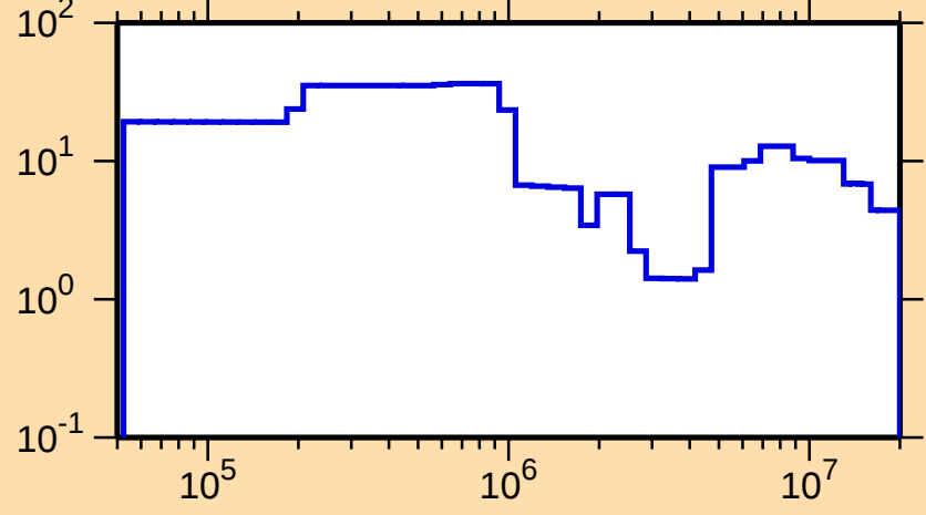
\Delta\sigma/\sigma vs. E for ^{228}\text{U}(\text{n,tot.})
