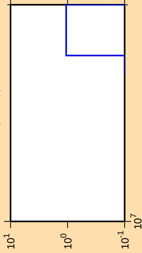
\Delta\sigma/\sigma vs. E for ^{228}\text{U} (mt 34)
