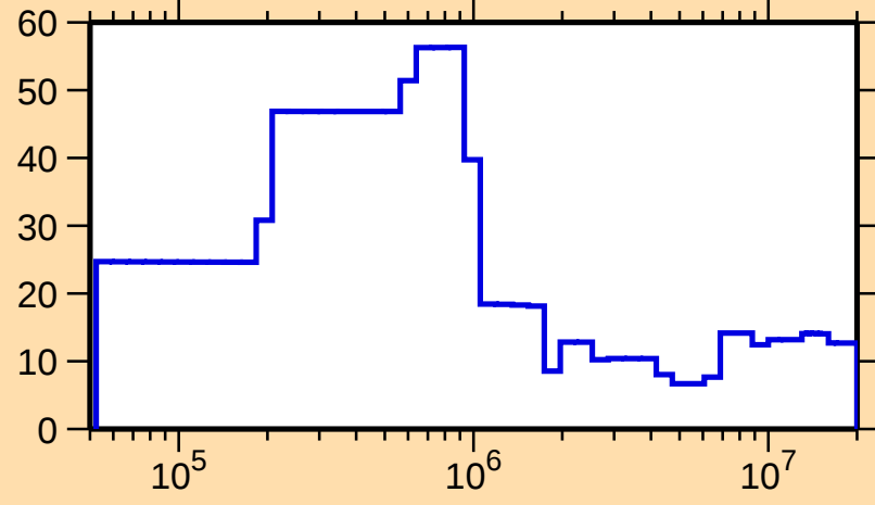
\Delta\sigma/\sigma vs. E for ^{228}\text{U}(\text{n,el.})
