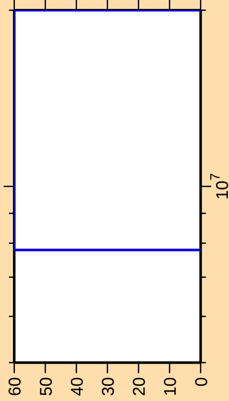
\Delta\sigma/\sigma vs. E for ^{228}\text{U}(n,f)
