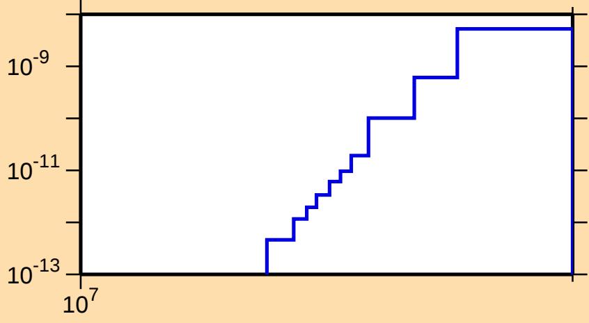
\sigma vs. E for ^{228}\text{U}(n,\text{He3})
