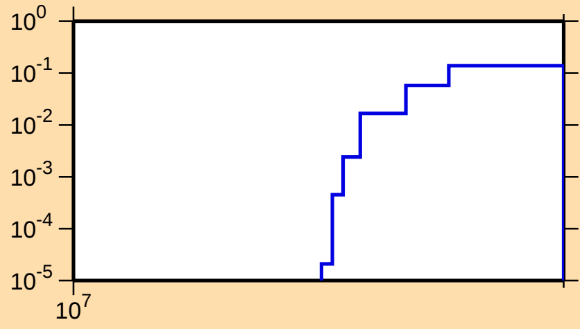
\sigma vs. E for ^{228}\text{U}(n,3n)
