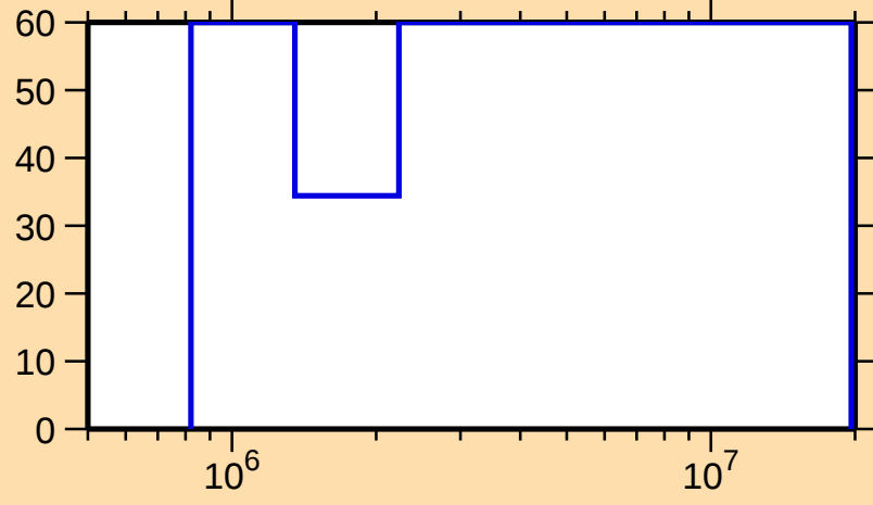
\Delta\sigma/\sigma vs. E for ^{228}\text{U}(\text{n},\text{f})
