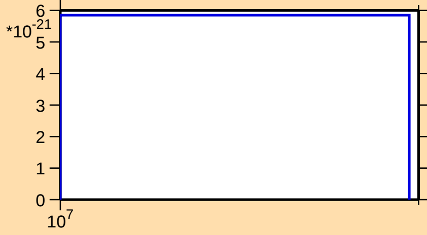
\sigma vs. E for ^{228}\text{U}(\text{mt } 42)
