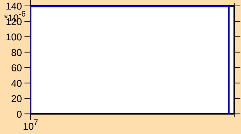
\sigma vs. E for ^{228}\text{U}(n,3n\alpha)
