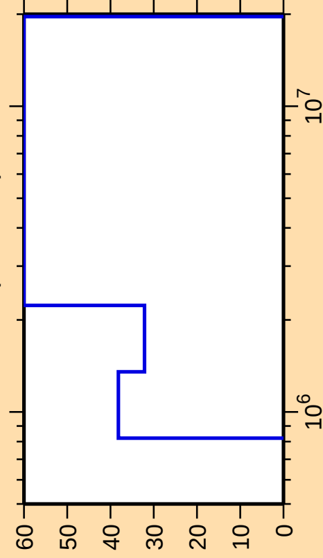
\Delta\sigma/\sigma vs. E for ^{228}\text{U}(\text{n,ncont.})
