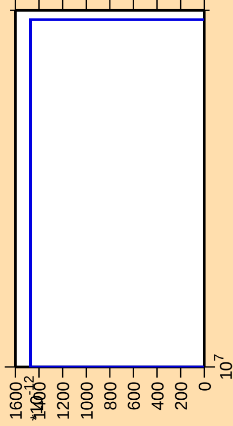
\Delta\sigma/\sigma vs. E for ^{228}\text{U}(\text{mt } 42)
