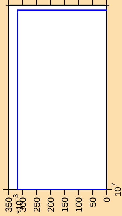
\Delta\sigma/\sigma vs. E for ^{228}\text{U}(\text{mt } 45)
