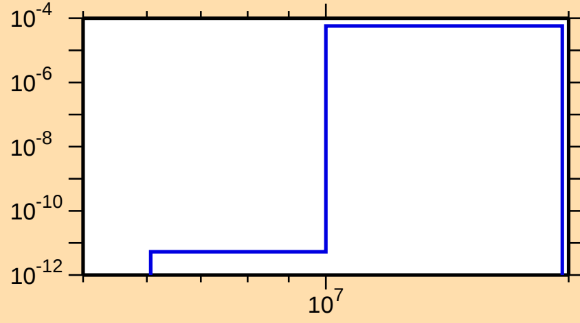
\sigma vs. E for ^{228}\text{U}(n,t)
