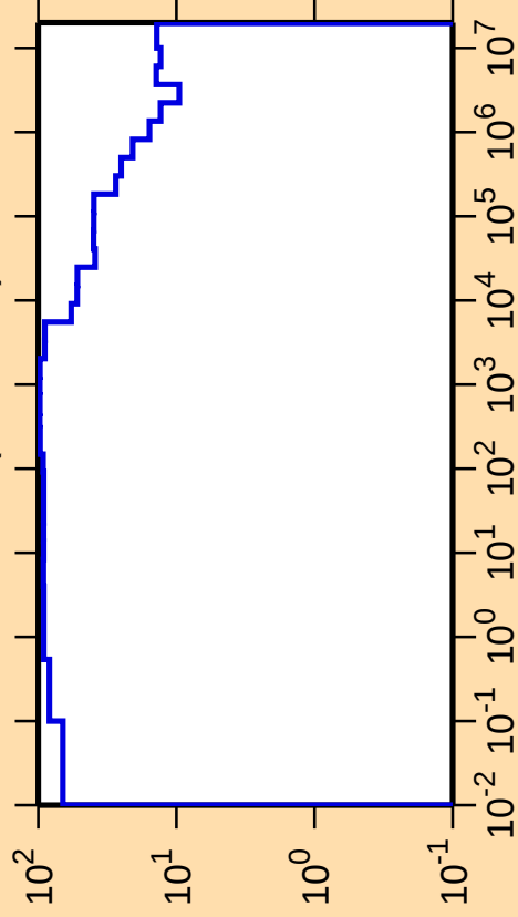
\Delta\sigma/\sigma vs. E for ^{228}\text{U}(n,\text{nonel.})
