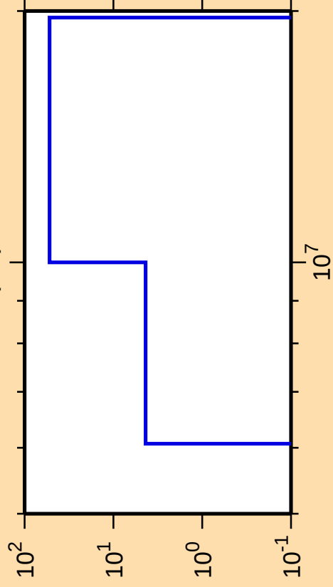
\Delta\sigma/\sigma vs. E for ^{228}\text{U}(n,t)
