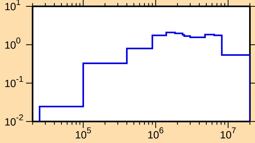
\sigma vs. E for ^{228}\text{U}(\text{n,inel.})
