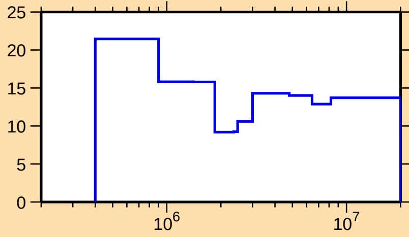
\Delta\sigma/\sigma vs. E for ^{228}\text{U}(\text{n},\text{nonel.})
