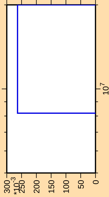
\Delta\sigma/\sigma vs. E for ^{228}\text{U}(\text{mt } 45)
