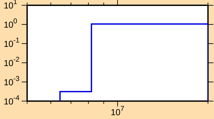
\sigma vs. E for ^{228}\text{U}(n,2n)
