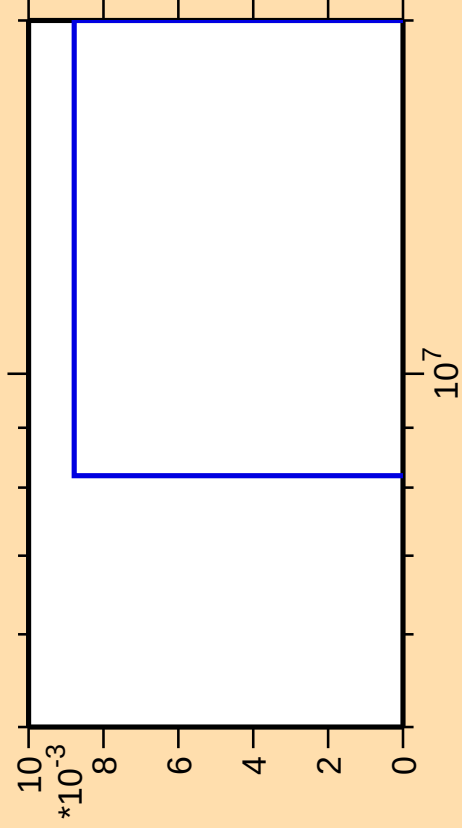
\Delta\sigma/\sigma vs. E for ^{228}\text{U}(\text{mt } 34)
