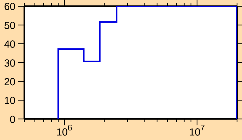
\Delta\sigma/\sigma vs. E for ^{228}\text{U}(n,ncont.)
