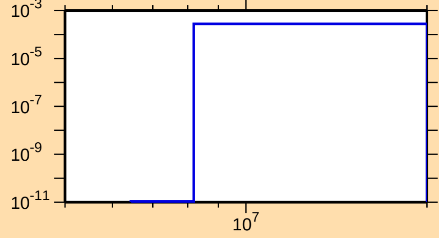
\sigma vs. E for ^{228}\text{U}(n,d)
