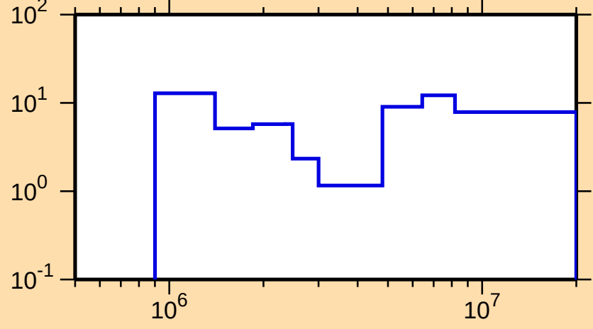
\Delta\sigma/\sigma vs. E for ^{228}\text{U}(n,\text{tot.})
