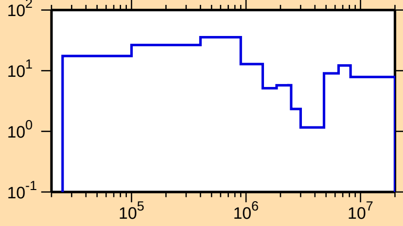
\Delta\sigma/\sigma vs. E for ^{228}\text{U}(\text{n,tot.})
