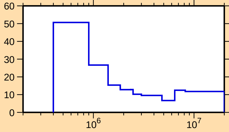
\Delta\sigma/\sigma vs. E for ^{228}\text{U}(\text{n},\text{el.})
