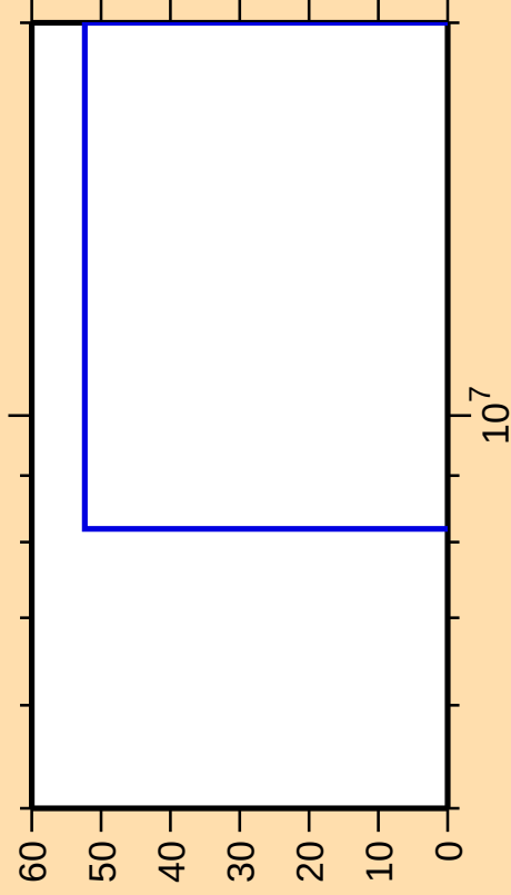
\Delta\sigma/\sigma vs. E for ^{228}\text{U}(\text{n,t})
