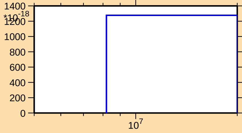
\sigma vs. E for ^{228}\text{U}(\text{mt } 34)
