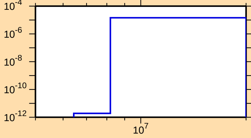
\sigma vs. E for ^{228}\text{U}(n,np)
