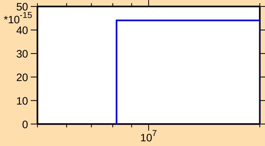
\sigma vs. E for ^{228}\text{U}(\text{mt } 45)
