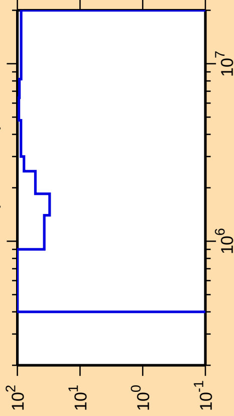
\Delta\sigma/\sigma vs. E for ^{228}\text{U}(\text{n},\text{ncont.})
