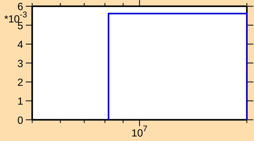
\sigma vs. E for ^{228}\text{U}(n,3n)
