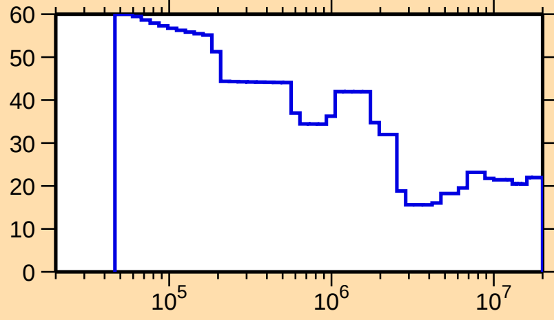
\Delta\sigma/\sigma vs. E for ^{230}\text{U}(\text{n,nonel.})
