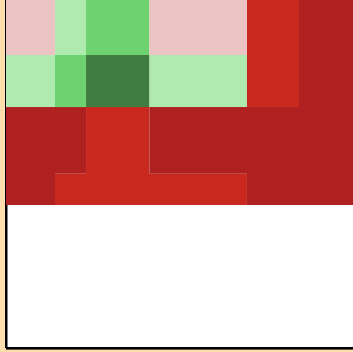
\Delta\sigma/\sigma vs. E for ^{230}\text{U}(n,\text{inel.})
