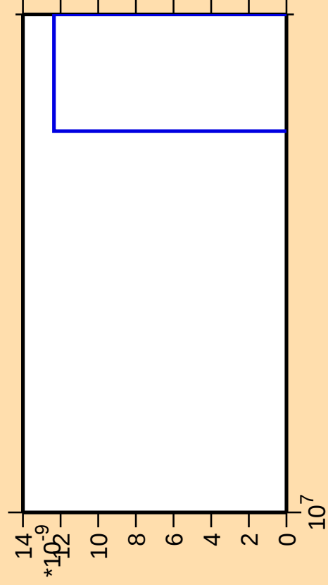
\Delta\sigma/\sigma vs. E for ^{230}\text{U} (mt 42)
