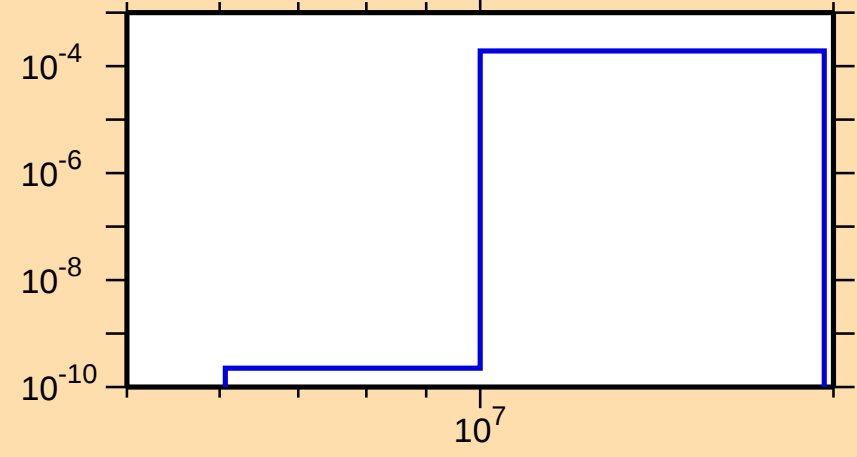
\sigma vs. E for ^{230}\text{U}(n,d)
