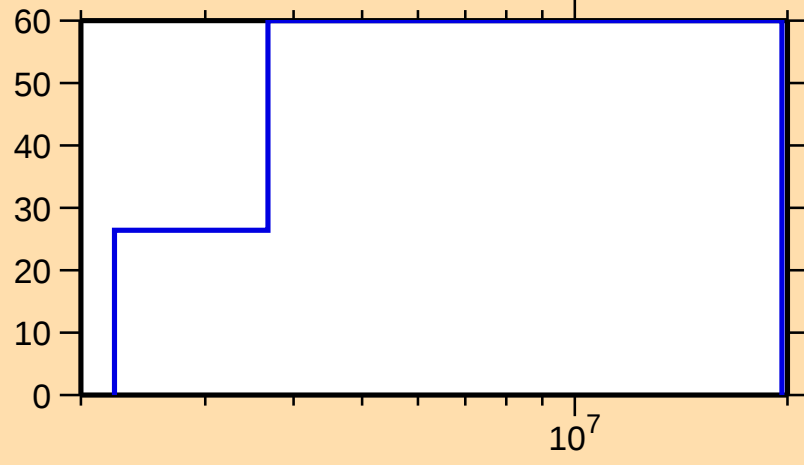
\Delta\sigma/\sigma vs. E for ^{230}\text{U}(n,p)
