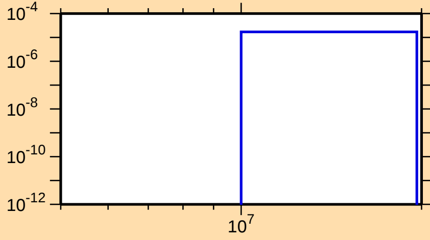
\sigma vs. E for ^{230}\text{U}(n,t)
