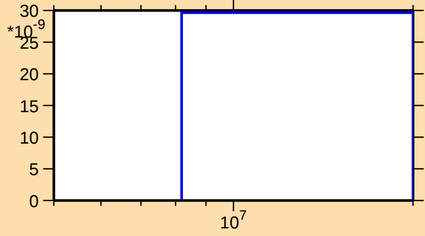
\sigma vs. E for ^{230}\text{U}(n,2n\alpha)
