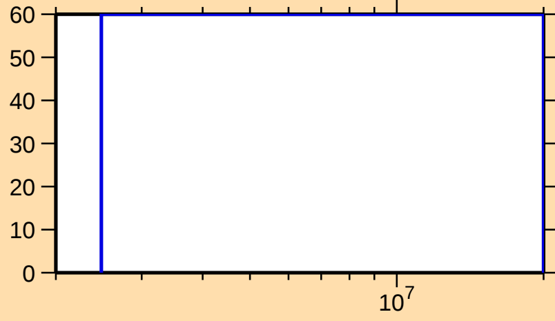
\Delta\sigma/\sigma vs. E for ^{230}\text{U}(n,\gamma)
