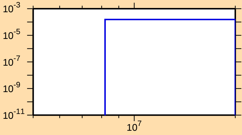
\sigma vs. E for ^{230}\text{U}(n,d)
