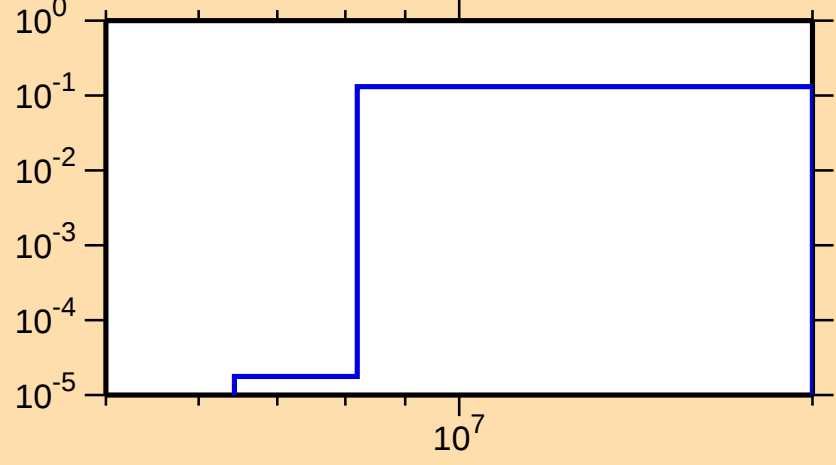
\sigma vs. E for ^{230}\text{U}(n,2n)
