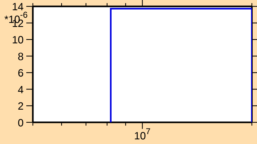
\sigma vs. E for ^{230}\text{U}(n,t)
