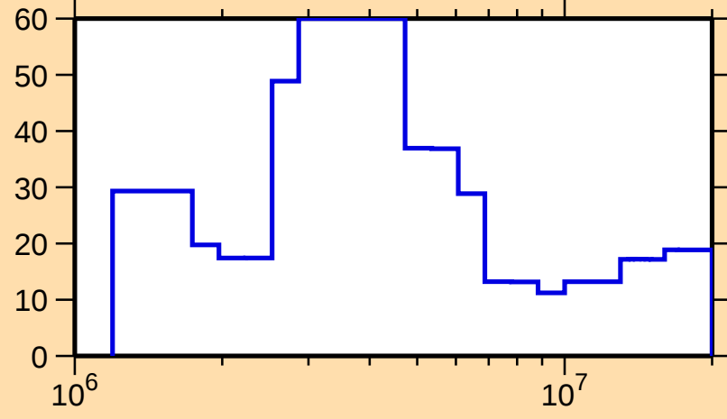
\Delta\sigma/\sigma vs. E for ^{231}\text{U}(\text{n},\text{f})
