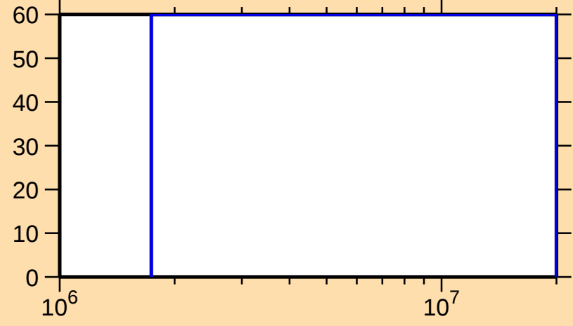
\Delta\sigma/\sigma vs. E for ^{231}\text{U}(n,ncont.)
