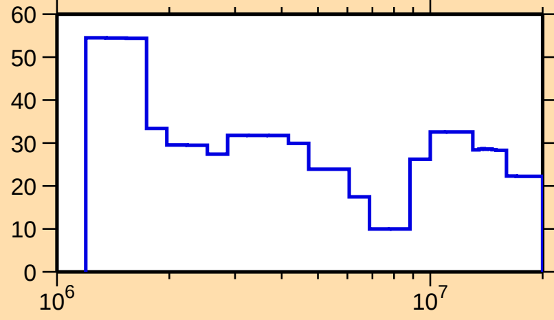
\Delta\sigma/\sigma vs. E for ^{231}\text{U}(\text{n},\text{el.})
