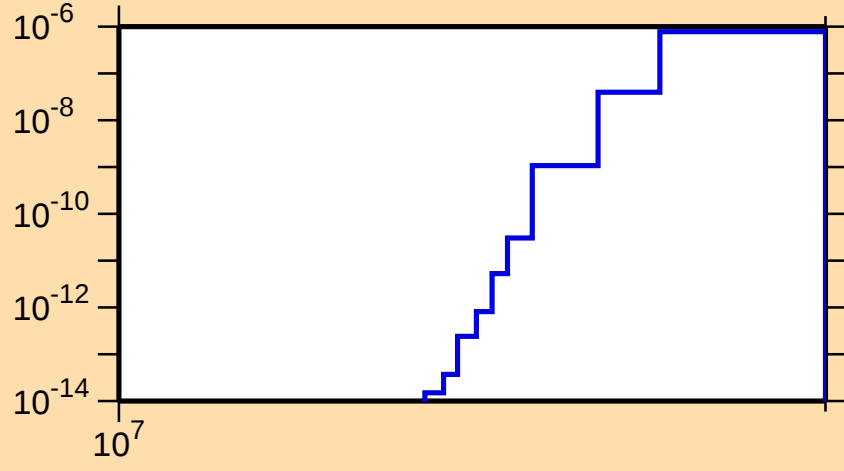
\sigma vs. E for ^{231}\text{U}(n,2np)
