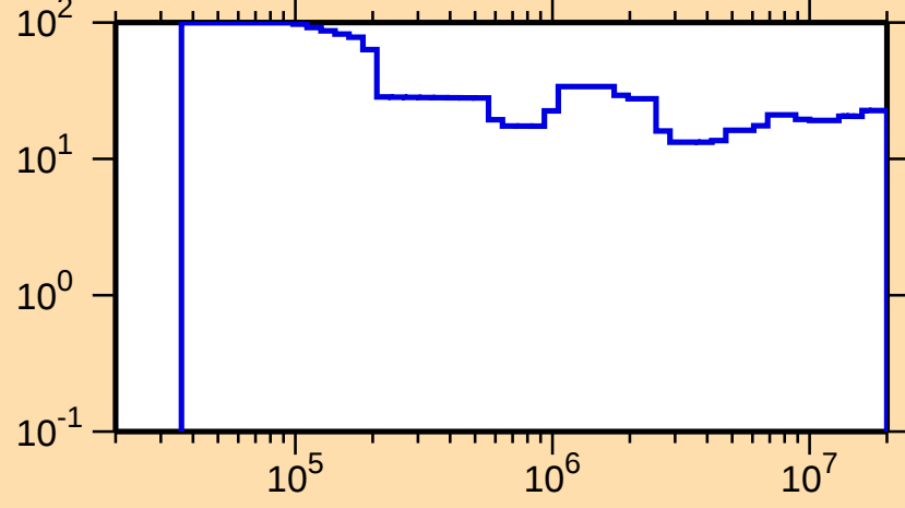
\Delta\sigma/\sigma vs. E for ^{231}\text{U}(\text{n,nonel.})
