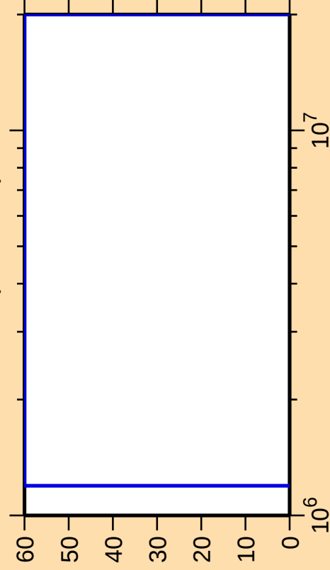
\Delta\sigma/\sigma vs. E for ^{231}\text{U}(\text{n,ncont.})
