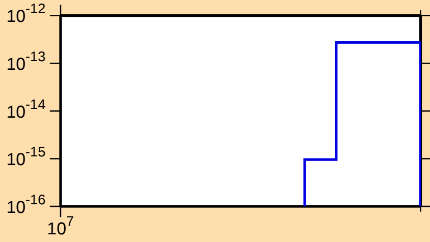
\sigma vs. E for ^{231}\text{U} (mt 34)
