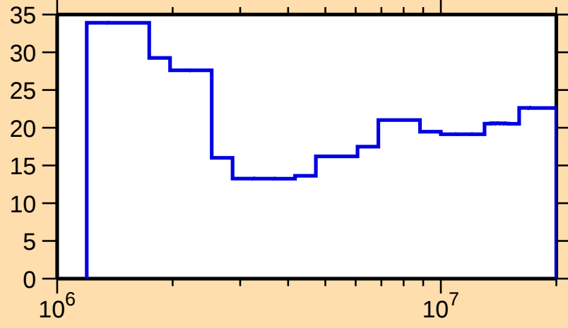
\Delta\sigma/\sigma vs. E for ^{231}\text{U}(\text{n},\text{nonel.})
