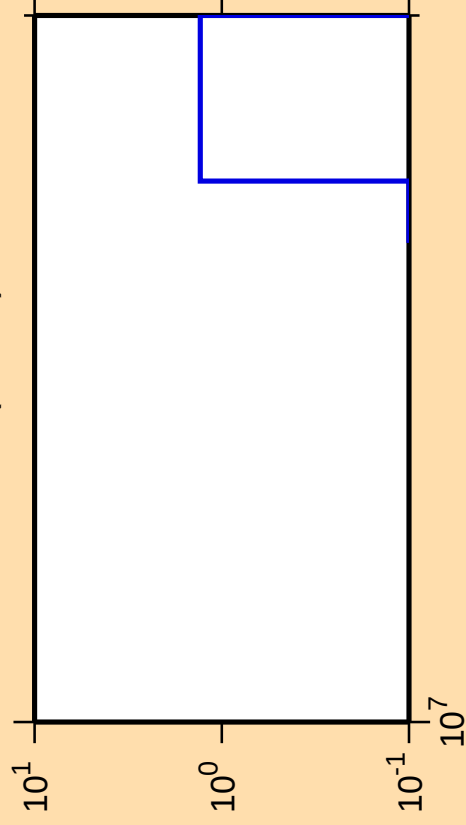
\Delta\sigma/\sigma vs. E for ^{231}\text{U} (mt 34)
