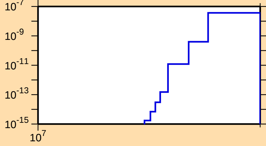
\sigma vs. E for ^{231}\text{U}(n,nt)
