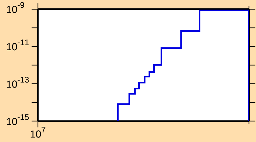
\sigma vs. E for ^{231}\text{U}(n,\text{He3})
