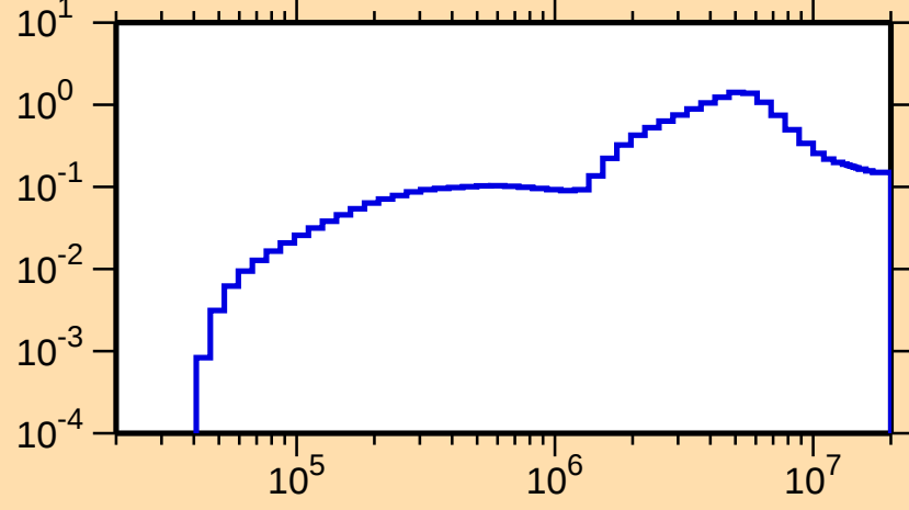
\sigma vs. E for ^{231}\text{U}(\text{n,inel.})
