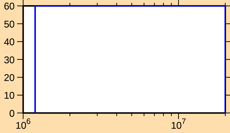
\Delta\sigma/\sigma vs. E for ^{231}\text{U}(\text{n,inel.})
