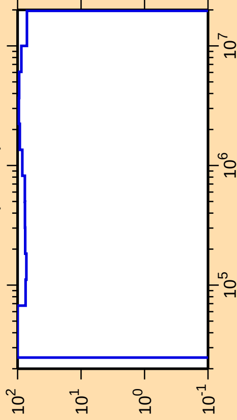
\Delta\sigma/\sigma vs. E for ^{231}\text{U}(\text{n,inel.})
