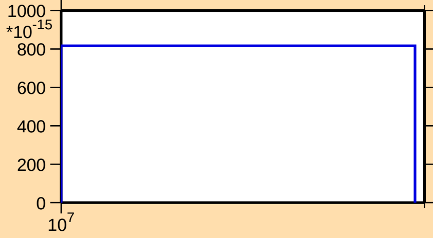
\sigma vs. E for ^{231}\text{U}(n,p\alpha)
