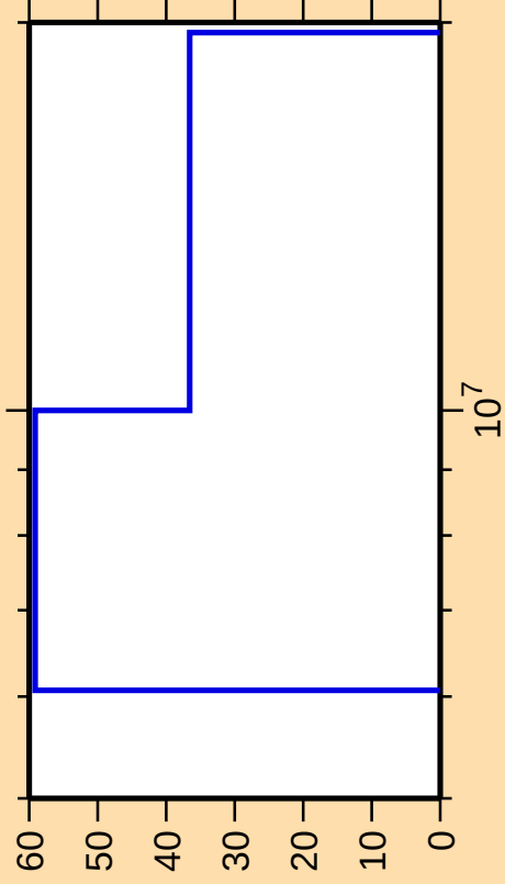
\Delta\sigma/\sigma vs. E for ^{231}\text{U}(n,d)
