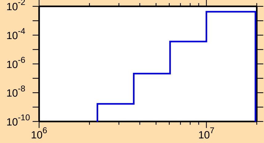
\sigma vs. E for ^{231}\text{U}(n,p)
