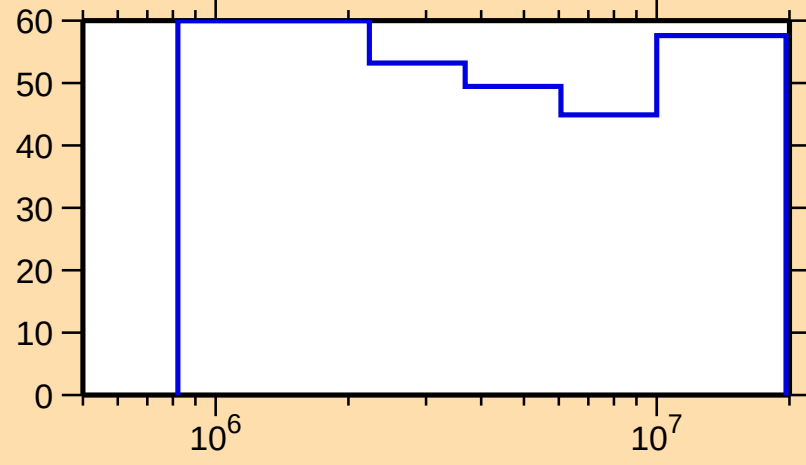
\Delta\sigma/\sigma vs. E for ^{231}\text{U}(n,n_1)
