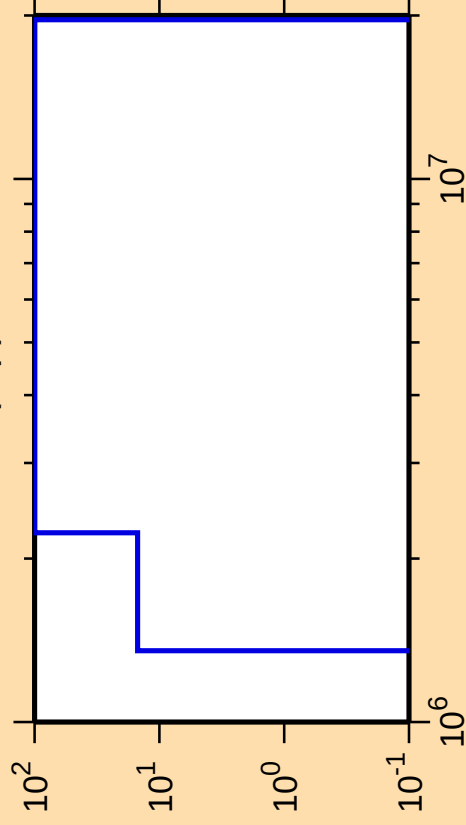
\Delta\sigma/\sigma vs. E for ^{231}\text{U}(n,p)
