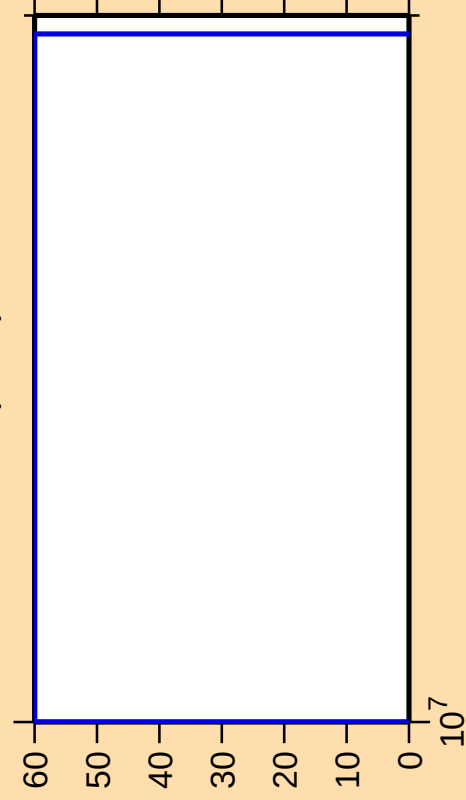
\Delta\sigma/\sigma vs. E for ^{231}\text{U}(\text{n},\text{nd})
