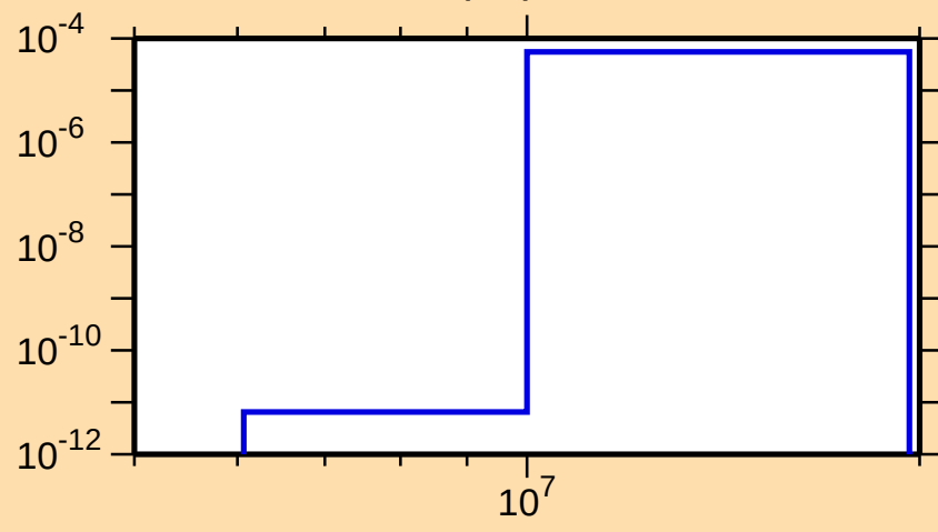
\sigma vs. E for ^{231}\text{U}(n,t)
