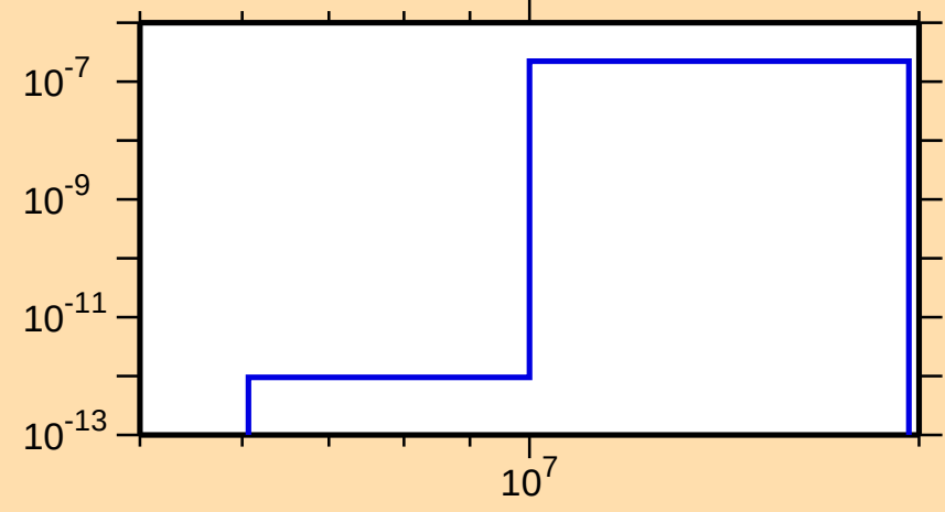
\sigma vs. E for ^{231}\text{U}(n,2n\alpha)
