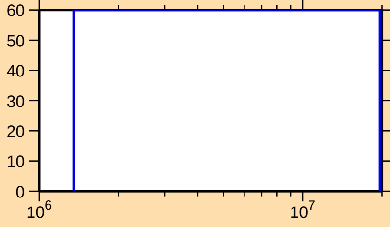
\Delta\sigma/\sigma vs. E for ^{231}\text{U}(n,\text{inel.})
