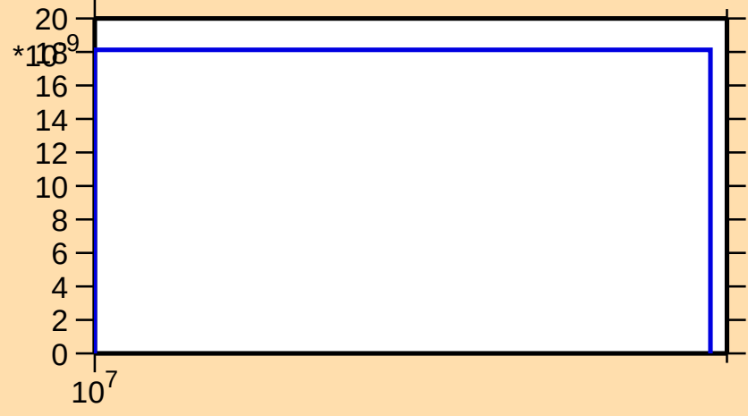
\sigma vs. E for ^{231}\text{U}(\text{n},\text{nd})
