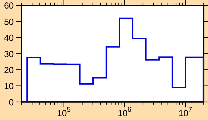
\Delta\sigma/\sigma vs. E for ^{231}\text{U}(\text{n,el.})
