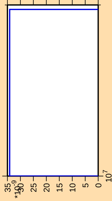
\Delta\sigma/\sigma vs. E for ^{231}\text{U}(\text{mt } 42)
