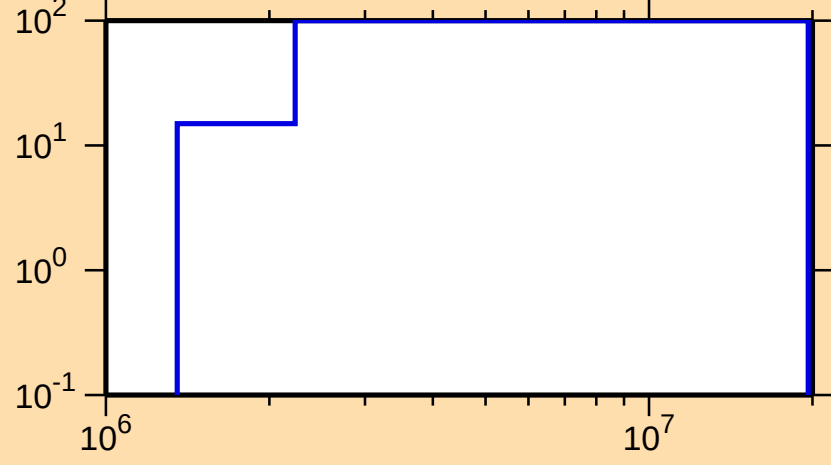
\Delta\sigma/\sigma vs. E for ^{231}\text{U}(n,p)
