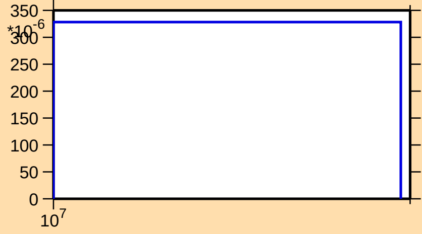
\sigma vs. E for ^{231}\text{U}(n,3n)
