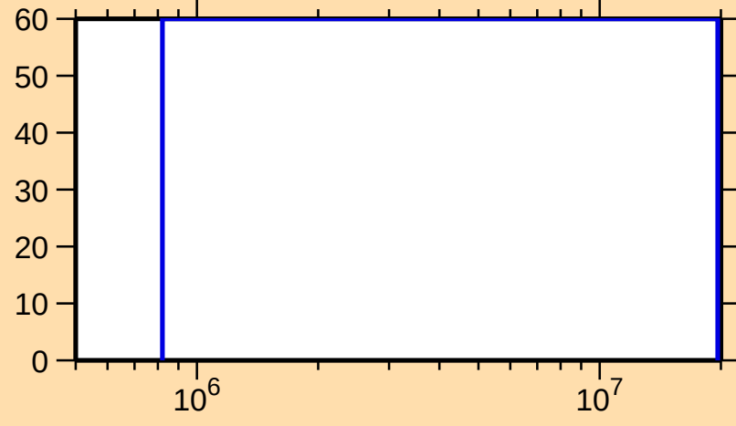
\Delta\sigma/\sigma vs. E for ^{231}\text{U}(n,n\text{cont.})
