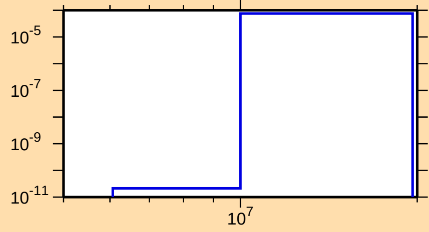
\sigma vs. E for ^{231}\text{U}(n,np)
