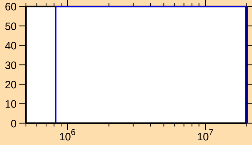
\Delta\sigma/\sigma vs. E for ^{231}\text{U}(\text{n},\text{inel.})
