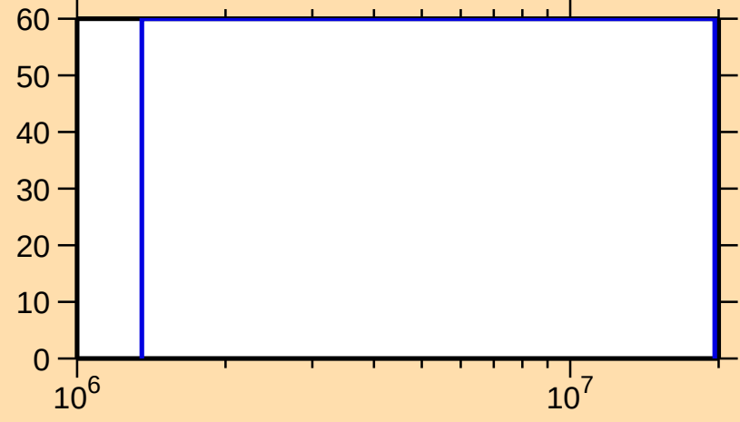
\Delta\sigma/\sigma vs. E for ^{231}\text{U}(n,\gamma)
