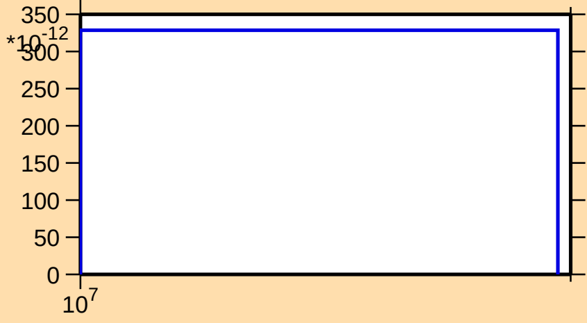
\sigma vs. E for ^{231}\text{U}(\text{n},\text{nt})
