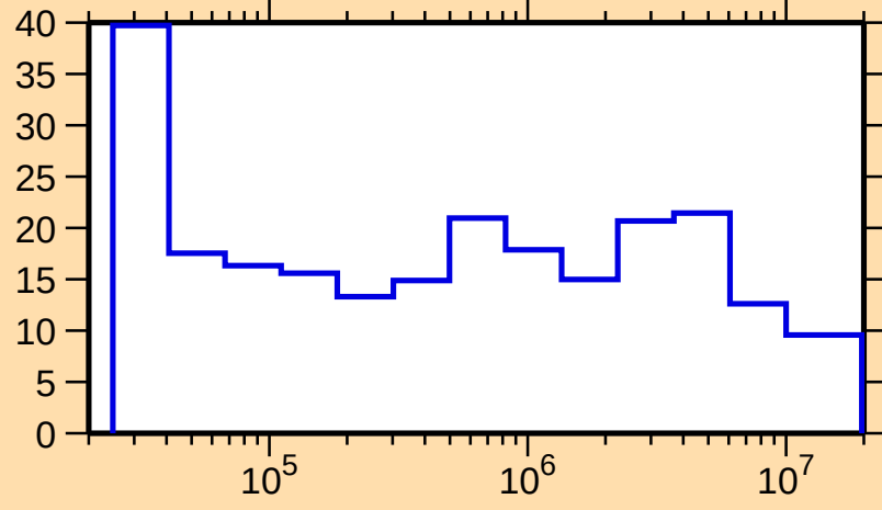
\Delta\sigma/\sigma vs. E for ^{231}\text{U}(\text{n,tot.})
