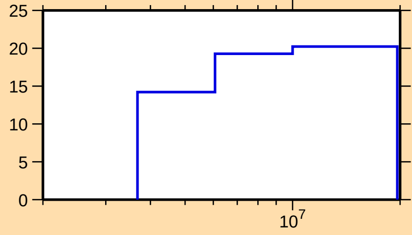
\Delta\sigma/\sigma vs. E for ^{231}\text{U}(n,\text{nonel.})
