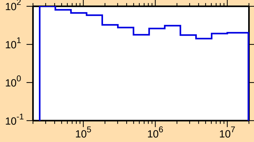
\Delta\sigma/\sigma vs. E for ^{231}\text{U}(\text{n,nonel.})
