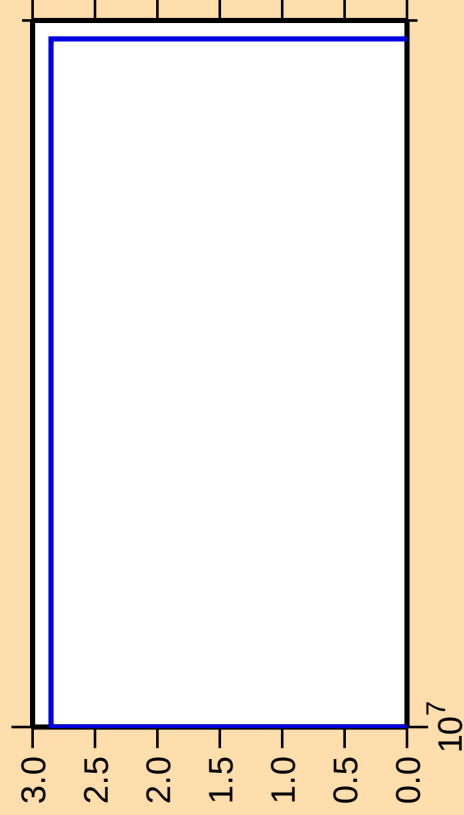
\Delta\sigma/\sigma vs. E for ^{231}\text{U}(n,p\alpha)
