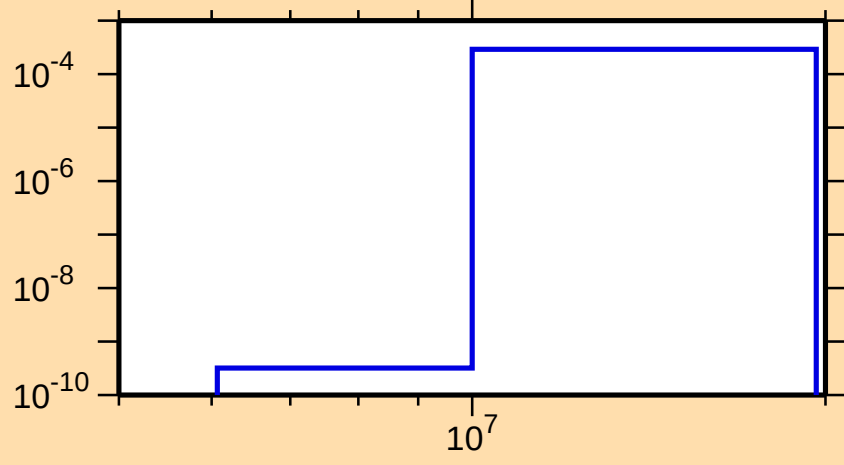
\sigma vs. E for ^{231}\text{U}(n,d)
