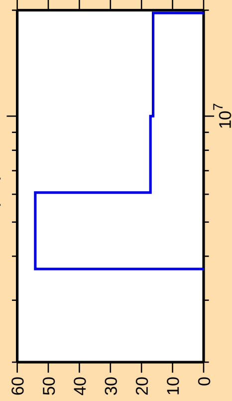
\Delta\sigma/\sigma vs. E for ^{231}\text{U}(n,f)
