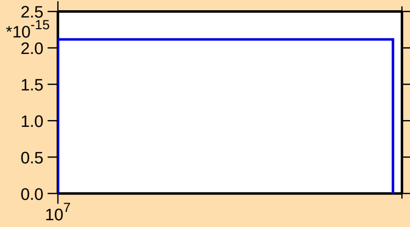
\sigma vs. E for ^{231}\text{U}(\text{mt } 34)
