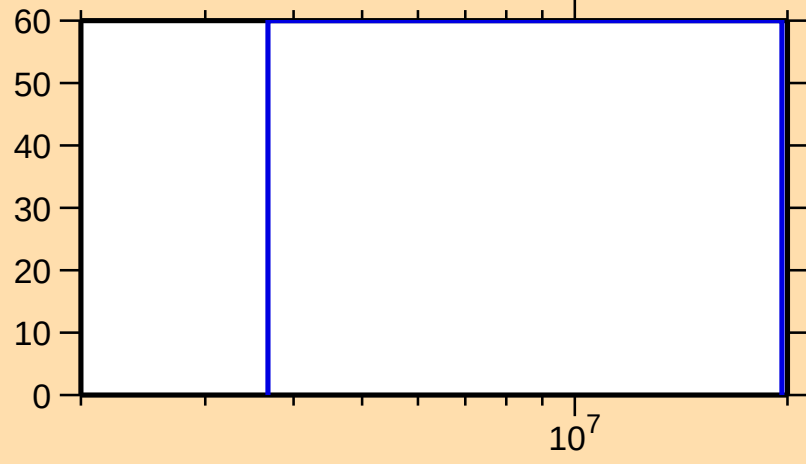
\Delta\sigma/\sigma vs. E for ^{231}\text{U}(n,2n)
