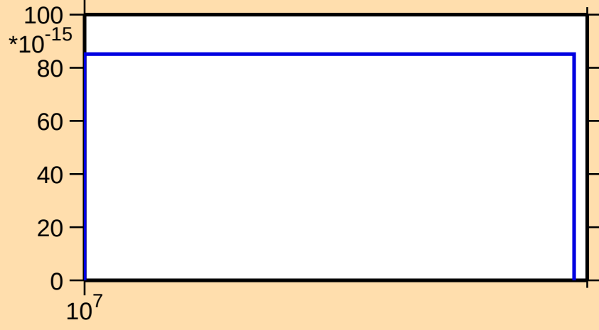
\sigma vs. E for ^{231}\text{U}(n,3n\alpha)
