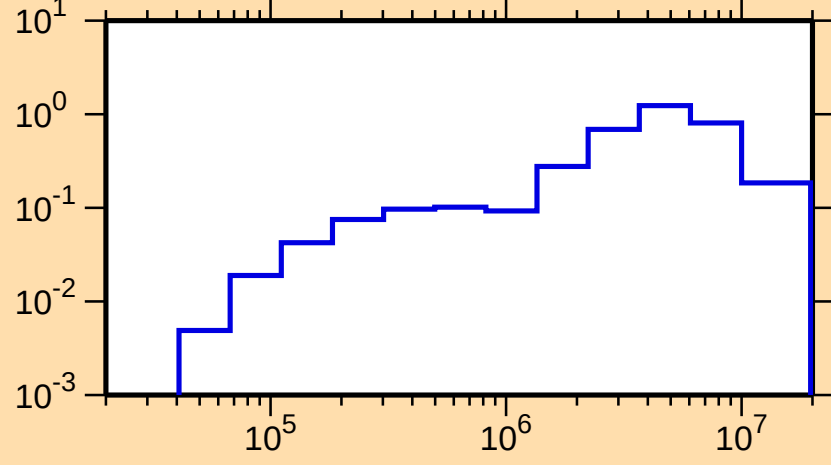
\sigma vs. E for ^{231}\text{U}(\text{n,inel.})
