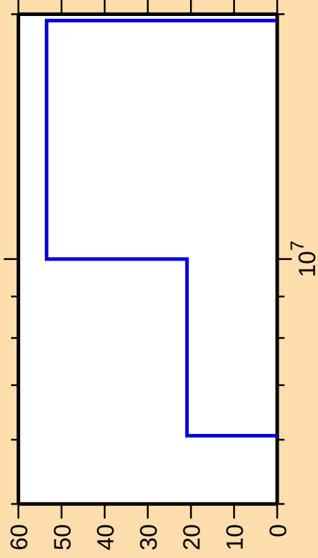
\Delta\sigma/\sigma vs. E for ^{231}\text{U}(n,t)
