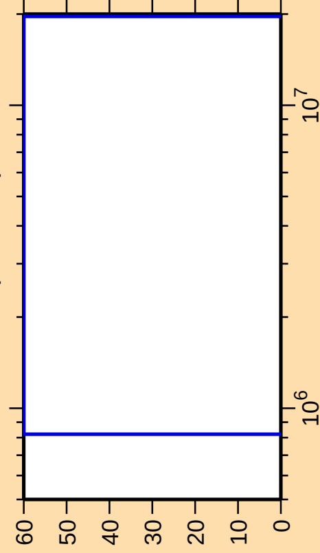
\Delta\sigma/\sigma vs. E for ^{231}\text{U}(\text{n},\text{ncont.})
