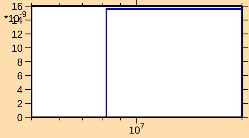
\sigma vs. E for ^{231}\text{U}(n,\text{nd})
