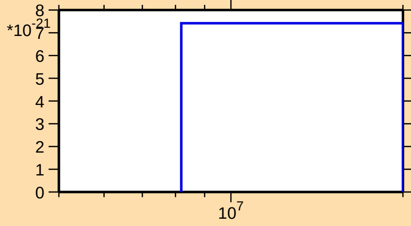
\sigma vs. E for ^{231}\text{U}(\text{mt } 42)
