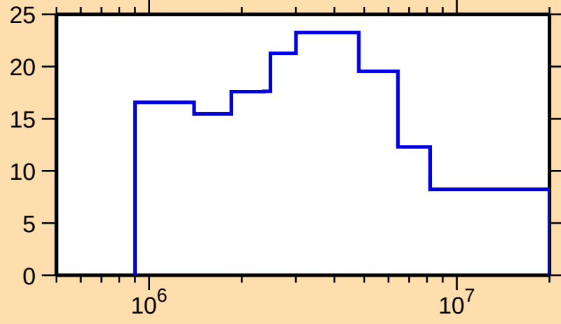
\Delta\sigma/\sigma vs. E for ^{231}\text{U}(\text{n},\text{tot.})
