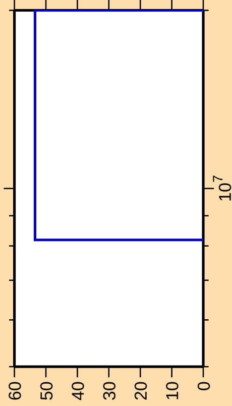
\Delta\sigma/\sigma vs. E for ^{231}\text{U}(\text{n,t})
