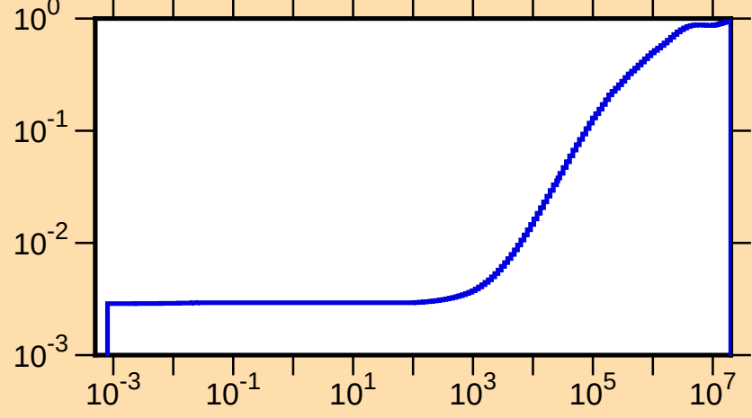
\mu vs. E for ^{234}\text{U}(\text{mt251})
