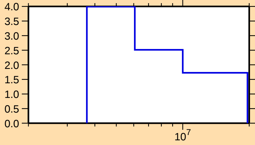
\Delta\sigma/\sigma vs. E for ^{234}\text{U}(\text{n,nonel.})
