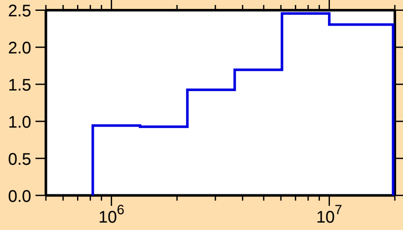
\Delta\sigma/\sigma vs. E for ^{234}\text{U}(\text{n},\text{f})
