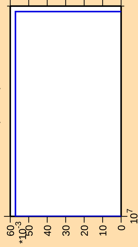
\Delta\sigma/\sigma vs. E for ^{234}\text{U}(n,3n\alpha)
