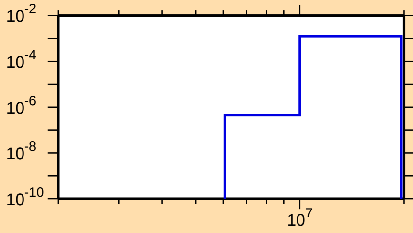
\sigma vs. E for ^{234}\text{U}(n,p)
