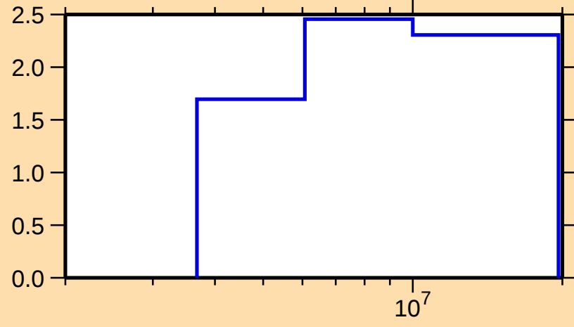
\Delta\sigma/\sigma vs. E for ^{234}\text{U}(\text{n,f})
