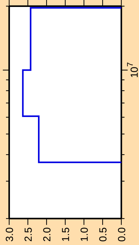
\Delta\sigma/\sigma vs. E for ^{234}\text{U}(\text{n,p})
