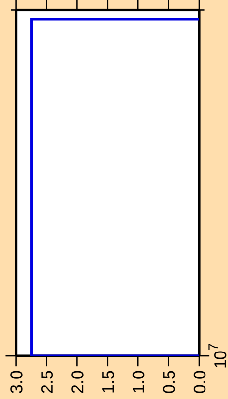
\Delta\sigma/\sigma vs. E for ^{234}\text{U}(\text{n,np})
