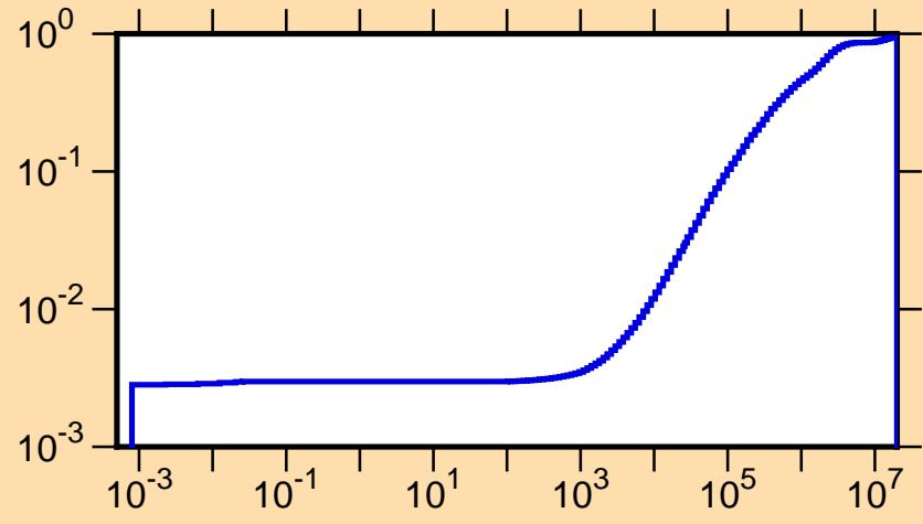
\mu vs. E for ^{239}\text{U}(\text{mt251})
