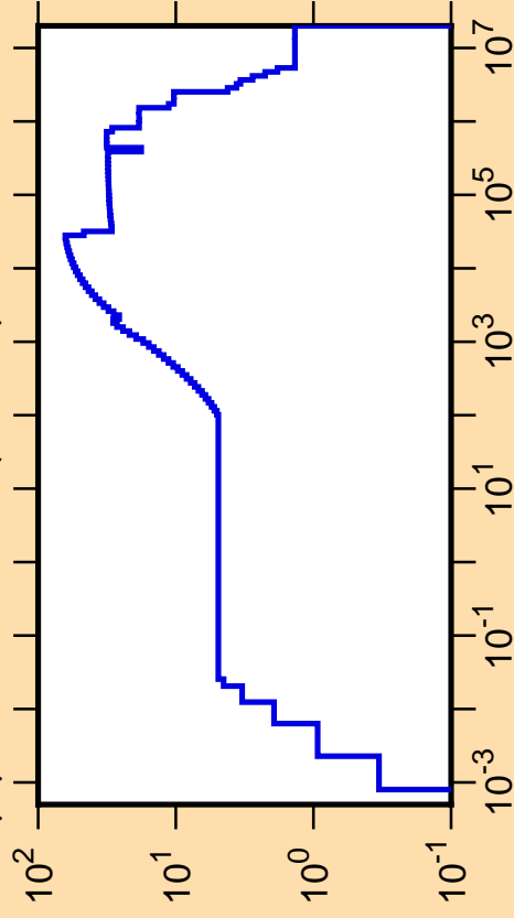
\Delta\mu/\mu vs. E for ^{239}\text{U}(\text{mt251})
