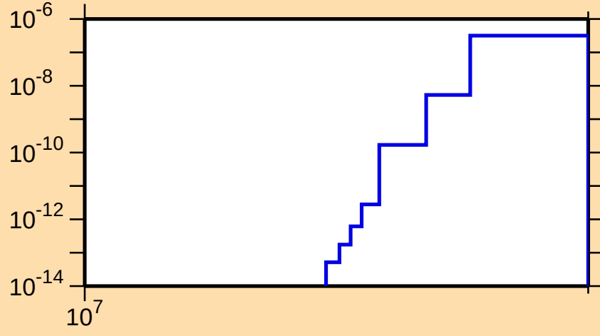
\sigma vs. E for ^{239}\text{U}(n,nt)
