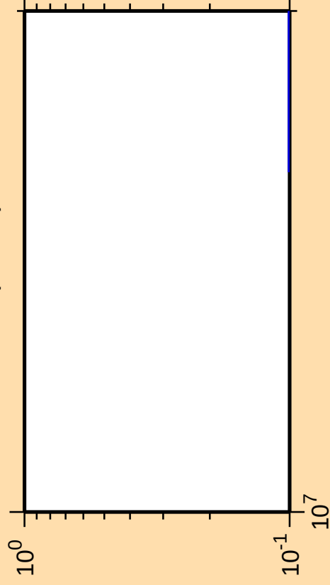
\Delta\sigma/\sigma vs. E for ^{239}\text{U} (mt 11)
