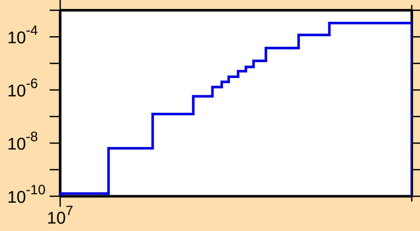
\sigma vs. E for ^{239}\text{U}(n,t)
