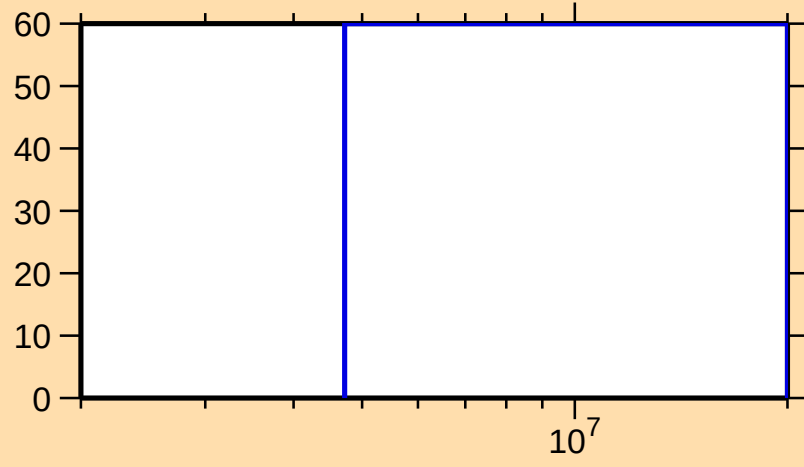
\Delta\sigma/\sigma vs. E for ^{239}\text{U}(n,ncont.)
