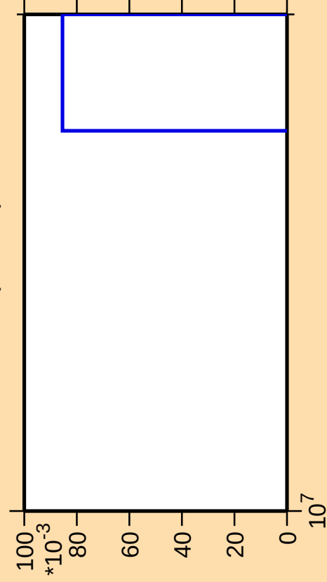
\Delta\sigma/\sigma vs. E for ^{239}\text{U}(n,\text{He3})
