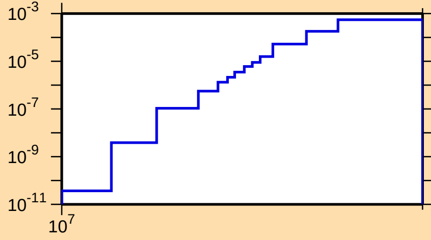
\sigma vs. E for ^{239}\text{U}(n,d)
