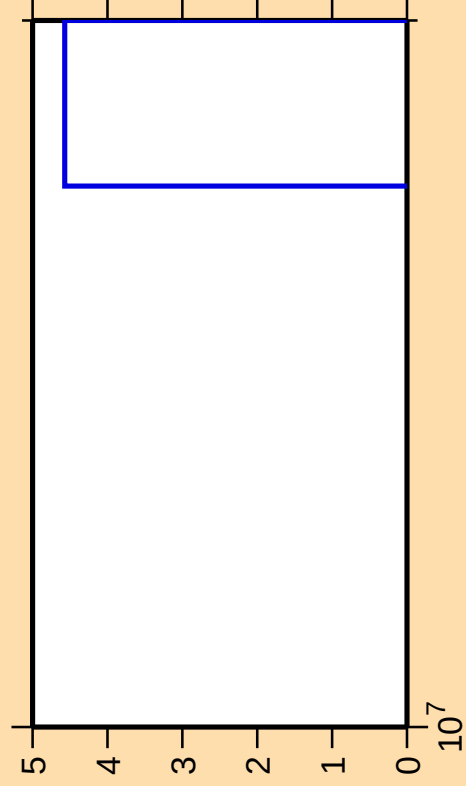
\Delta\sigma/\sigma vs. E for ^{239}\text{U}(n,3n\alpha)
