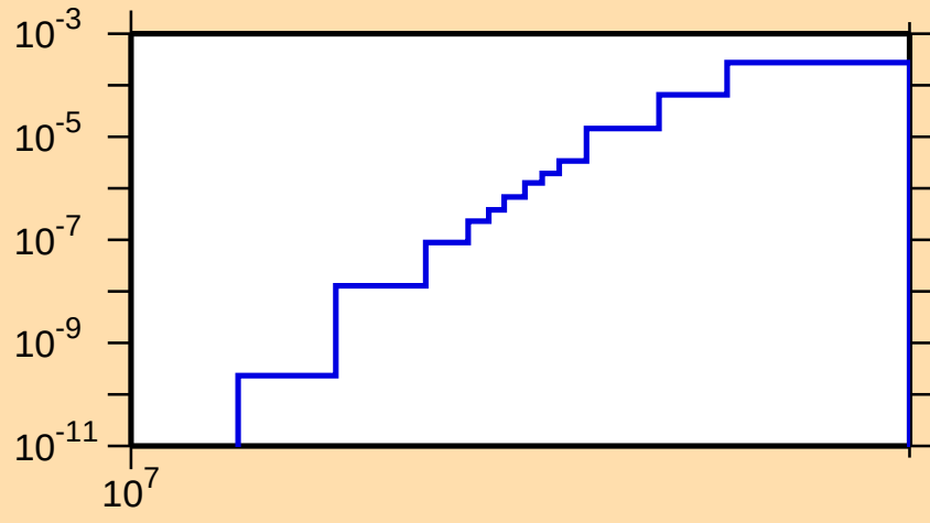
\sigma vs. E for ^{239}\text{U}(n,np)
