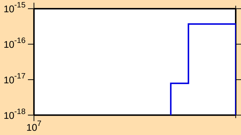
\sigma vs. E for ^{239}\text{U} (mt 11)
