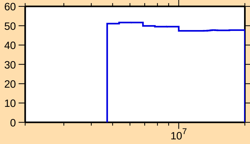
\Delta\sigma/\sigma vs. E for ^{239}\text{U}(n,el.)
