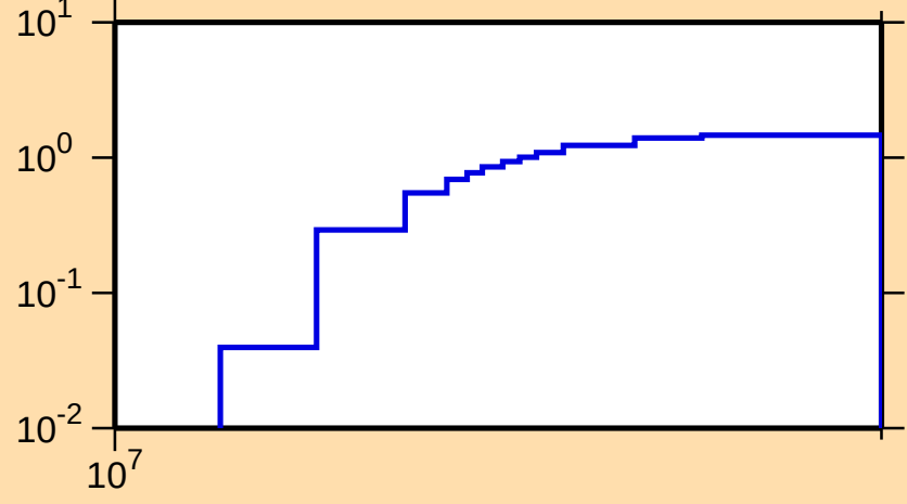
\sigma vs. E for ^{239}\text{U}(n,3n)
