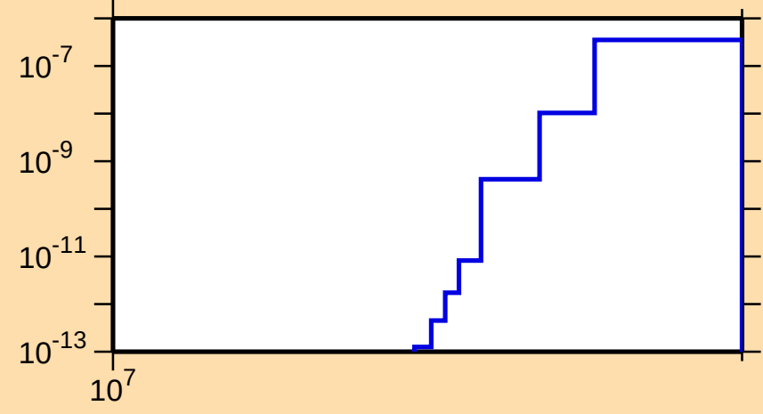
\sigma vs. E for ^{239}\text{U}(n,\text{nd})
