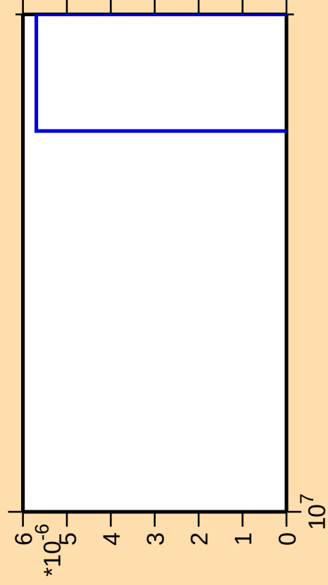
\Delta\sigma/\sigma vs. E for ^{239}\text{U} (mt 42)
