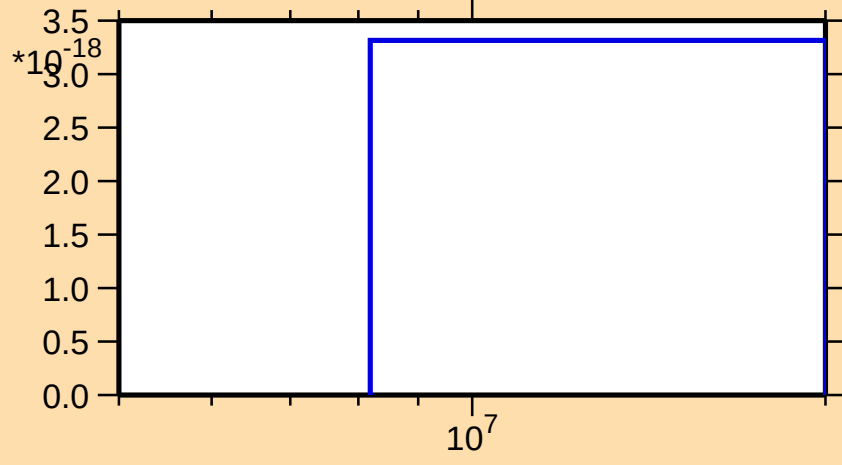
\sigma vs. E for ^{239}\text{U} (mt 11)
