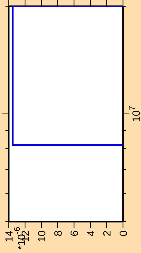
\Delta\sigma/\sigma vs. E for ^{239}\text{U} (mt 11)
