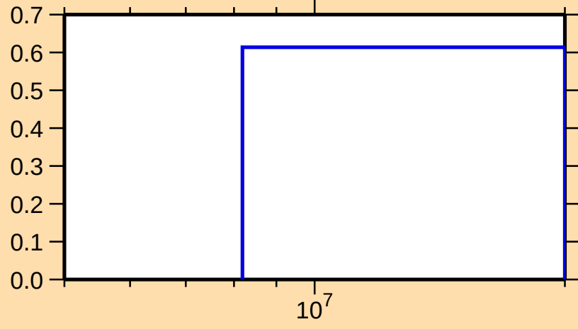
\sigma vs. E for ^{239}\text{U}(n,3n)
