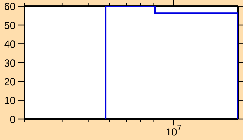
\Delta\sigma/\sigma vs. E for ^{239}\text{U}(n,p)
