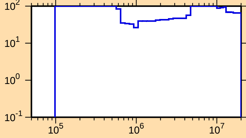
\Delta\sigma/\sigma vs. E for ^{241}\text{U}(\text{n},\text{inel.})
