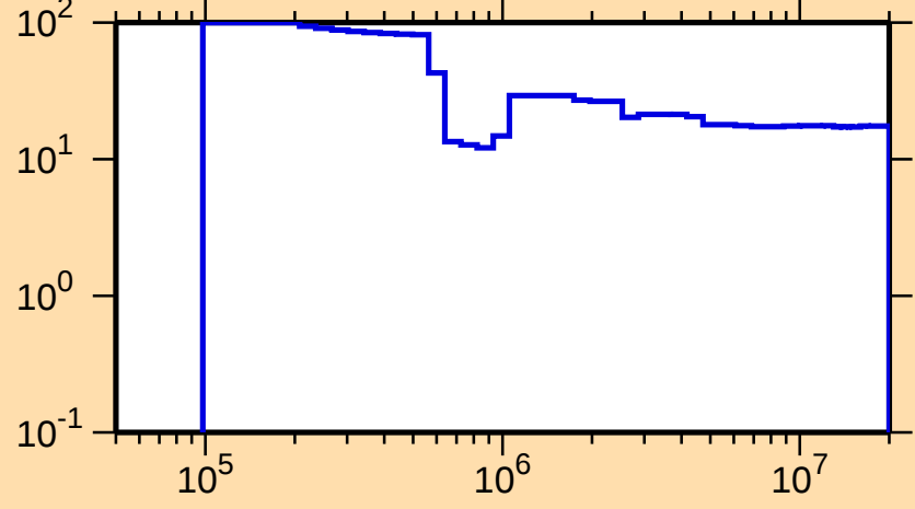
\Delta\sigma/\sigma vs. E for ^{241}\text{U}(\text{n,nonel.})
