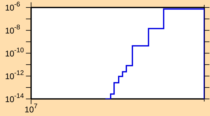
\sigma vs. E for ^{241}\text{U}(n,nt)
