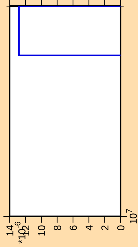
\Delta\sigma/\sigma vs. E for ^{241}\text{U} (mt 42)
