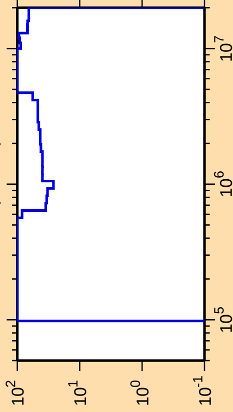
\Delta\sigma/\sigma vs. E for ^{241}\text{U}(\text{n,inel.})
