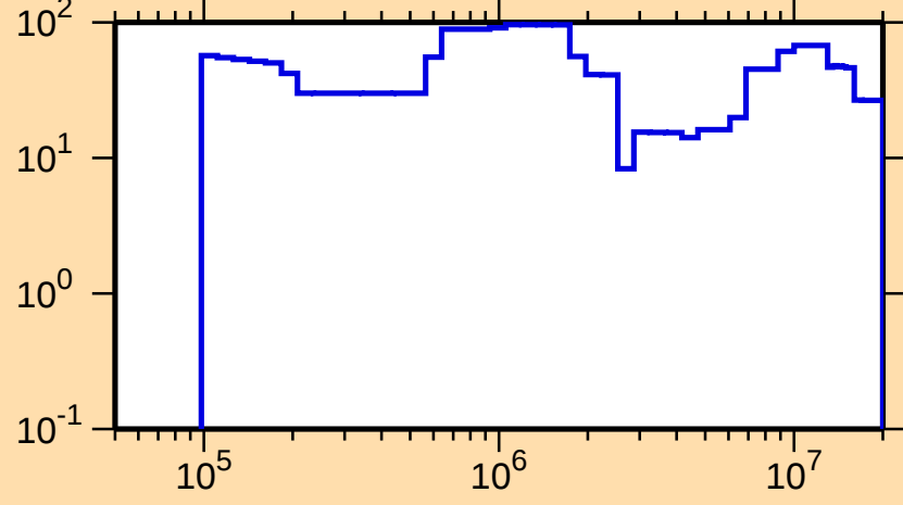
\Delta\sigma/\sigma vs. E for ^{241}\text{U}(\text{n,el.})
