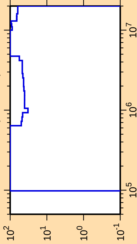
\Delta\sigma/\sigma vs. E for ^{241}\text{U}(\text{n},\text{ncont.})
