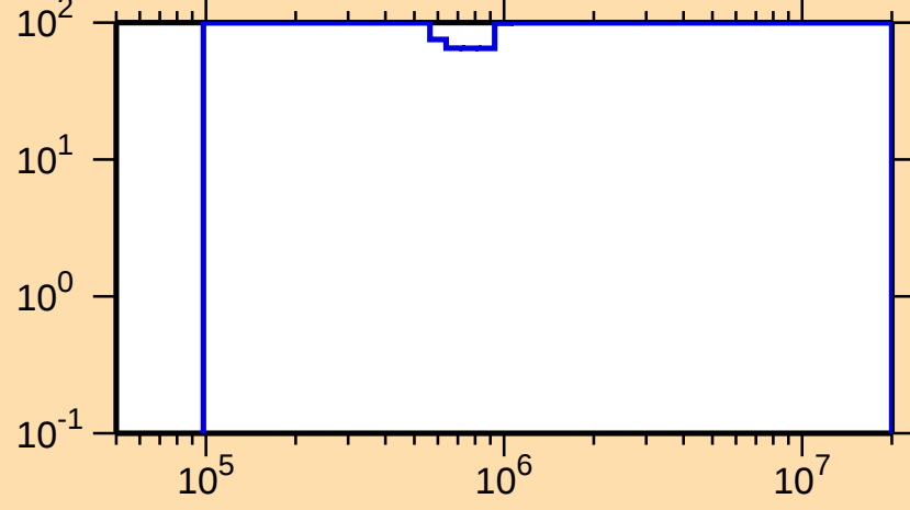
\Delta\sigma/\sigma vs. E for ^{241}\text{U}(n,\text{f})
