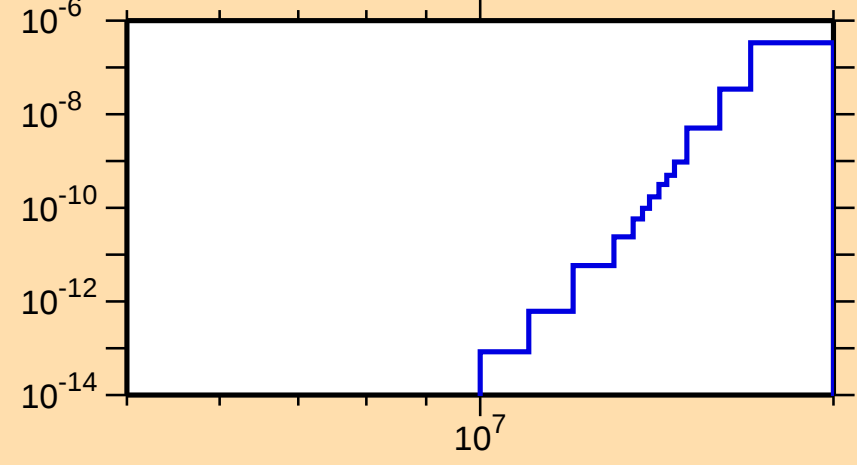
\sigma vs. E for ^{241}\text{U}(n,2n\alpha)
