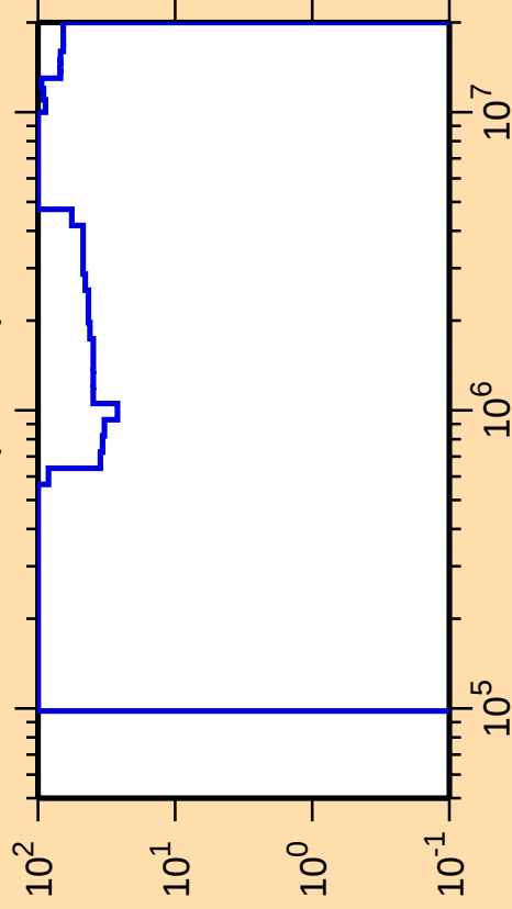
\Delta\sigma/\sigma vs. E for ^{241}\text{U}(n,\text{inel.})
