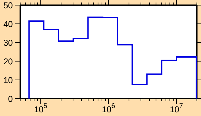
\Delta\sigma/\sigma vs. E for ^{241}\text{U}(\text{n,tot.})
