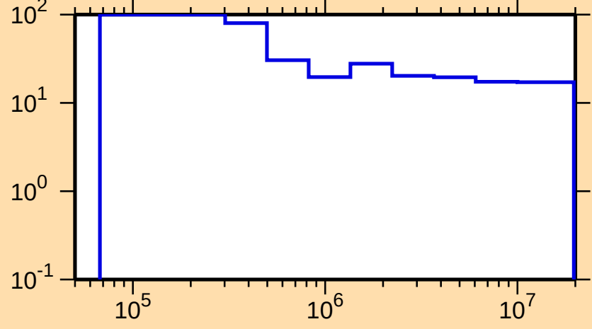
\Delta\sigma/\sigma vs. E for ^{241}\text{U}(n,\text{nonel.})
