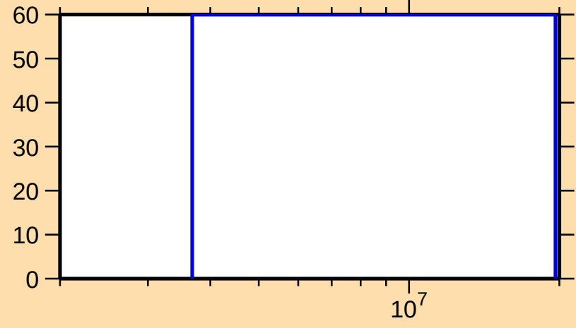
\Delta\sigma/\sigma vs. E for ^{241}\text{U}(n,n\text{cont.})
