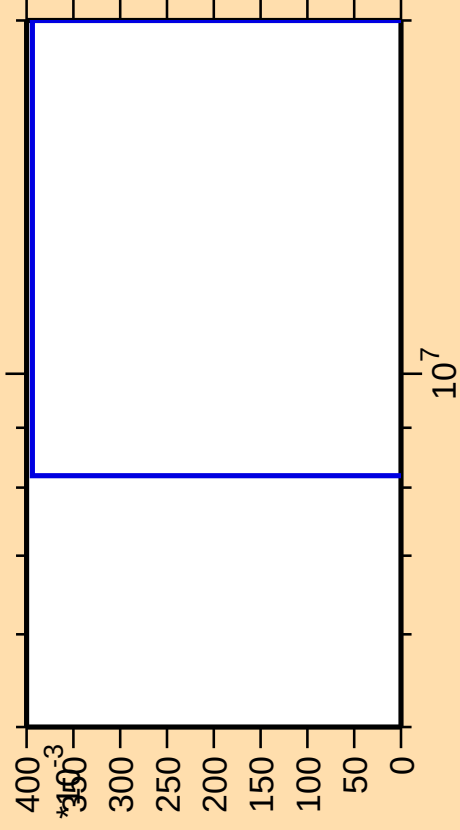
\Delta\sigma/\sigma vs. E for ^{241}\text{U}(n,3n\alpha)
