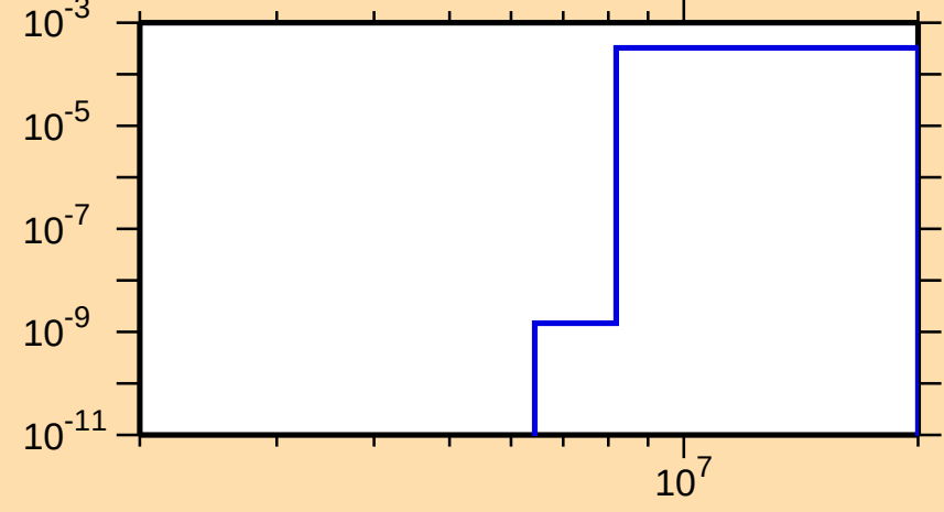
\sigma vs. E for ^{241}\text{U}(n,p)
