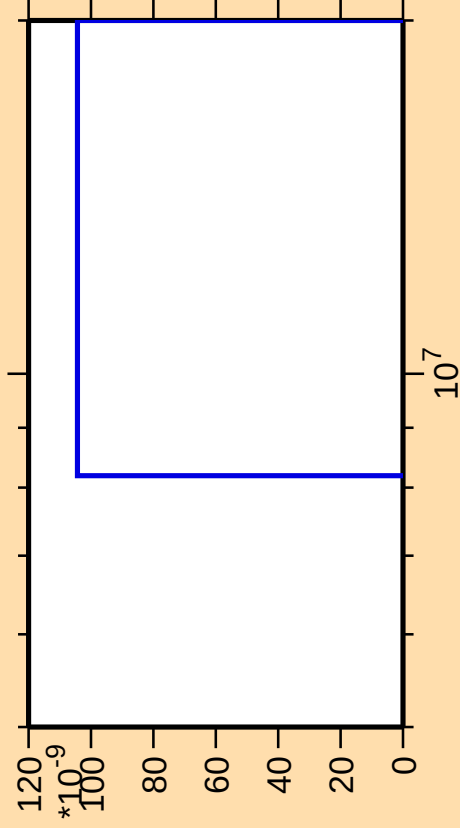
\Delta\sigma/\sigma vs. E for ^{241}\text{U}(\text{mt } 42)
