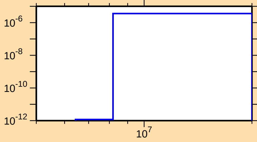
\sigma vs. E for ^{241}\text{U}(n,n\alpha)
