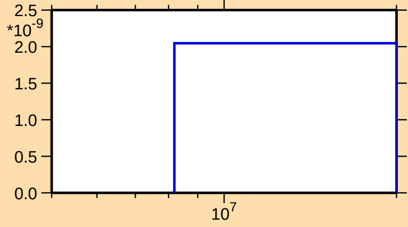
\sigma vs. E for ^{241}\text{U}(n,\text{nd})
