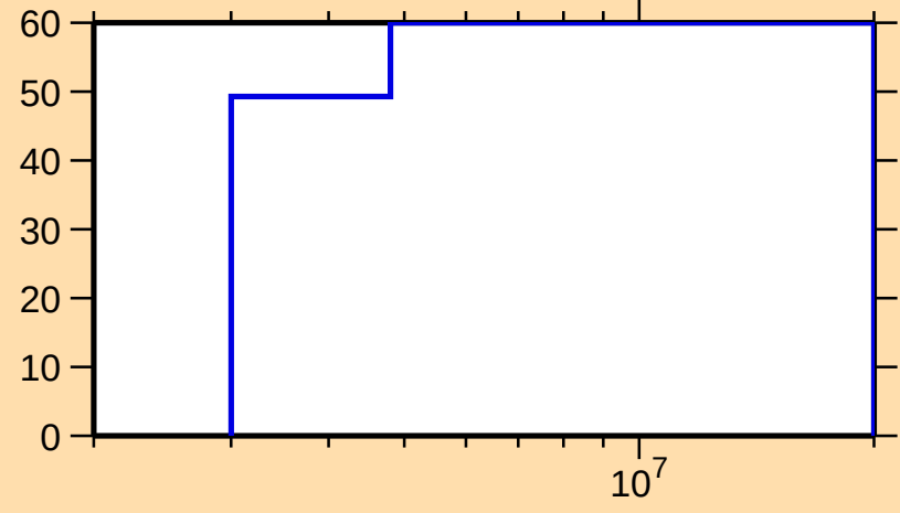
\Delta\sigma/\sigma vs. E for ^{241}\text{U}(n,\text{inel.})
