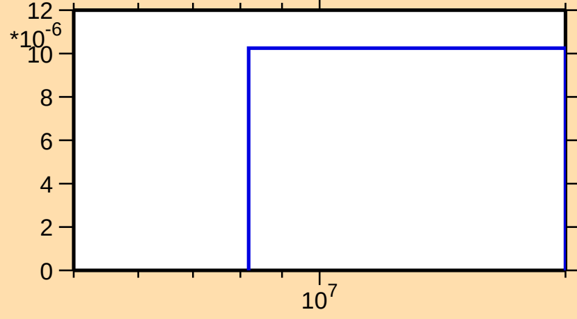
\sigma vs. E for ^{241}\text{U}(n,t)
