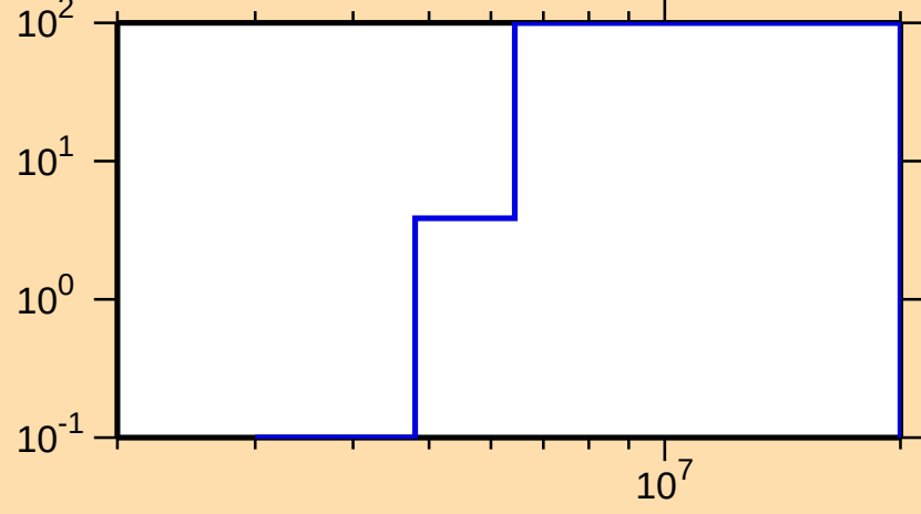
\Delta\sigma/\sigma vs. E for ^{241}\text{U}(n,p)
