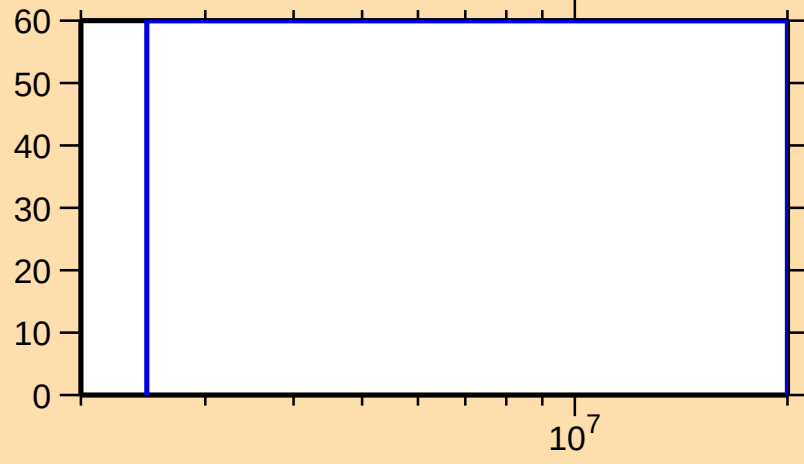
\Delta\sigma/\sigma vs. E for ^{241}\text{U}(n,\gamma)
