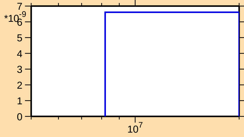
\sigma vs. E for ^{241}\text{U}(n,nt)
