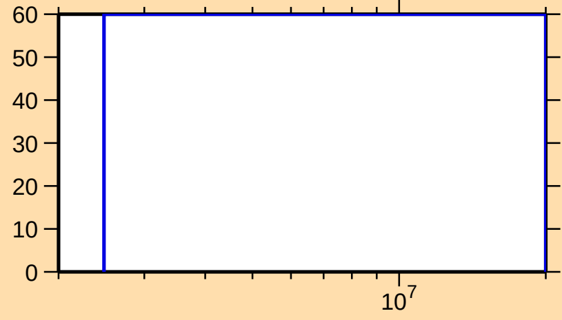
\Delta\sigma/\sigma vs. E for ^{241}\text{U}(n,n_1)
