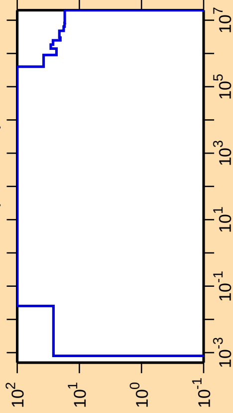
\Delta\sigma/\sigma vs. E for ^{241}\text{U}(n,\text{nonel.})
