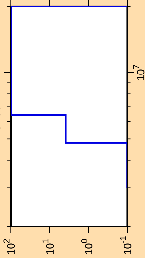
\Delta\sigma/\sigma vs. E for ^{241}\text{U}(n,p)
