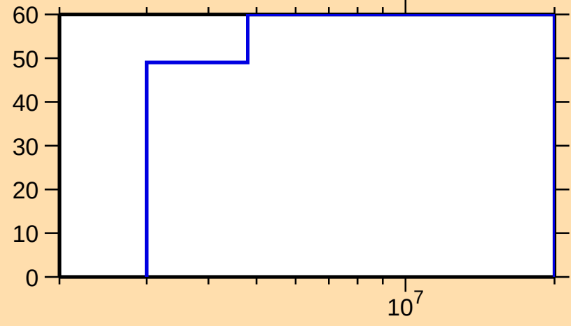
\Delta\sigma/\sigma vs. E for ^{241}\text{U}(n,ncont.)
