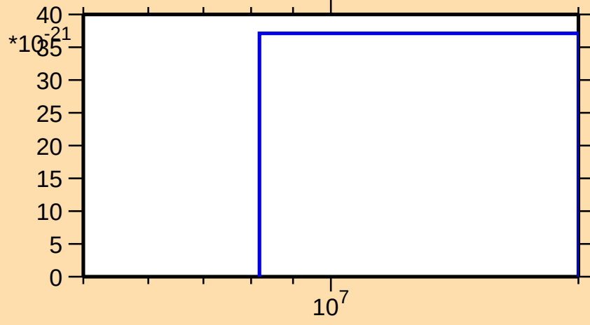
\sigma vs. E for ^{241}\text{U}(\text{mt } 42)
