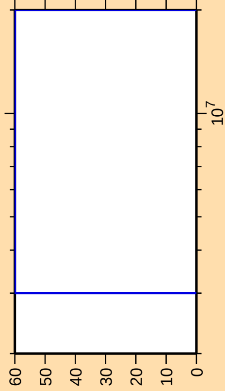
\Delta\sigma/\sigma vs. E for ^{241}\text{U}(n,n_1)
