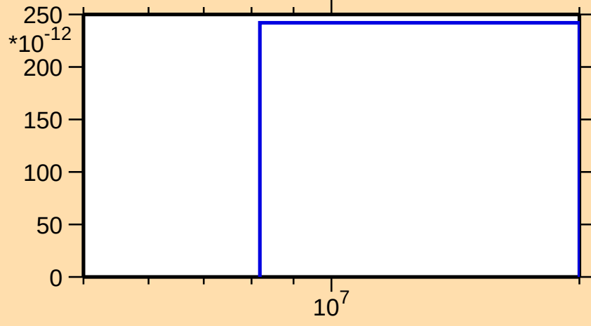
\sigma vs. E for ^{241}\text{U}(n,2np)
