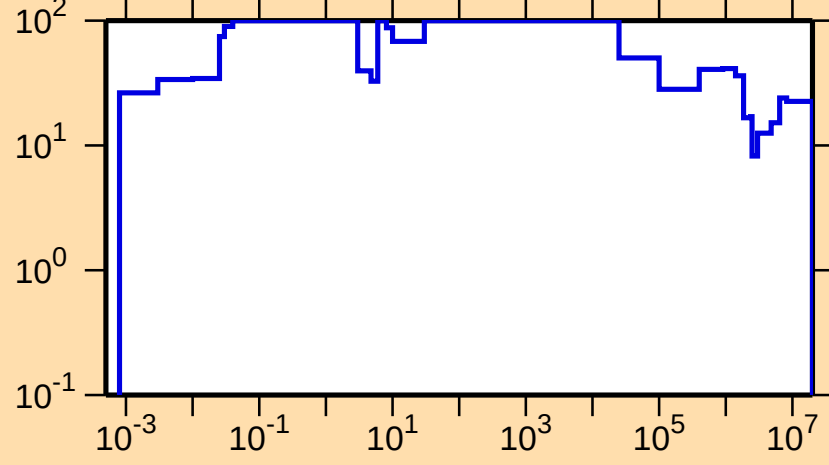
\Delta\sigma/\sigma vs. E for ^{241}\text{U}(n,\text{tot.})
