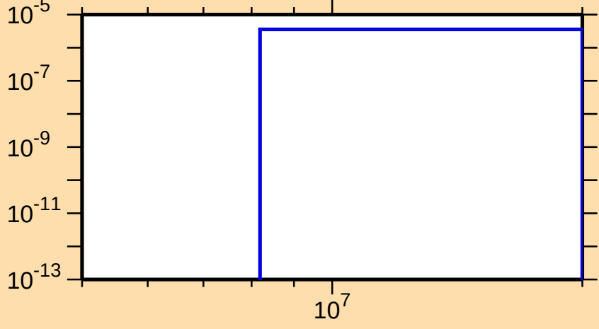
\sigma vs. E for ^{241}\text{U}(n,np)
