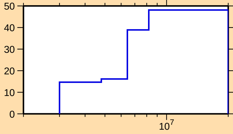
\Delta\sigma/\sigma vs. E for ^{241}\text{U}(n,\text{el.})
