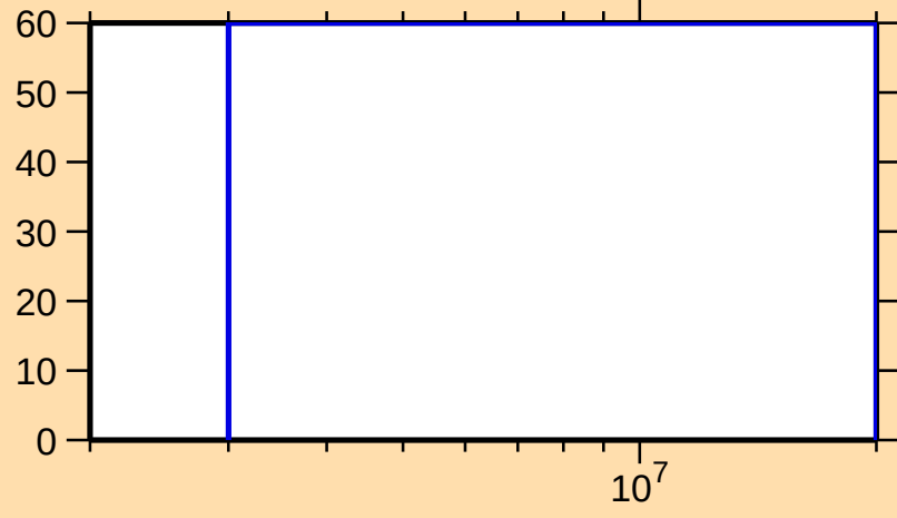
\Delta\sigma/\sigma vs. E for ^{241}\text{U}(n,2n)
