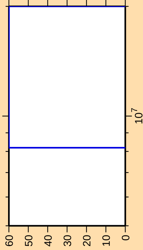
\Delta\sigma/\sigma vs. E for ^{241}\text{U}(n,3n)
