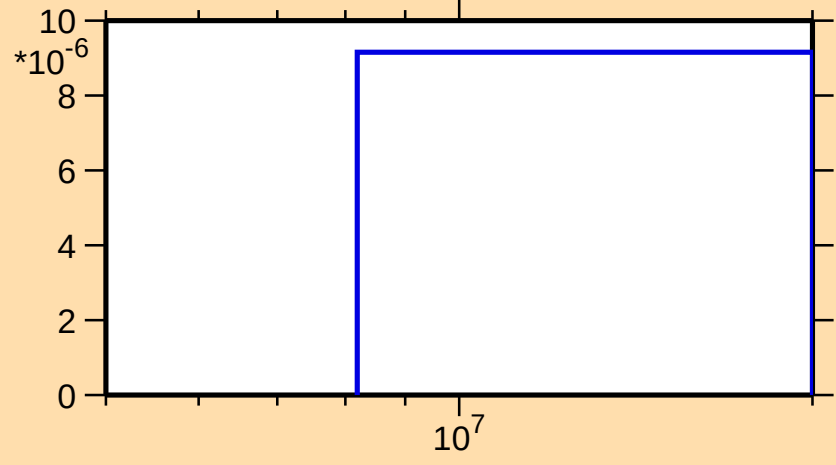
\sigma vs. E for ^{241}\text{U}(n,d)
