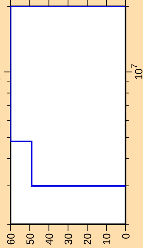
\Delta\sigma/\sigma vs. E for ^{241}\text{U}(n,\text{ncont.})
