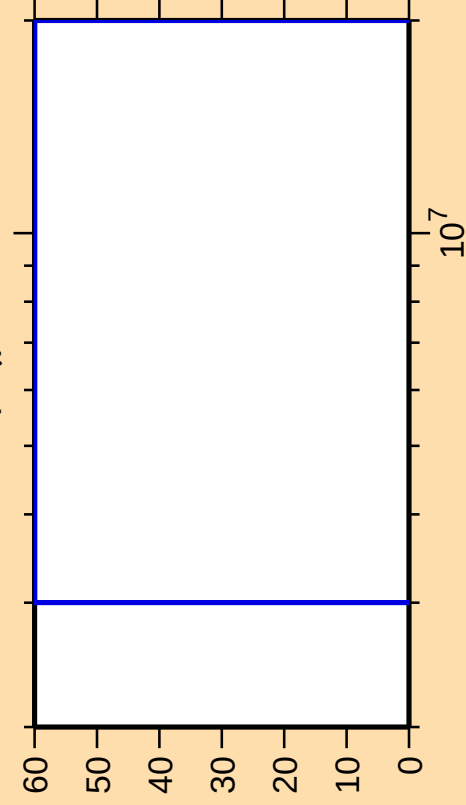
\Delta\sigma/\sigma vs. E for ^{241}\text{U}(n,\gamma)
