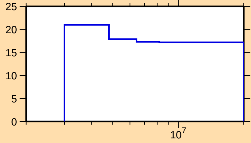
\Delta\sigma/\sigma vs. E for ^{241}\text{U}(n,\text{nonel.})
