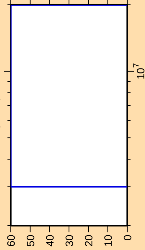
\Delta\sigma/\sigma vs. E for ^{241}\text{U}(n,2n)
