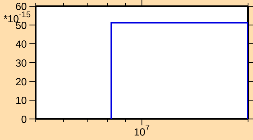
\sigma vs. E for ^{241}\text{U}(n,3n\alpha)
