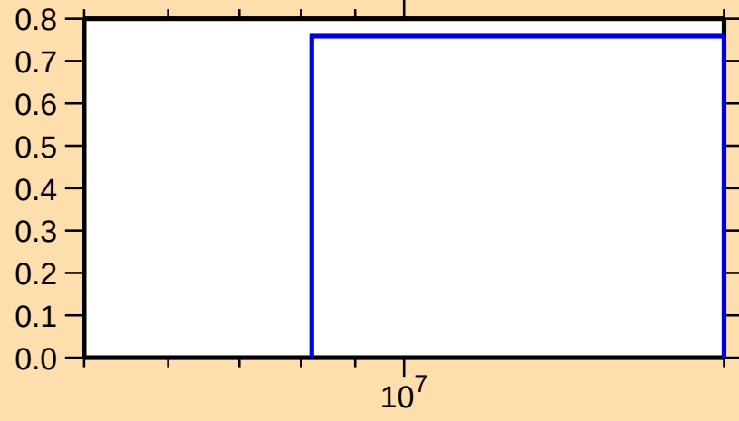
\sigma vs. E for ^{241}\text{U}(n,3n)
