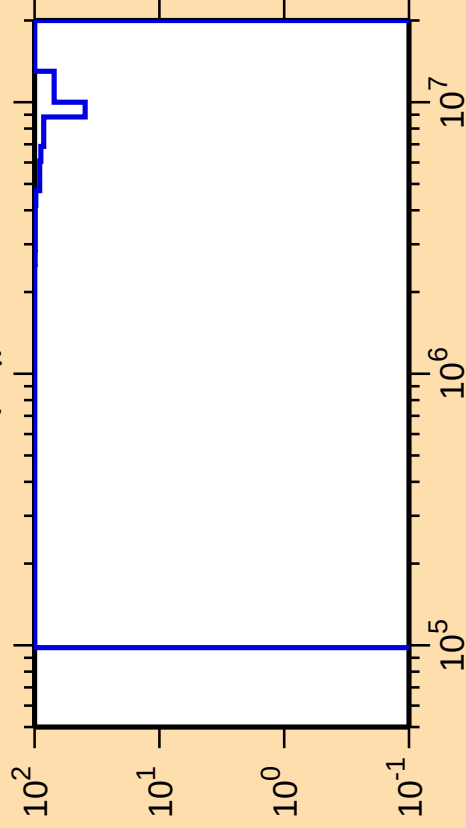
\Delta\sigma/\sigma vs. E for ^{243}\text{U}(n,\gamma)
