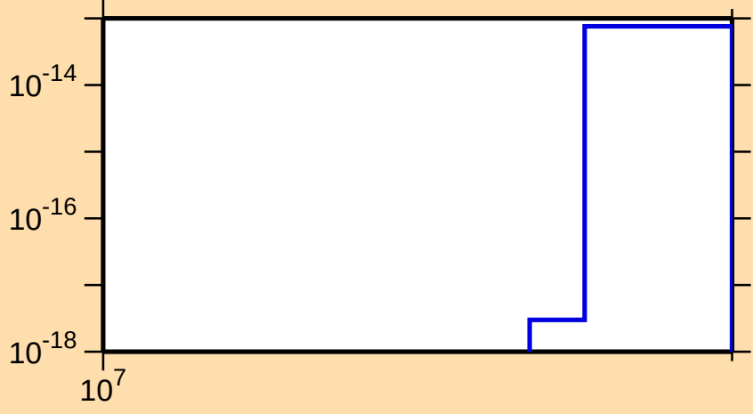
\sigma vs. E for ^{243}\text{U}(n,\text{He3})
