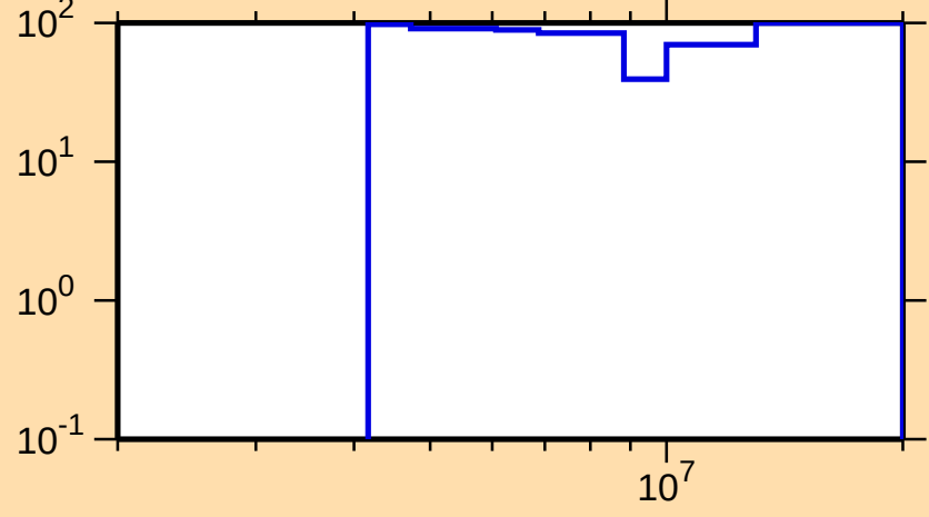
\Delta\sigma/\sigma vs. E for ^{243}\text{U}(n,\gamma)
