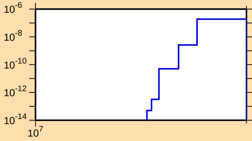
\sigma vs. E for ^{243}\text{U}(n,2np)
