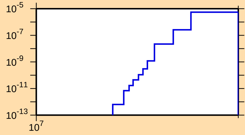
\sigma vs. E for ^{243}\text{U}(n,nt)
