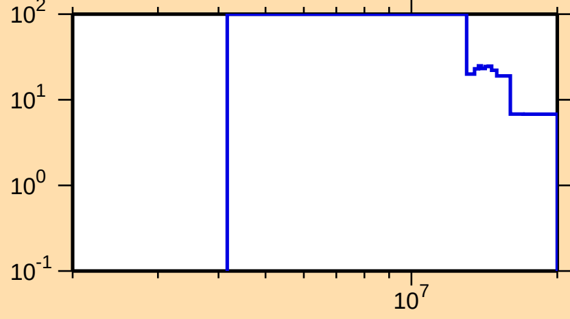
\Delta\sigma/\sigma vs. E for ^{243}\text{U}(n,ncont.)
