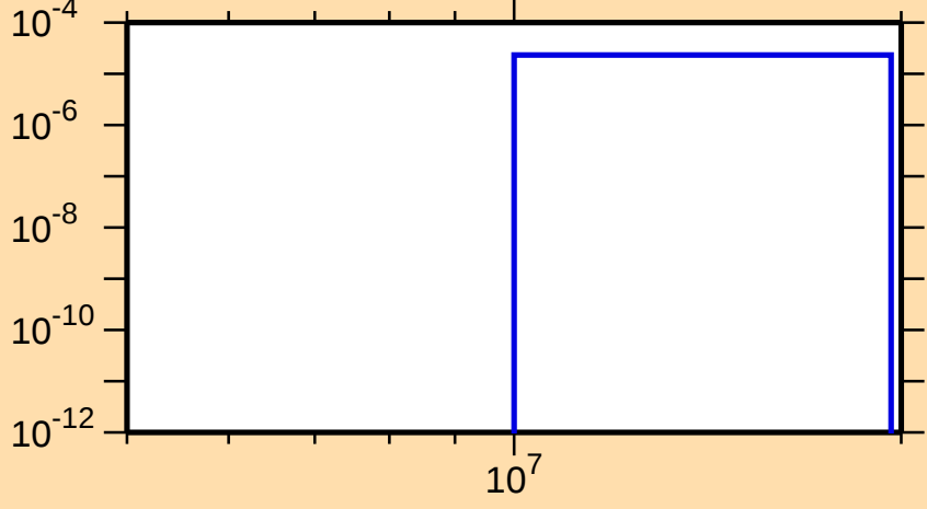
\sigma vs. E for ^{243}\text{U}(n,d)
