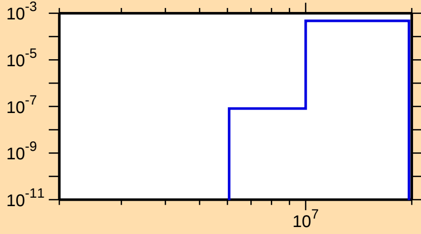
\sigma vs. E for ^{243}\text{U}(n,p)
