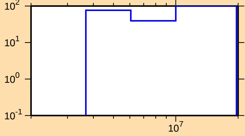
\Delta\sigma/\sigma vs. E for ^{243}\text{U}(n,2n)
