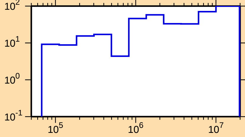
\Delta\sigma/\sigma vs. E for ^{243}\text{U}(\text{n,el.})
