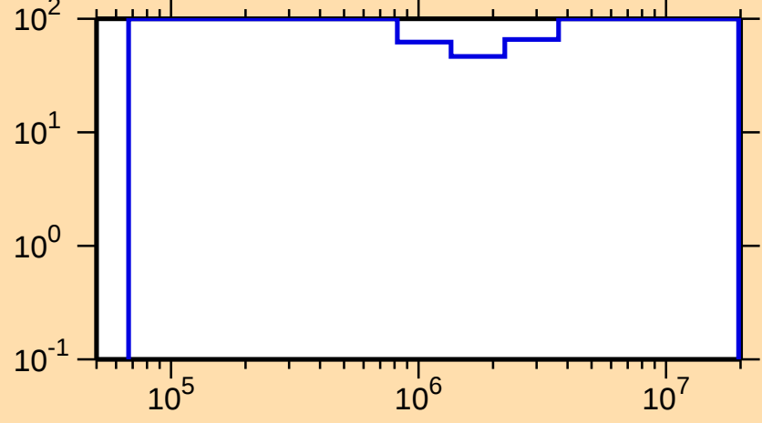
\Delta\sigma/\sigma vs. E for ^{243}\text{U}(n,n\text{cont.})
