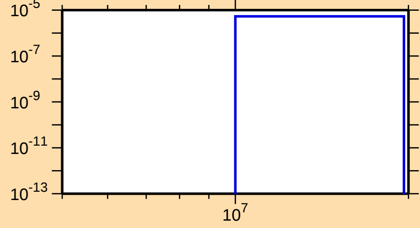
\sigma vs. E for ^{243}\text{U}(n,np)
