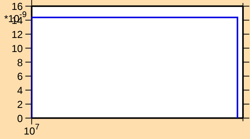
\sigma vs. E for ^{243}\text{U}(\text{n},\text{nd})
