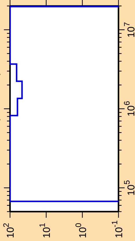
\Delta\sigma/\sigma vs. E for ^{243}\text{U}(\text{n},\text{ncont.})
