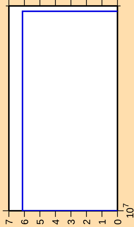
\Delta\sigma/\sigma vs. E for ^{243}\text{U}(\text{n},\text{nt})
