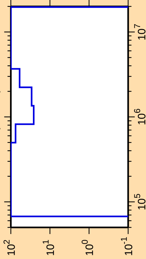
\Delta\sigma/\sigma vs. E for ^{243}\text{U}(\text{n,inel.})
