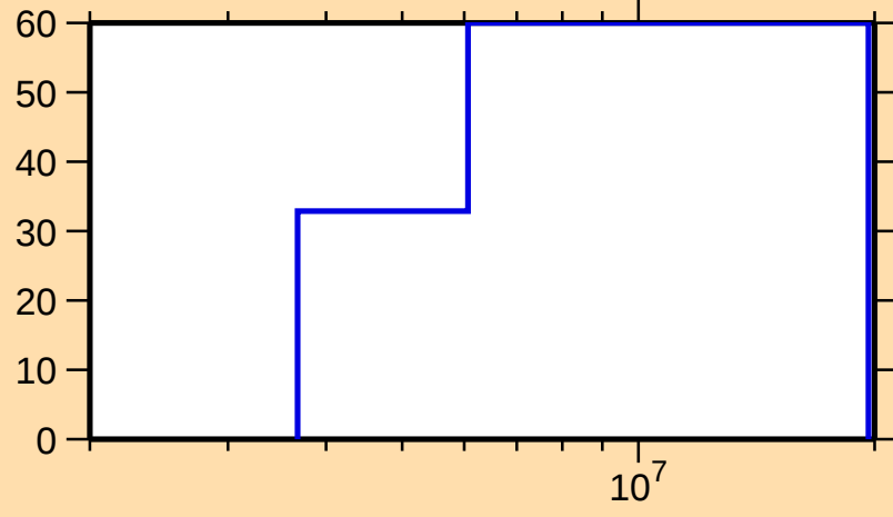
\Delta\sigma/\sigma vs. E for ^{243}\text{U}(\text{n,el.})
