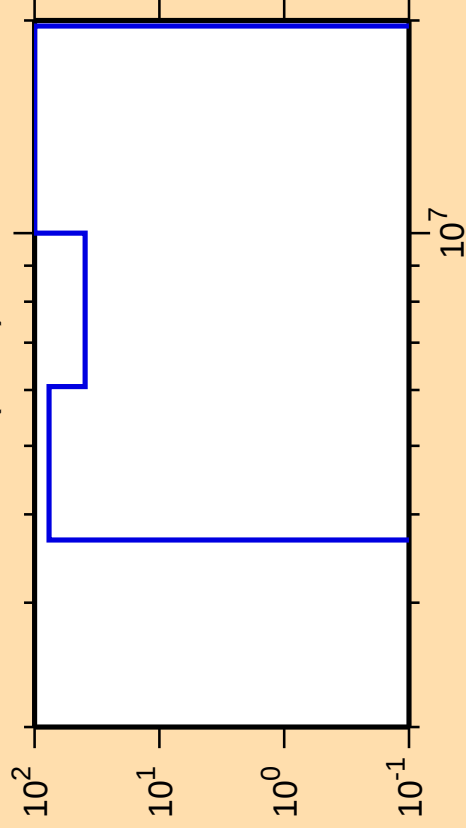
\Delta\sigma/\sigma vs. E for ^{243}\text{U}(n,2n)
