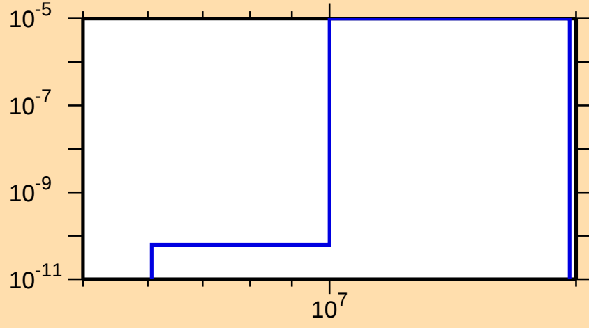
\sigma vs. E for ^{243}\text{U}(n,\alpha)
