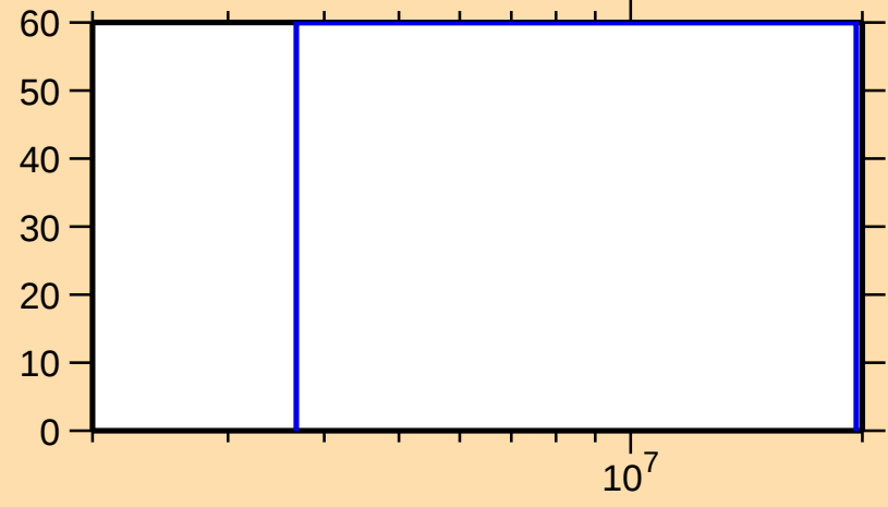
\Delta\sigma/\sigma vs. E for ^{243}\text{U}(n,ncont.)
