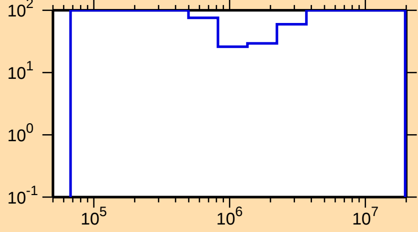
\Delta\sigma/\sigma vs. E for ^{243}\text{U}(n,\text{inel.})
