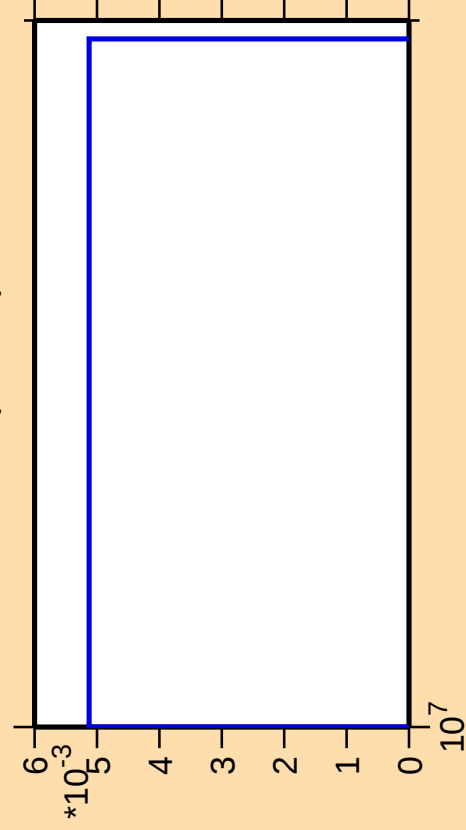
\Delta\sigma/\sigma vs. E for ^{243}\text{U}(n,\text{He3})
