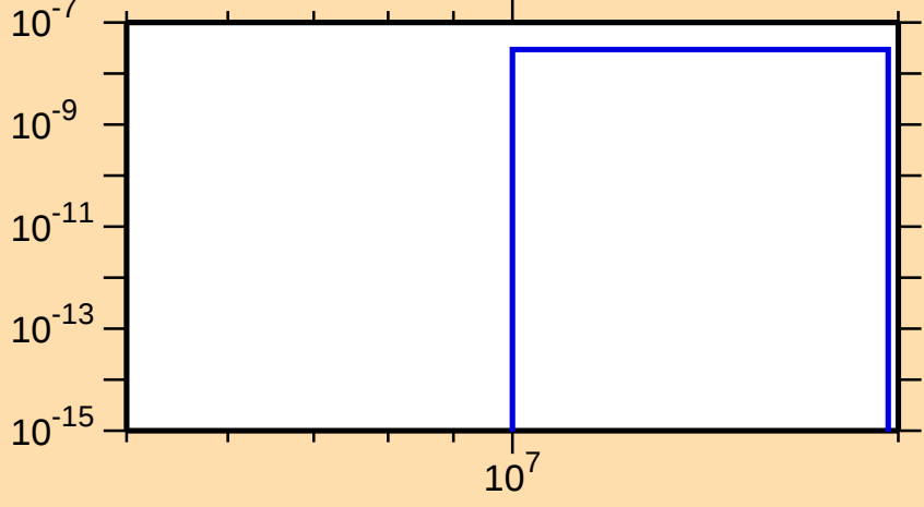
\sigma vs. E for ^{243}\text{U}(n,2n\alpha)
