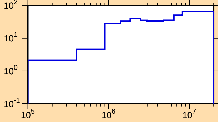
\Delta\sigma/\sigma vs. E for ^{243}\text{U}(\text{n},\text{tot.})
