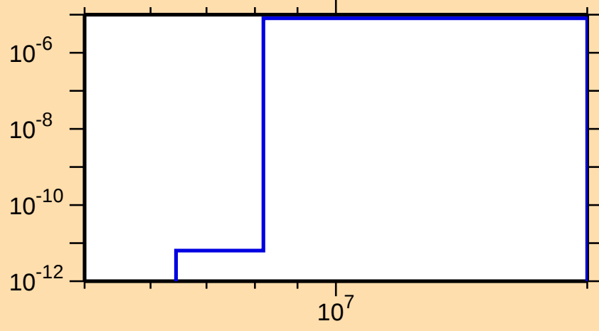
\sigma vs. E for ^{243}\text{U}(n,n\alpha)
