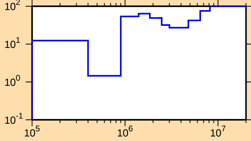
\Delta\sigma/\sigma vs. E for ^{243}\text{U}(\text{n},\text{el.})
