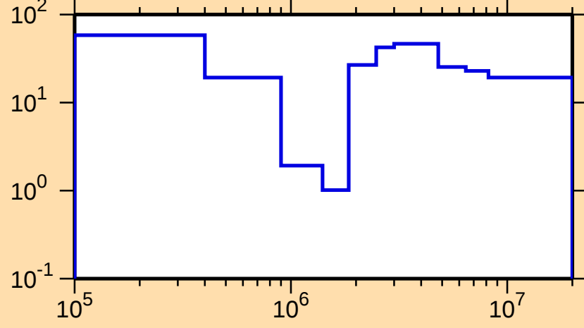
\Delta\sigma/\sigma vs. E for ^{243}\text{U}(\text{n,nonel.})
