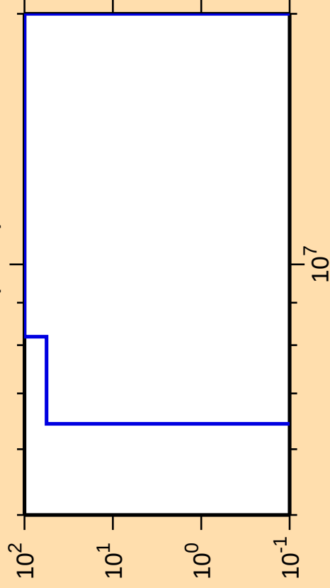
\Delta\sigma/\sigma vs. E for ^{243}\text{U}(n,n\alpha)
