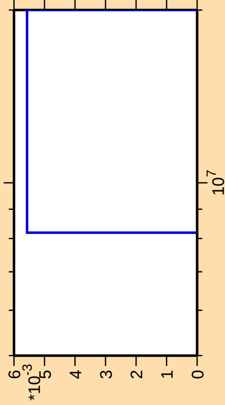
\Delta\sigma/\sigma vs. E for ^{243}\text{U}(\text{n},\text{He3})
