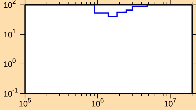
\Delta\sigma/\sigma vs. E for ^{243}\text{U}(n,n\text{cont.})
