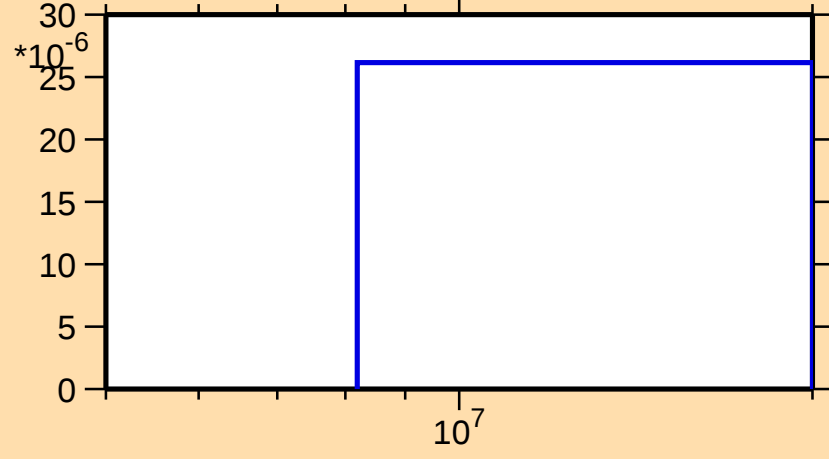
\sigma vs. E for ^{243}\text{U}(n,t)
