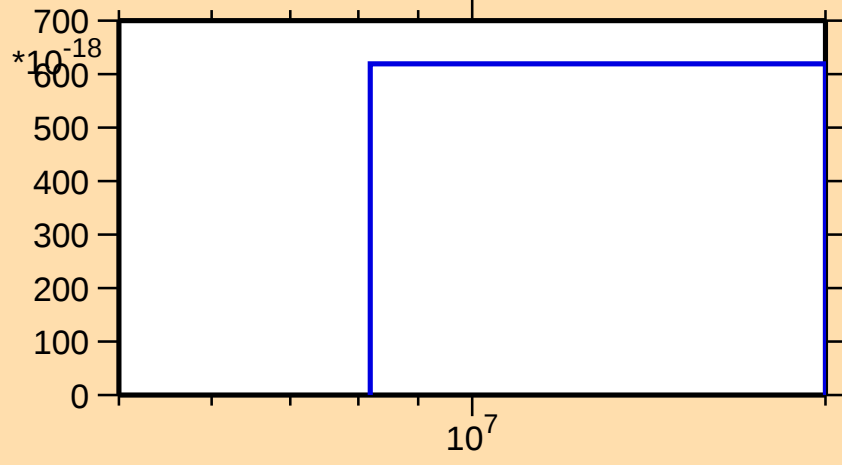
\sigma vs. E for ^{243}\text{U}(\text{n},\text{He3})
