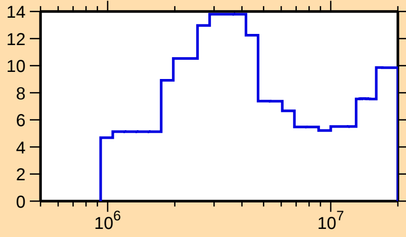
\Delta\sigma/\sigma vs. E for ^{95}\text{Ag}(n,\text{tot.})
