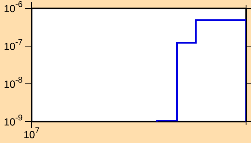
\sigma vs. E for ^{95}\text{Ag}(n,2n)
