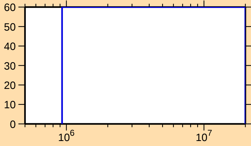
\Delta\sigma/\sigma vs. E for ^{95}\text{Ag}(n,n\text{cont.})
