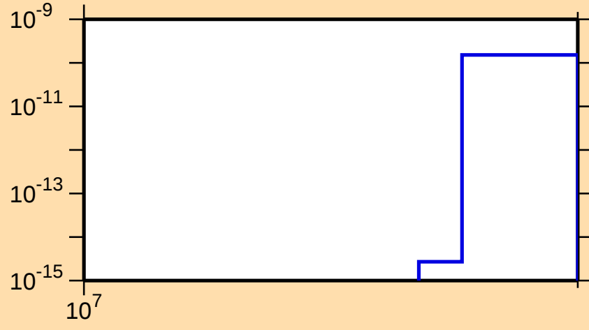
\sigma vs. E for ^{95}\text{Ag}(n,2np)
