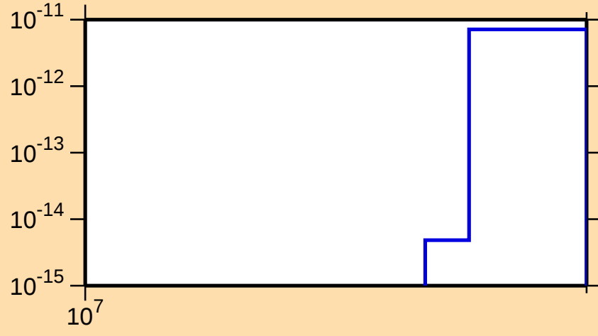
\sigma vs. E for ^{95}\text{Ag}(\text{mt } 34)
