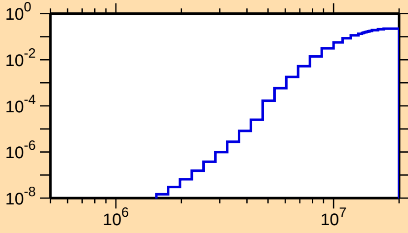
\sigma vs. E for ^{95}\text{Ag}(n,p\alpha)
