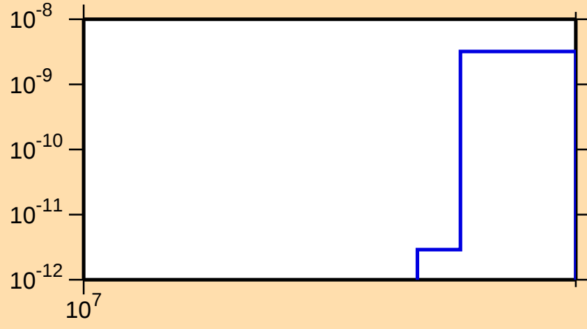
\sigma vs. E for ^{95}\text{Ag}(n,\text{nd})
