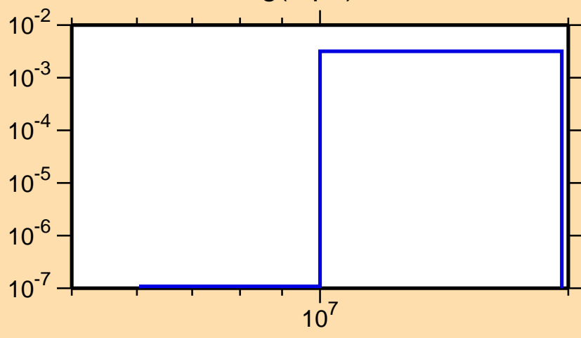
\sigma vs. E for ^{95}\text{Ag}(n,\text{pd})
