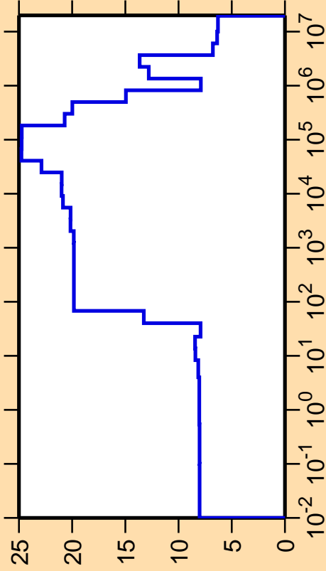
\Delta\sigma/\sigma vs. E for ^{95}\text{Ag}(n,\text{el.})
