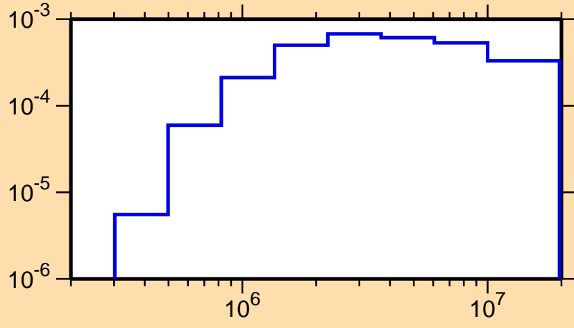
\sigma vs. E for ^{95}\text{Ag}(n,n_2)
