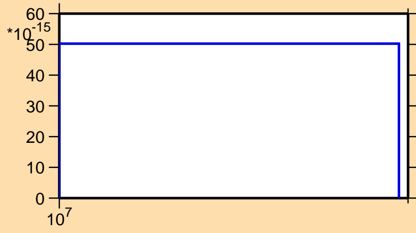
\sigma vs. E for ^{95}\text{Ag} (mt 34)
