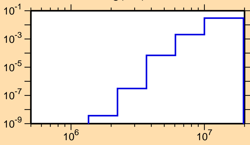
\sigma vs. E for ^{95}\text{Ag}(n,d)
