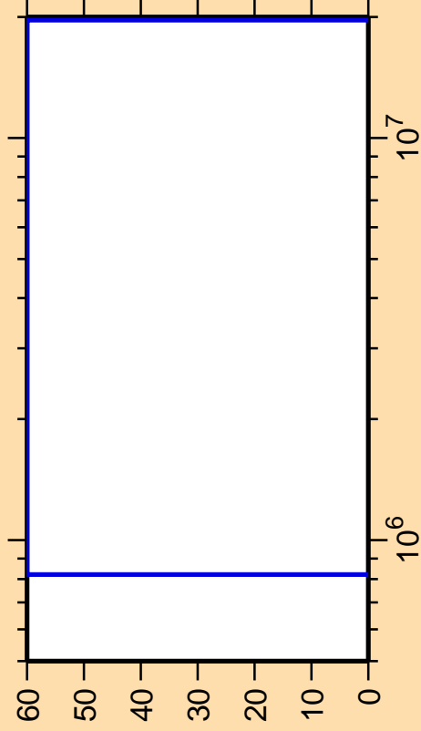
\Delta\sigma/\sigma vs. E for ^{95}\text{Ag}(n,d)
