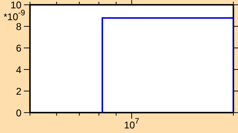
\sigma vs. E for ^{95}\text{Ag}(n,2n)
