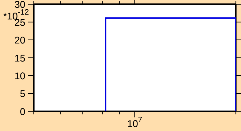
\sigma vs. E for ^{95}\text{Ag}(n,\text{nd})
