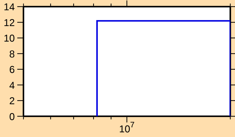
\Delta\sigma/\sigma vs. E for ^{95}\text{Ag}(n,\text{nonel.})
