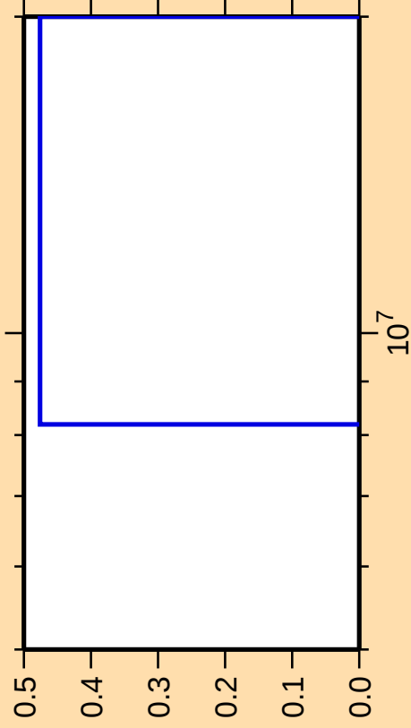
\Delta\sigma/\sigma vs. E for ^{95}\text{Ag}(\text{mt } 34)
