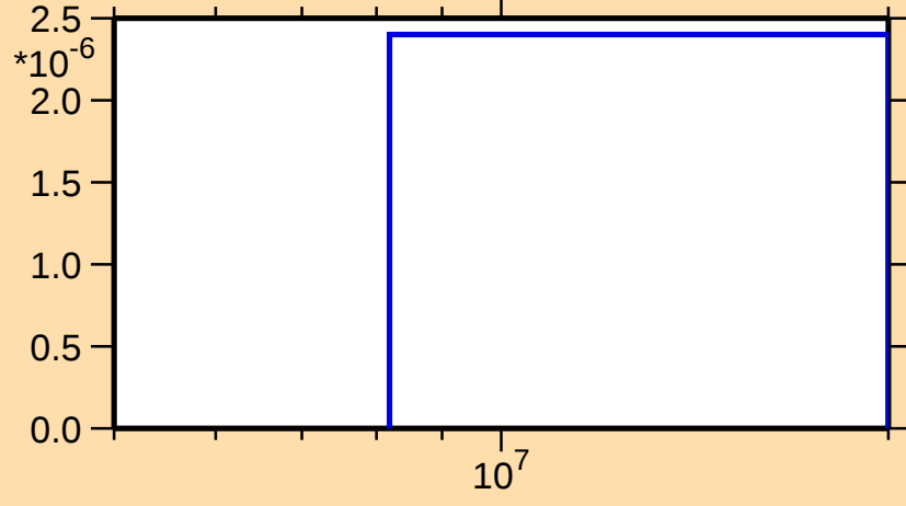
\sigma vs. E for ^{95}\text{Ag}(n,n\alpha)
