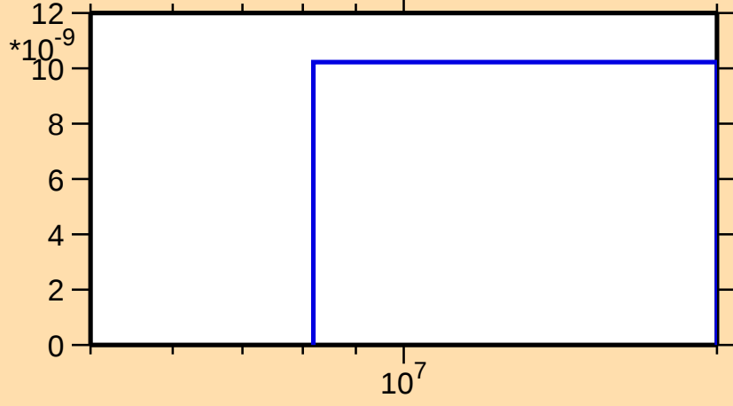
\sigma vs. E for ^{95}\text{Ag}(n,\text{pt})
