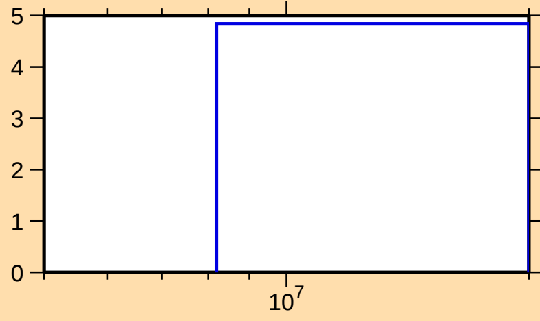
\Delta\sigma/\sigma vs. E for ^{95}\text{Ag}(n,\text{el.})
