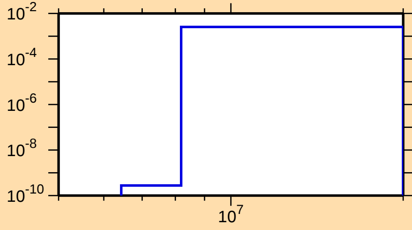
\sigma vs. E for ^{95}\text{Ag}(n,\text{pd})
