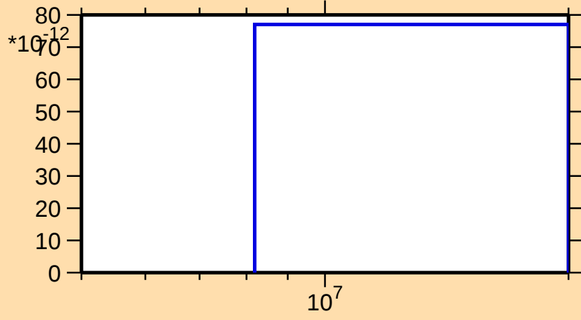
\sigma vs. E for ^{95}\text{Ag}(\text{mt117})
