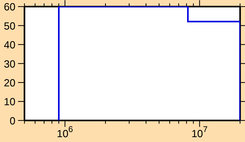
\Delta\sigma/\sigma vs. E for ^{95}\text{Ag}(n,n_1)
