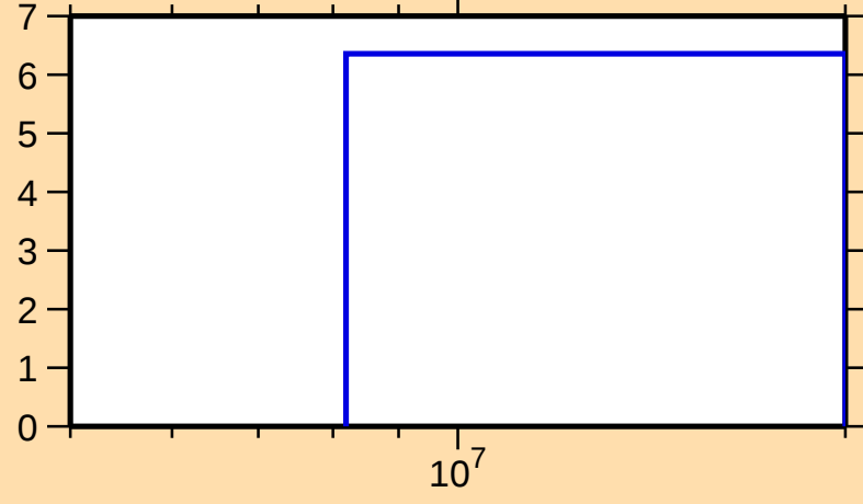
\Delta\sigma/\sigma vs. E for ^{95}\text{Ag}(n,\text{tot.})
