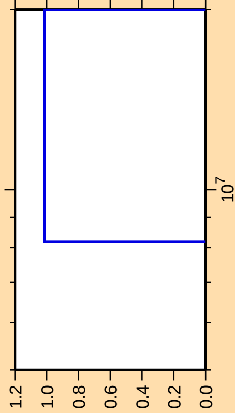
\Delta\sigma/\sigma vs. E for ^{95}\text{Ag}(n,2np)
