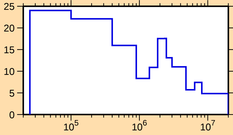
\Delta\sigma/\sigma vs. E for ^{95}\text{Ag}(n,\text{el.})
