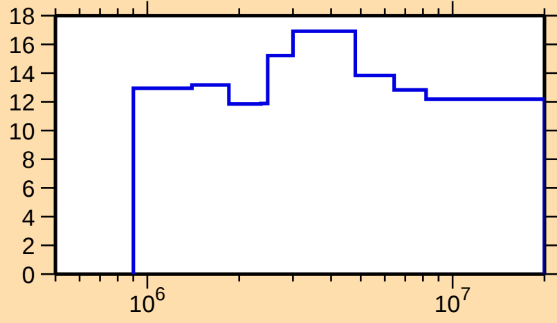
\Delta\sigma/\sigma vs. E for ^{95}\text{Ag}(n,\text{nonel.})
