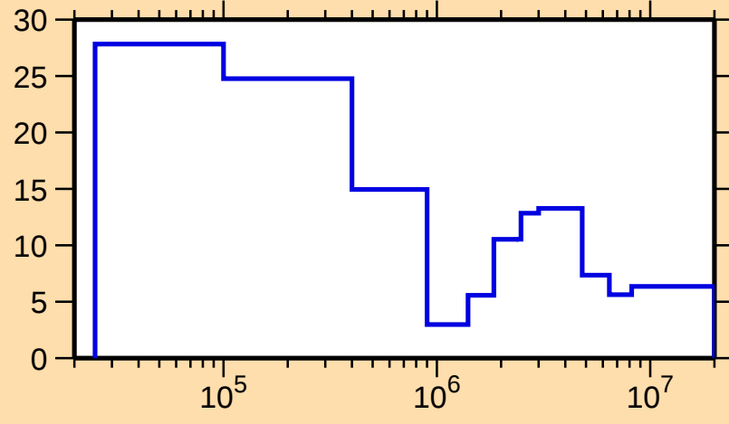
\Delta\sigma/\sigma vs. E for ^{95}\text{Ag}(n,\text{tot.})
