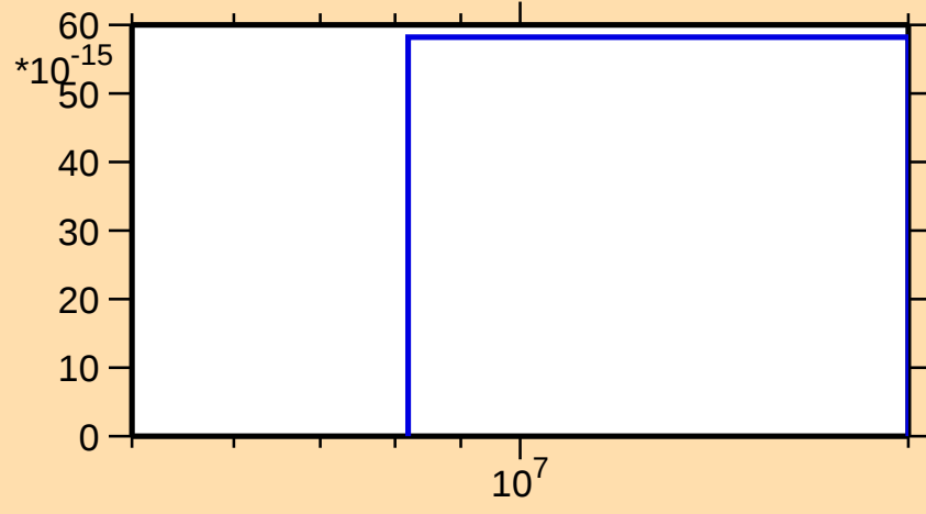
\sigma vs. E for ^{95}\text{Ag}(\text{mt } 34)
