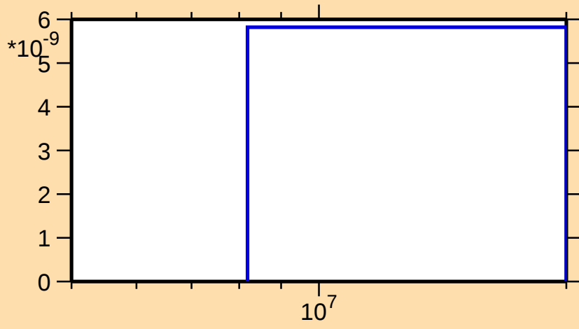
\sigma vs. E for ^{95}\text{Ag}(\text{mt } 45)
