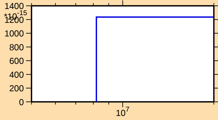
\sigma vs. E for ^{95}\text{Ag}(n,2np)
