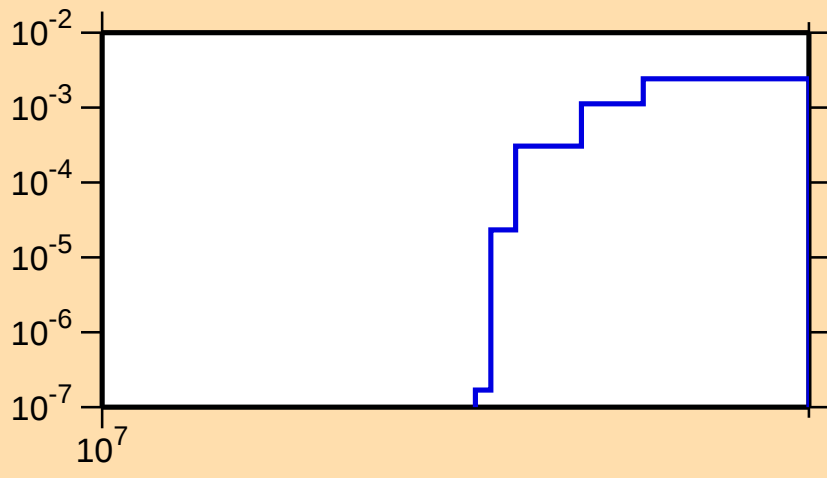
\sigma vs. E for ^{97}\text{Ag}(n,2n)
