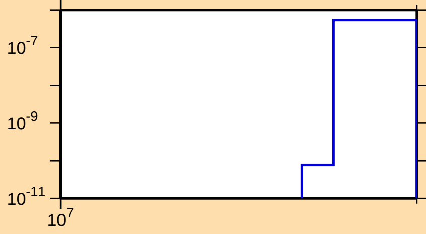
\sigma vs. E for ^{97}\text{Ag}(n,2np)
