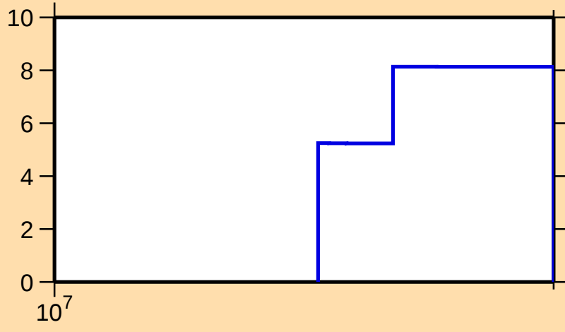
\Delta\sigma/\sigma vs. E for ^{97}\text{Ag}(n,\text{tot.})
