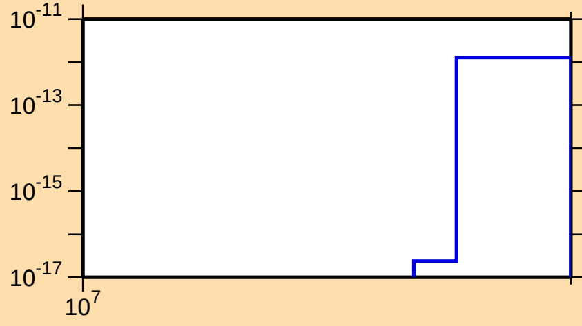
\sigma vs. E for ^{97}\text{Ag}(\text{mt } 34)
