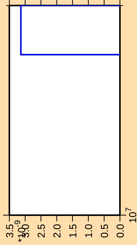
\Delta\sigma/\sigma vs. E for ^{97}\text{Ag}(n,nt)
