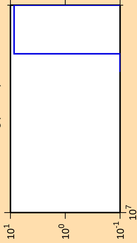
\Delta\sigma/\sigma vs. E for ^{97}\text{Ag}(\text{mt } 34)
