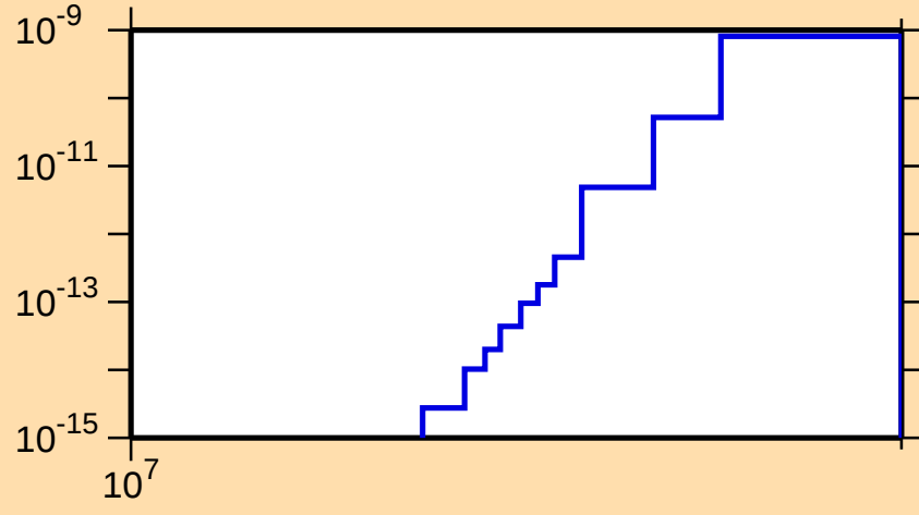
\sigma vs. E for ^{97}\text{Ag}(\text{mt117})
