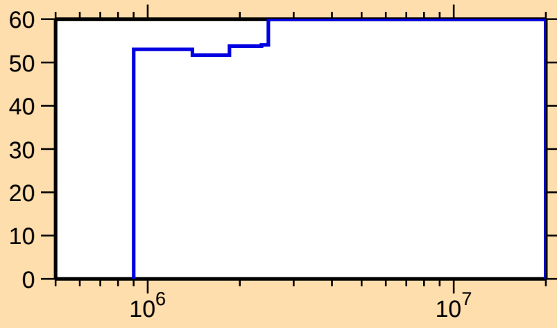
\Delta\sigma/\sigma vs. E for ^{97}\text{Ag}(n,n_1)
