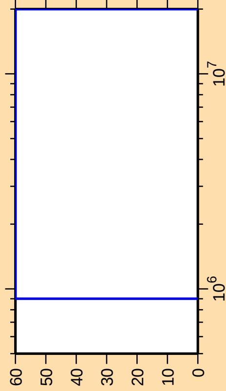
\Delta\sigma/\sigma vs. E for ^{97}\text{Ag}(n,\alpha)
