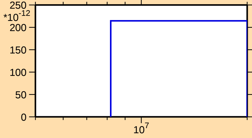
\sigma vs. E for ^{97}\text{Ag}(n,\text{nd})
