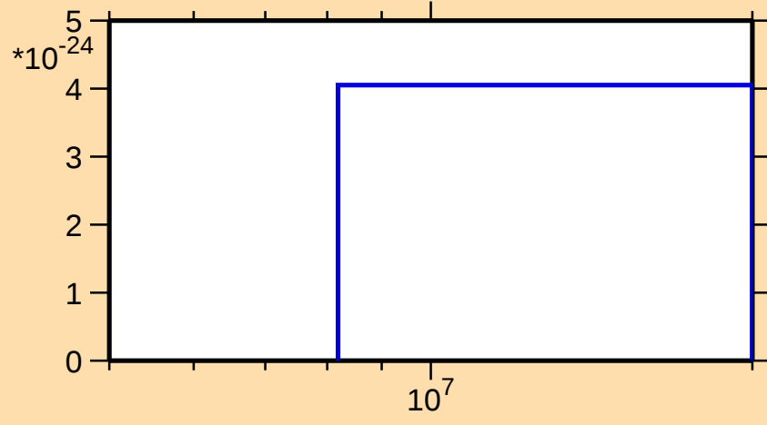
\sigma vs. E for ^{97}\text{Ag}(n,nt)
