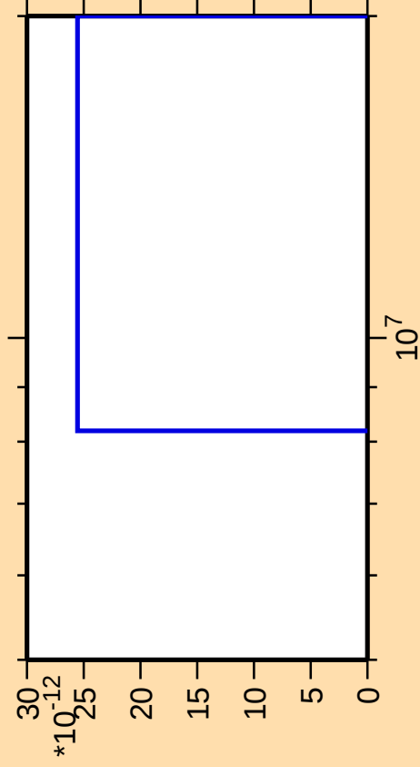
\Delta\sigma/\sigma vs. E for ^{97}\text{Ag}(n,nt)
