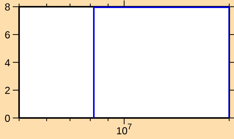
\Delta\sigma/\sigma vs. E for ^{97}\text{Ag}(n,\text{el.})
