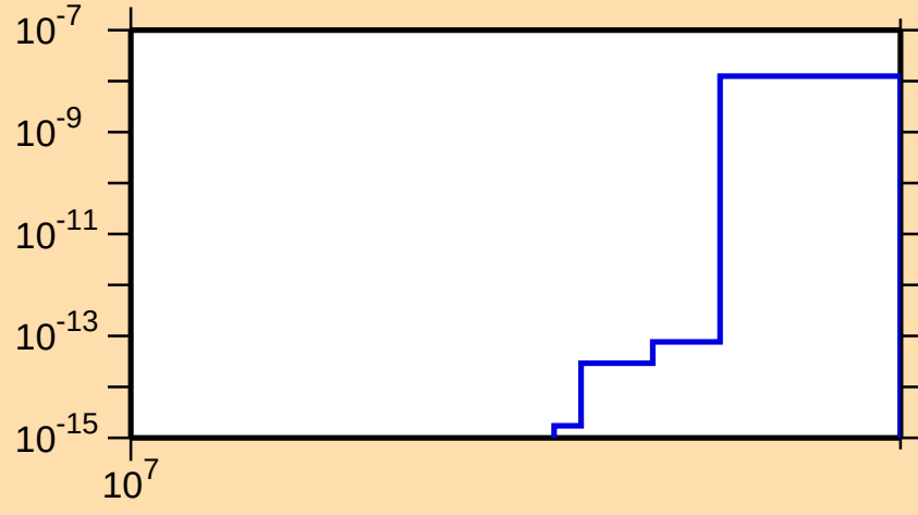
\sigma vs. E for ^{101}\text{Ag}(n,nt)
