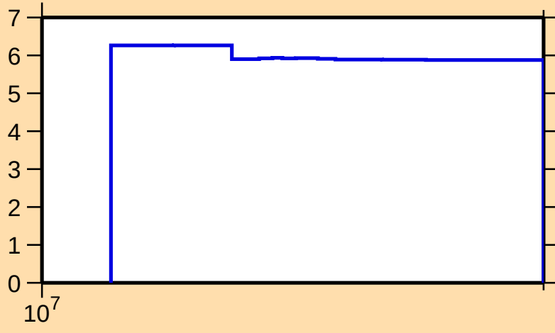
\Delta\sigma/\sigma vs. E for ^{101}\text{Ag}(n,\text{nonel.})
