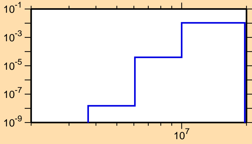
\sigma vs. E for ^{101}\text{Ag}(n,p\alpha)
