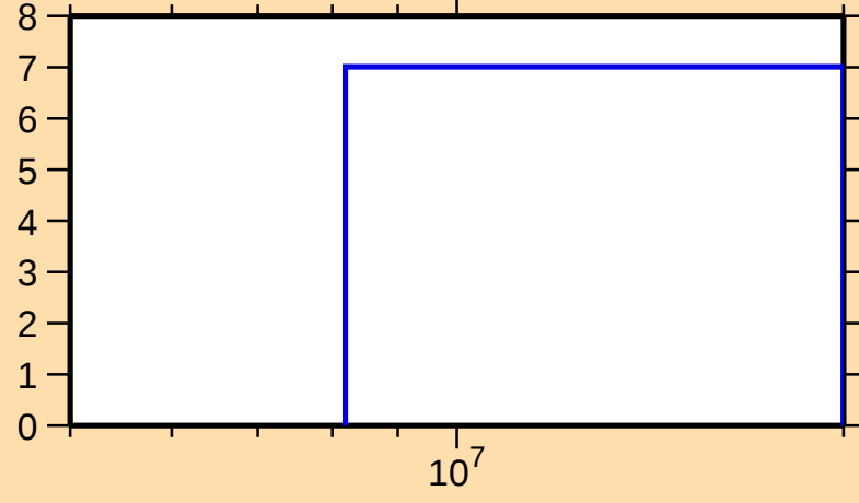
\Delta\sigma/\sigma vs. E for ^{101}\text{Ag}(n,\text{el.})
