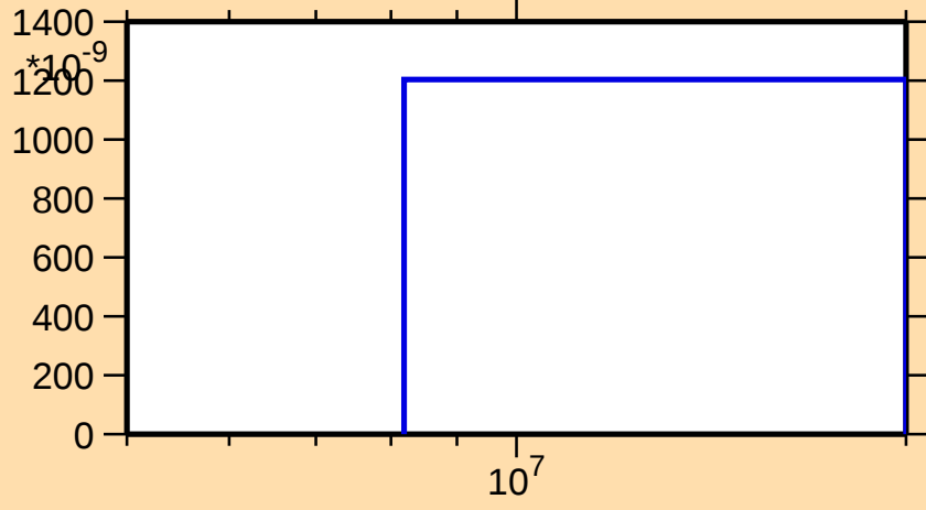
\sigma vs. E for ^{101}\text{Ag}(n,\text{nd})
