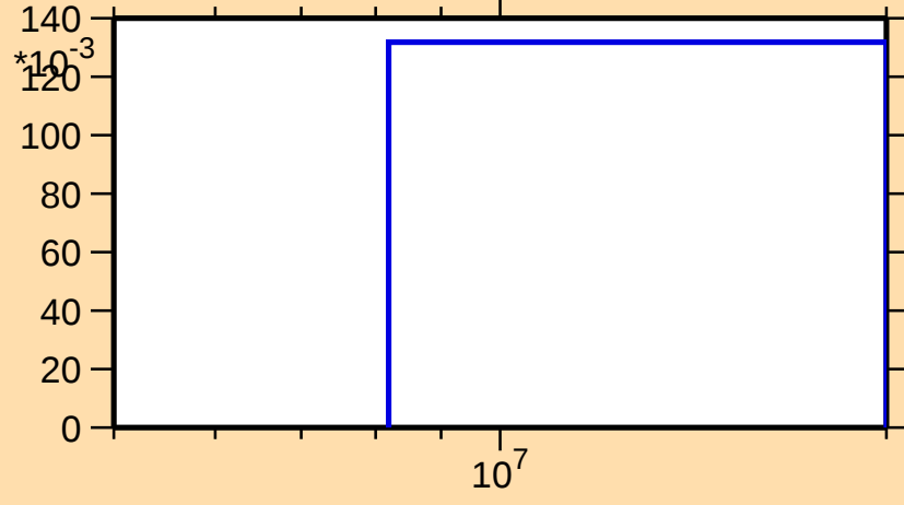
\sigma vs. E for ^{101}\text{Ag}(n,2n)
