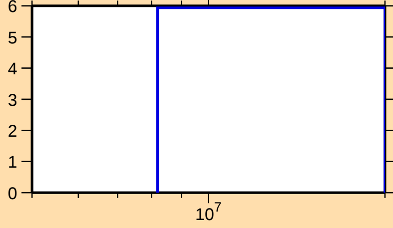
\Delta\sigma/\sigma vs. E for ^{101}\text{Ag}(n,\text{nonel.})
