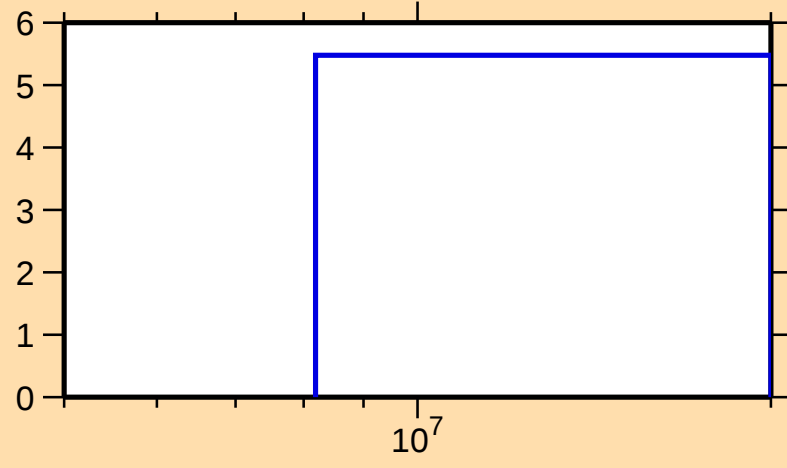
\Delta\sigma/\sigma vs. E for ^{101}\text{Ag}(n,\text{tot.})
