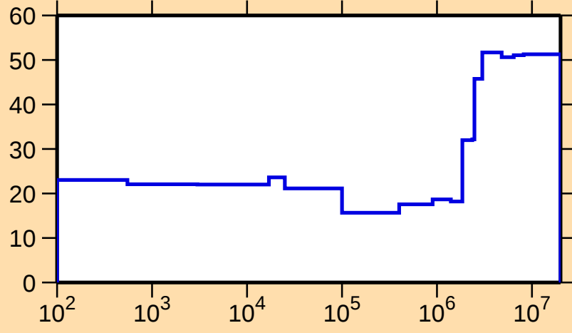
\Delta\sigma/\sigma vs. E for ^{101}\text{Ag}(n,n_1)
