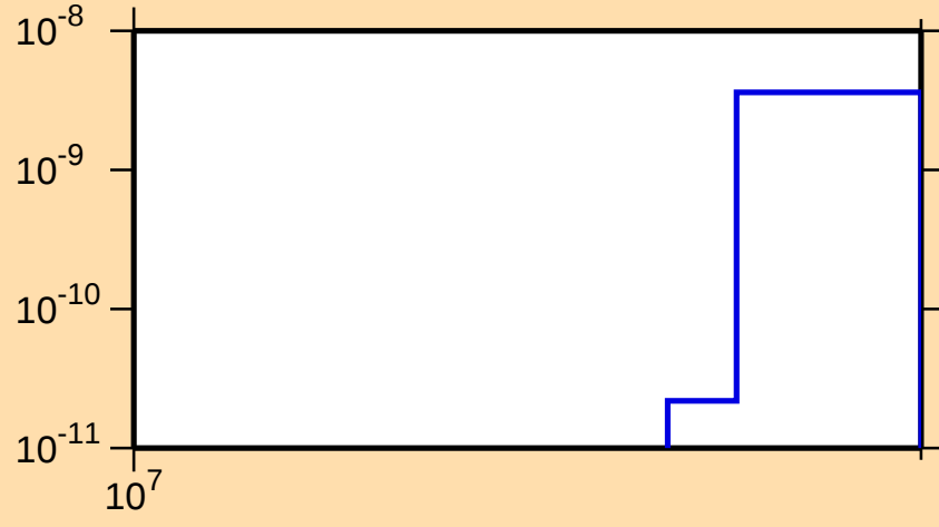
\sigma vs. E for ^{104}\text{Ag}(n,\text{pd})
