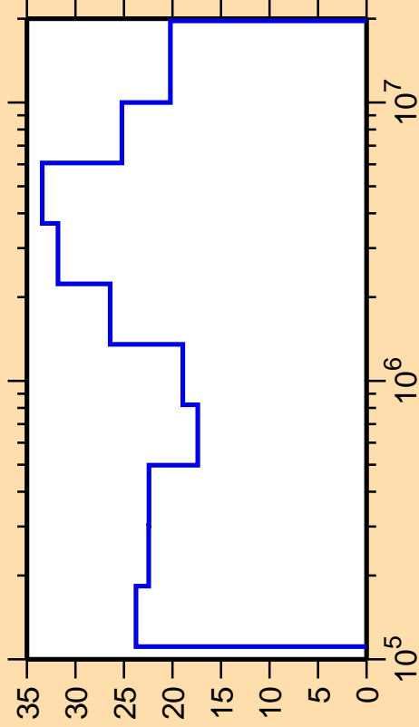
\Delta\sigma/\sigma vs. E for ^{104}\text{Ag}(n,n_4)
