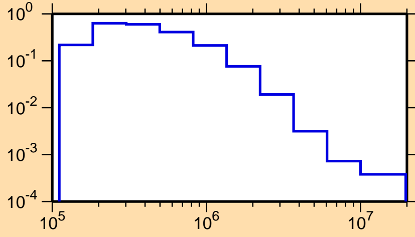
\sigma vs. E for ^{104}\text{Ag}(n,n_3)
