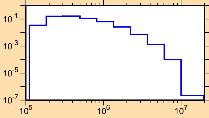
\sigma vs. E for ^{104}\text{Ag}(n,n_4)
