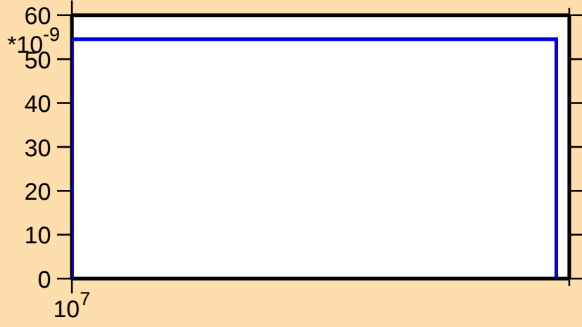
\sigma vs. E for ^{104}\text{Ag}(n,2n\alpha)
