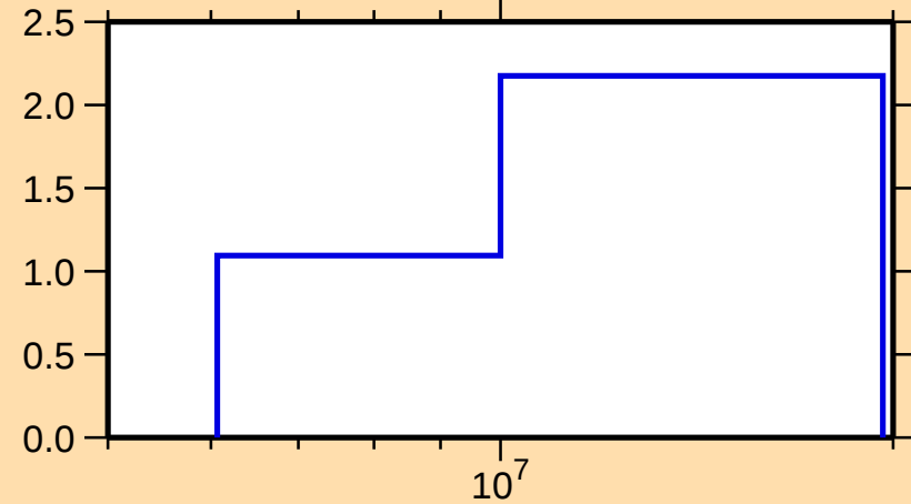
\Delta\sigma/\sigma vs. E for ^{104}\text{Ag}(n,\text{tot.})
