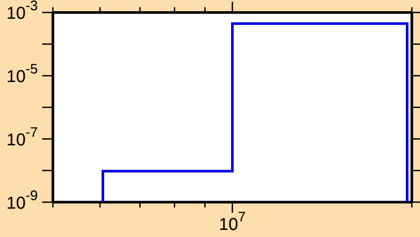
\sigma vs. E for ^{104}\text{Ag}(n,t)
