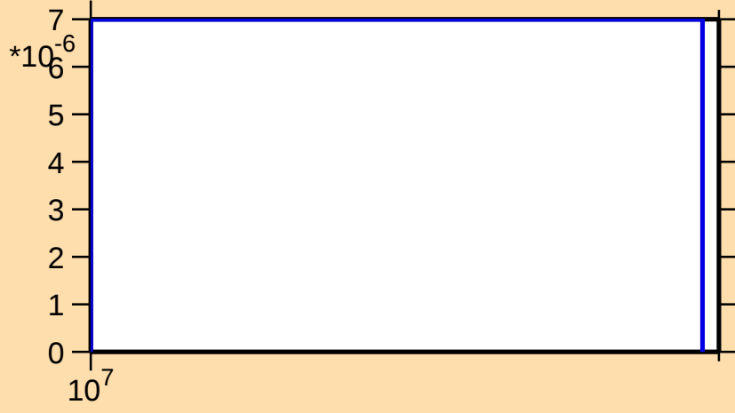
\sigma vs. E for ^{104}\text{Ag}(n,\text{nd})
