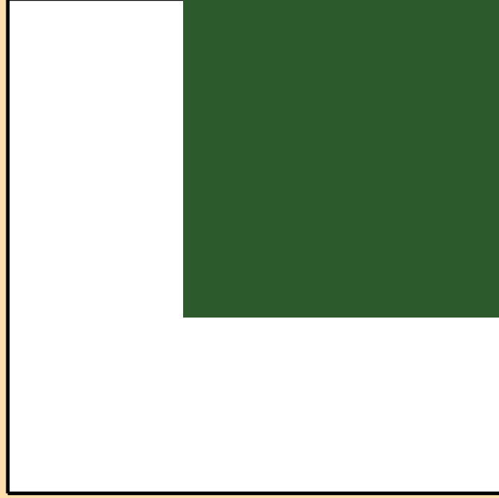
\sigma vs. E for ^{104}\text{Ag}(n,\text{pt})
