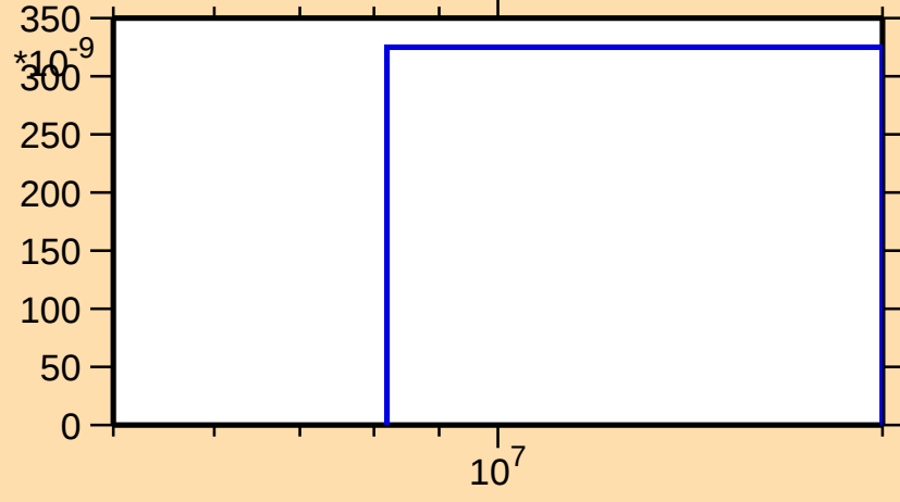
\sigma vs. E for ^{104}\text{Ag}(n,3n)
