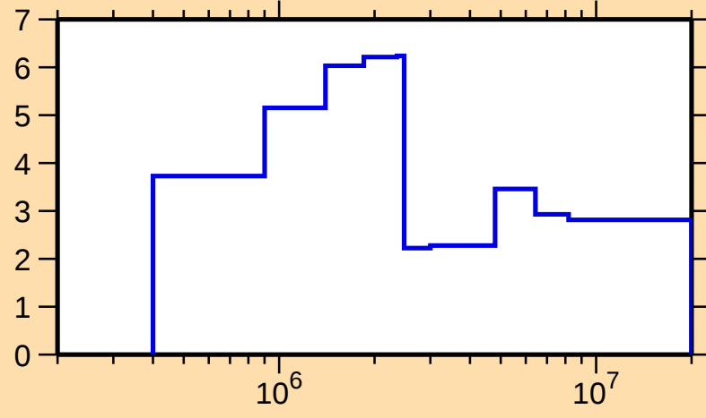
\Delta\sigma/\sigma vs. E for ^{104}\text{Ag}(n,\text{el.})
