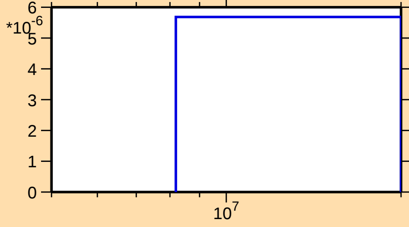
\sigma vs. E for ^{104}\text{Ag}(n,\text{nd})
