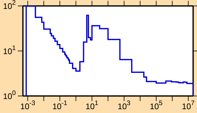
\sigma vs. E for ^{104}\text{Ag}(n,\text{nonel.})
