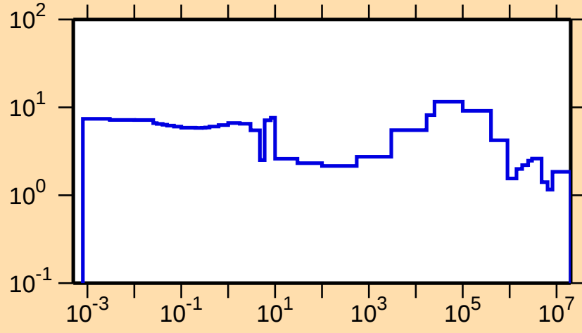
\Delta\sigma/\sigma vs. E for ^{104}\text{Ag}(n,\text{tot.})
