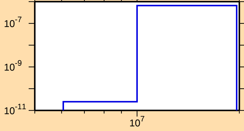
\sigma vs. E for ^{106}\text{Ag}(n,p\alpha)
