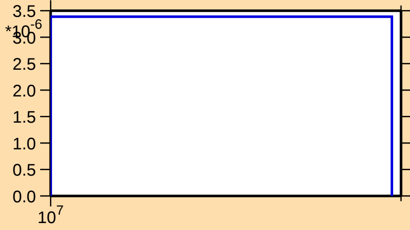
\sigma vs. E for ^{106}\text{Ag}(n,\text{nd})
