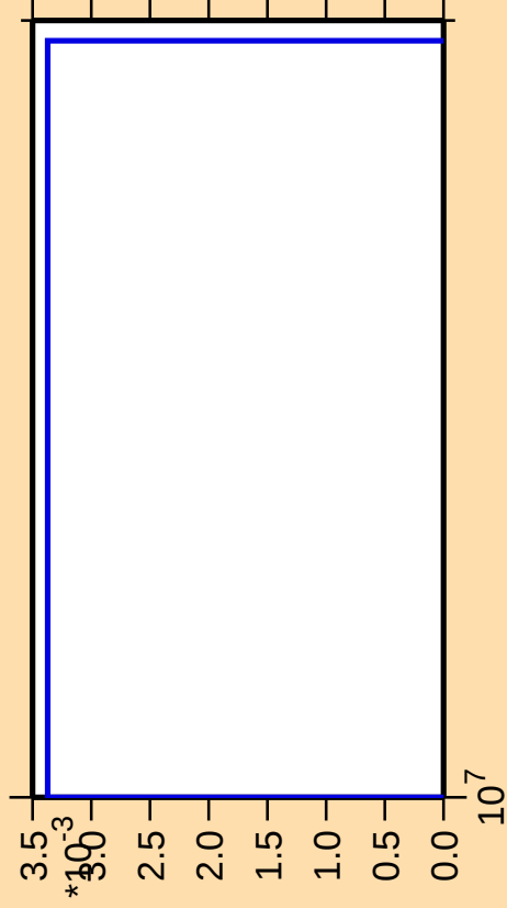
\Delta\sigma/\sigma vs. E for ^{106}\text{Ag}(n,\text{pt})
