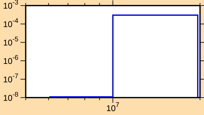
\sigma vs. E for ^{106}\text{Ag}(n,t)
