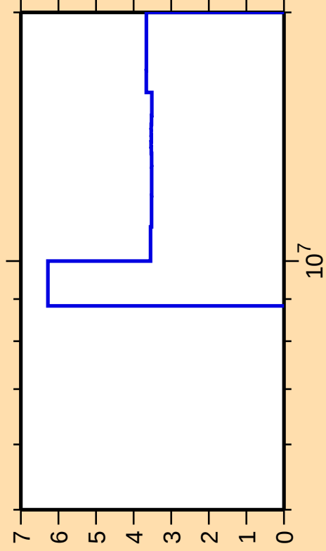
\Delta\sigma/\sigma vs. E for ^{107}\text{Ag}(n,2n)
