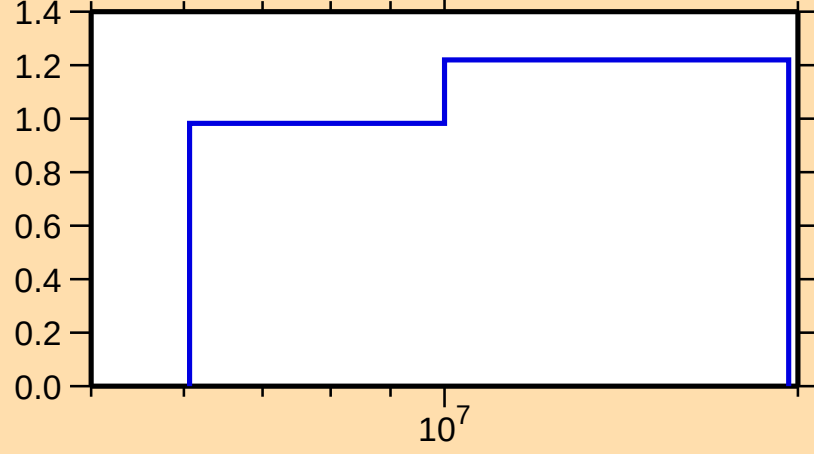
\Delta\sigma/\sigma vs. E for ^{107}\text{Ag}(n,\text{tot.})
