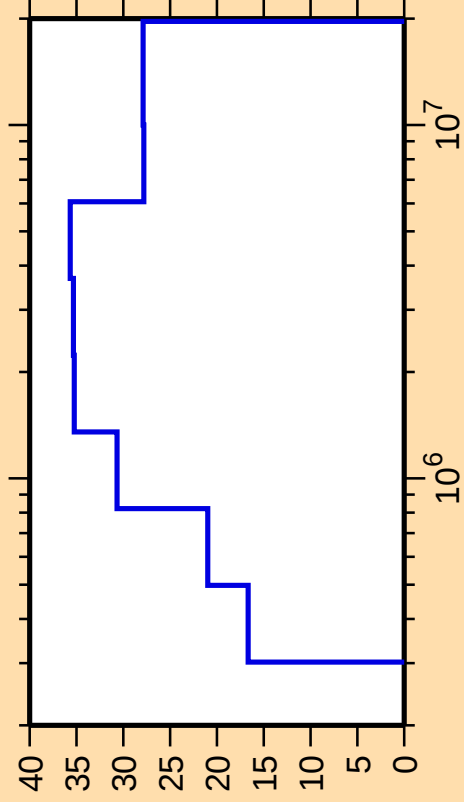
\Delta\sigma/\sigma vs. E for ^{108}\text{Ag}(n,\gamma)
