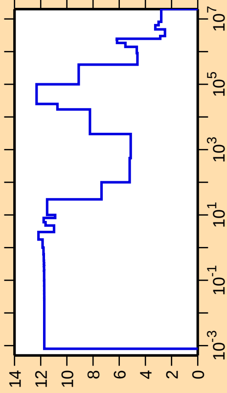
\Delta\sigma/\sigma vs. E for ^{108}\text{Ag}(n,\text{el.})
