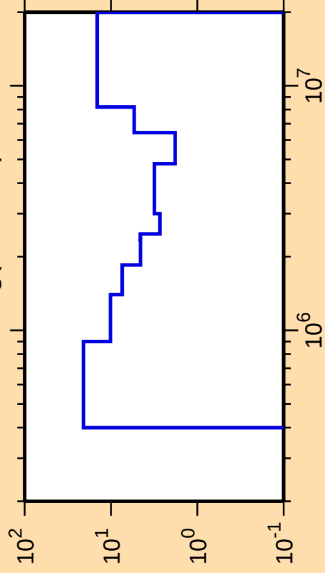
\Delta\sigma/\sigma vs. E for ^{108}\text{Ag}(n,\text{ncont.})
