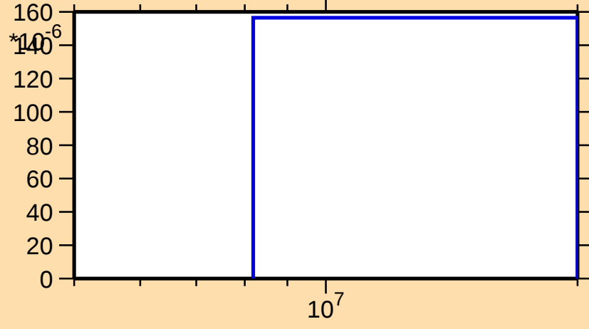
\sigma vs. E for ^{108}\text{Ag}(n,3n)
