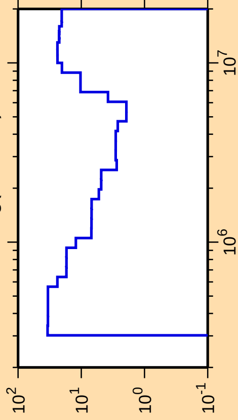
\Delta\sigma/\sigma vs. E for ^{110}\text{Ag}(n,n\text{cont.})
