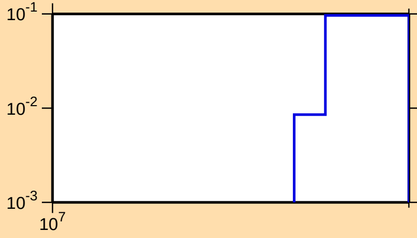
\sigma vs. E for ^{110}\text{Ag}(n,3n)
