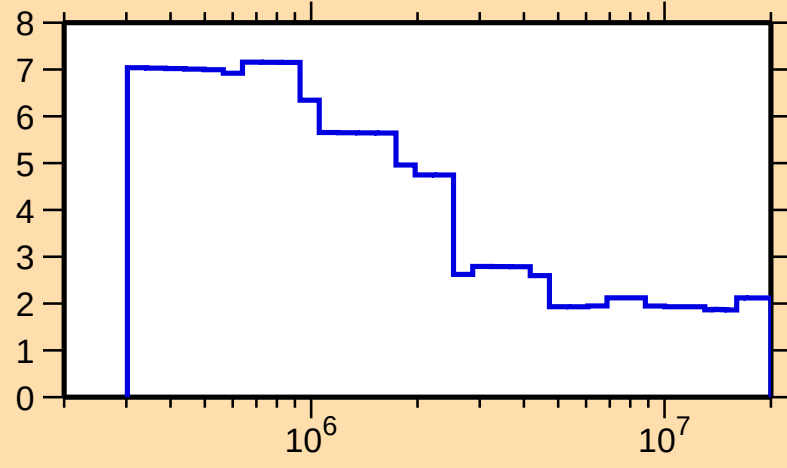
\Delta\sigma/\sigma vs. E for ^{110}\text{Ag}(n,n\text{onel.})
