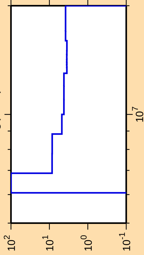
\Delta\sigma/\sigma vs. E for ^{110}\text{Ag}(n,2n)
