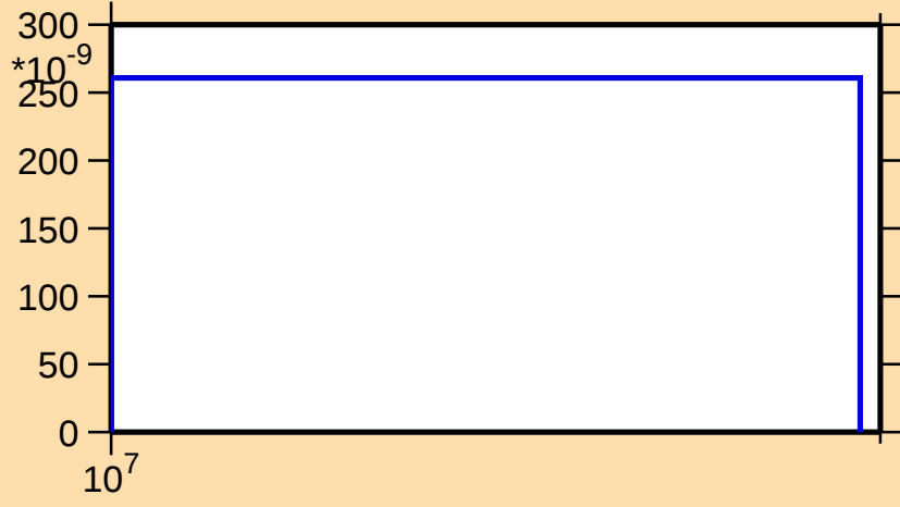
\sigma vs. E for ^{110}\text{Ag}(n,2np)
