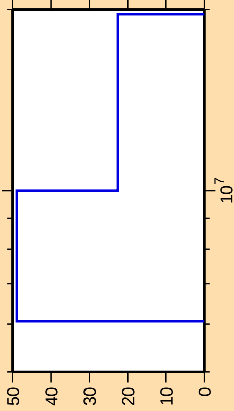
\Delta\sigma/\sigma vs. E for ^{110}\text{Ag}(n,np)
