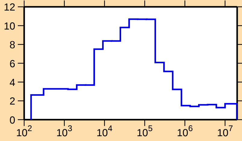
\Delta\sigma/\sigma vs. E for ^{110}\text{Ag}(n,\text{tot.})
