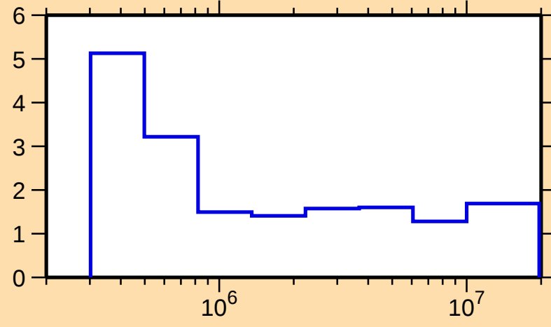
\Delta\sigma/\sigma vs. E for ^{110}\text{Ag}(n,\text{tot.})
