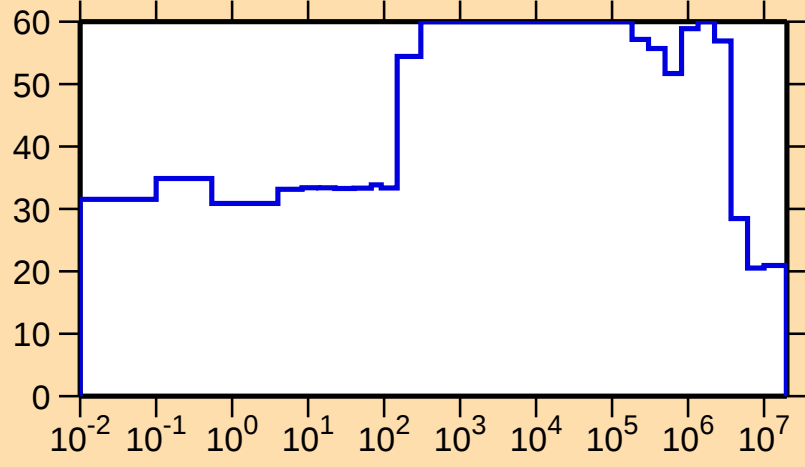
\Delta\sigma/\sigma vs. E for ^{110}\text{Ag}(n,p)
