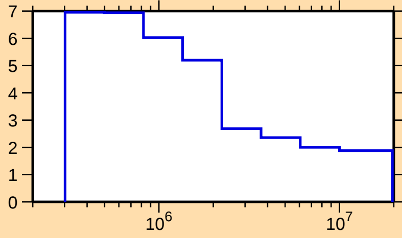
\Delta\sigma/\sigma vs. E for ^{110}\text{Ag}(n,\text{nonel.})
