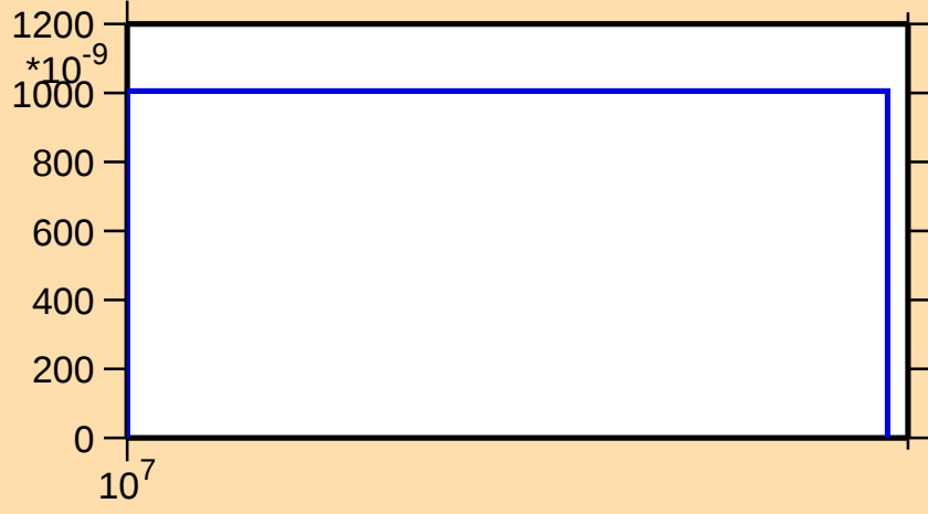
\sigma vs. E for ^{110}\text{Ag}(n,\text{nd})
