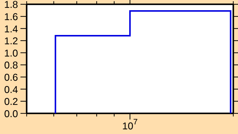
\Delta\sigma/\sigma vs. E for ^{110}\text{Ag}(n,\text{tot.})
