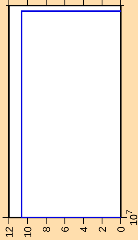
\Delta\sigma/\sigma vs. E for ^{110}\text{Ag}(n,3n)
