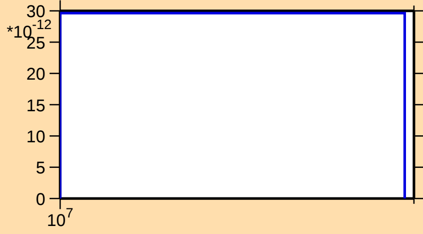
\sigma vs. E for ^{110}\text{Ag}(n,p\alpha)
