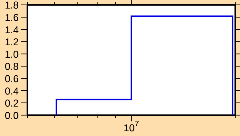
\sigma vs. E for ^{110}\text{Ag}(n,2n)
