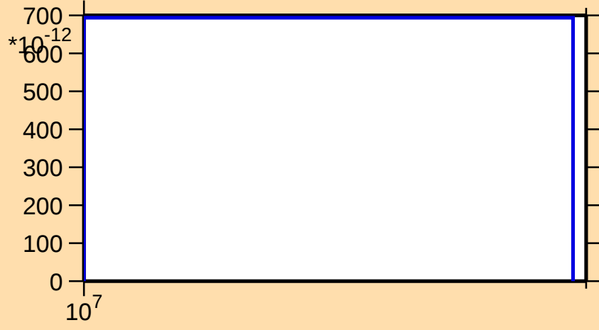
\sigma vs. E for ^{110}\text{Ag}(n,2n\alpha)
