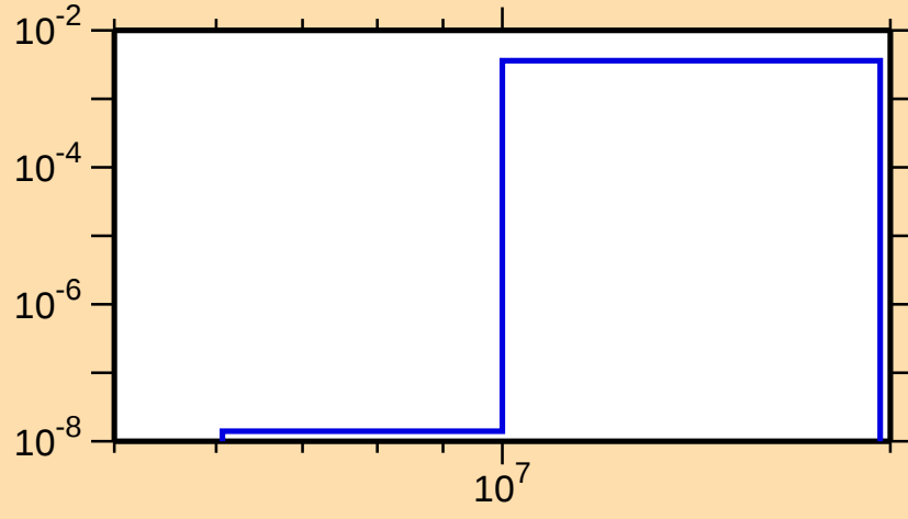
\sigma vs. E for ^{110}\text{Ag}(n,np)
