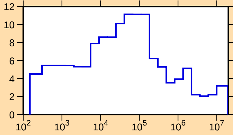
\Delta\sigma/\sigma vs. E for ^{110}\text{Ag}(n,\text{el.})
