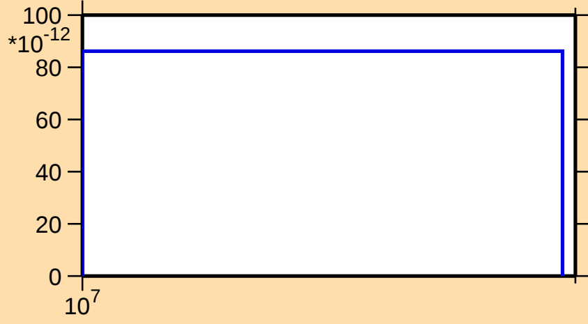
\sigma vs. E for ^{110}\text{Ag}(n,\text{He}3)
