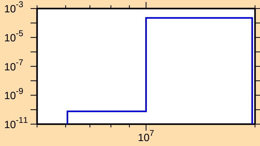
\sigma vs. E for ^{110}\text{Ag}(n,t)
