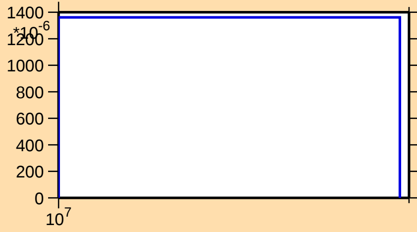
\sigma vs. E for ^{110}\text{Ag}(n,3n)
