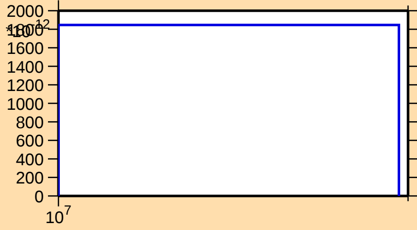
\sigma vs. E for ^{110}\text{Ag}(n,nt)
