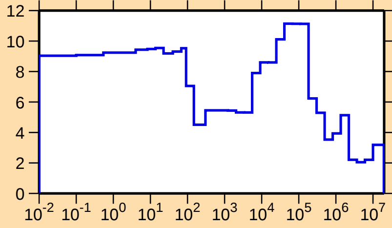
\Delta\sigma/\sigma vs. E for ^{110}\text{Ag}(n,\text{el.})
