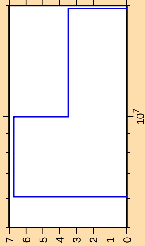
\Delta\sigma/\sigma vs. E for ^{110}\text{Ag}(n,2n)
