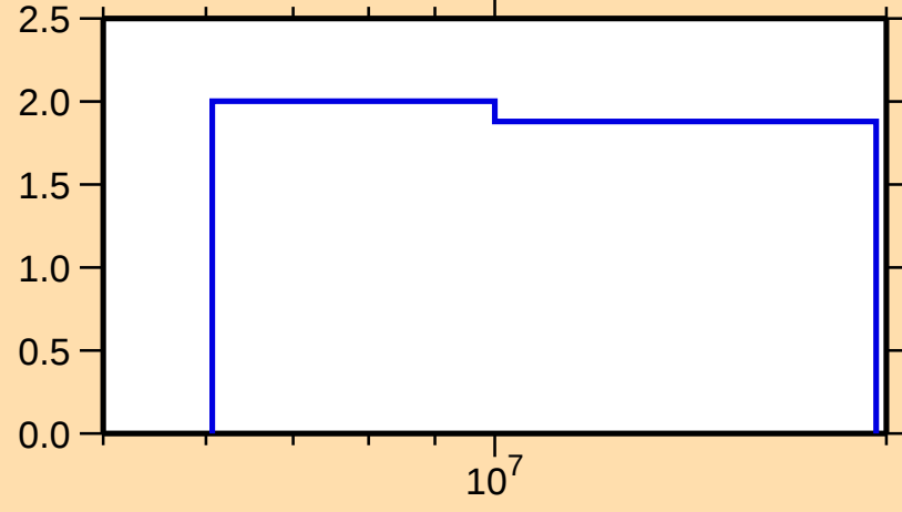
\Delta\sigma/\sigma vs. E for ^{110}\text{Ag}(n,\text{nonel.})
