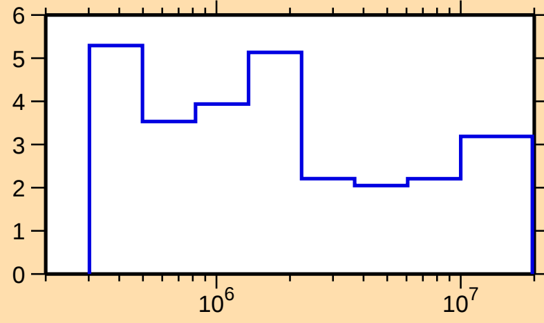
\Delta\sigma/\sigma vs. E for ^{110}\text{Ag}(n,\text{el.})
