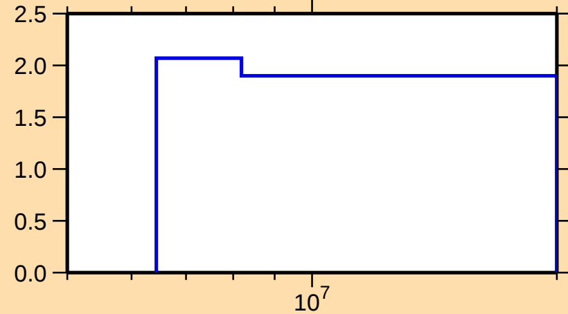
\Delta\sigma/\sigma vs. E for ^{110}\text{Ag}(n,\text{nonel.})
