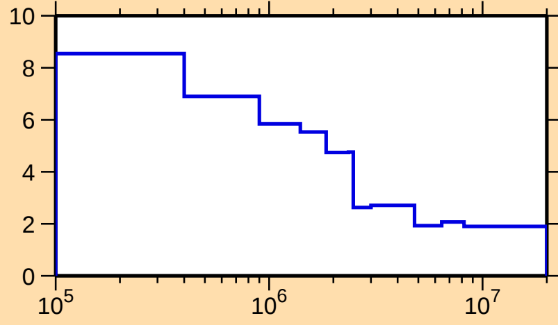
\Delta\sigma/\sigma vs. E for ^{110}\text{Ag}(n,n\text{onel.})
