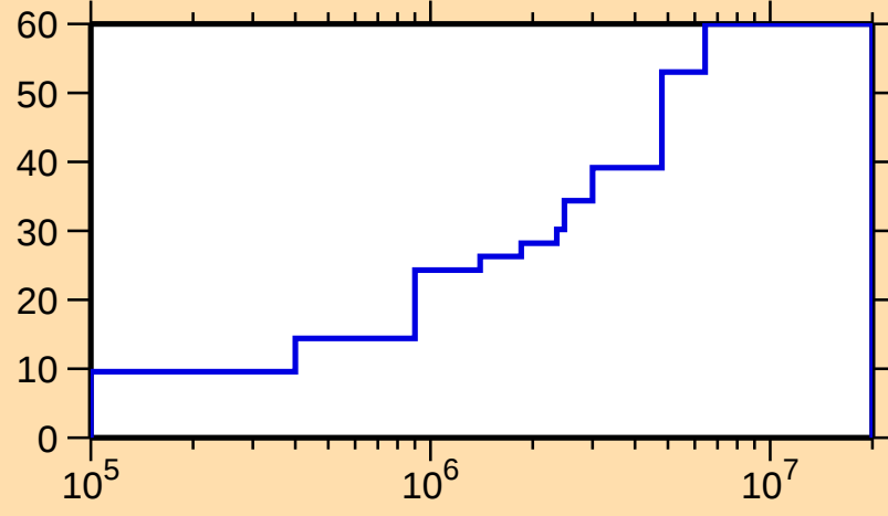
\Delta\sigma/\sigma vs. E for ^{110}\text{Ag}(n,n_1)
