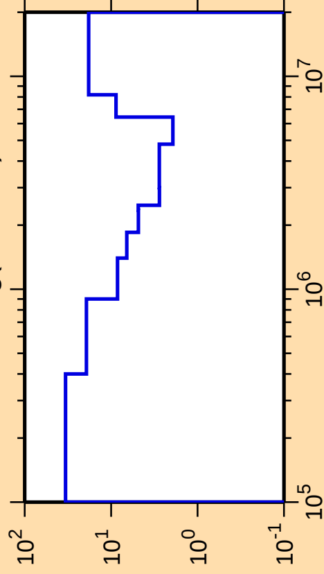
\Delta\sigma/\sigma vs. E for ^{110}\text{Ag}(n,\text{ncont.})
