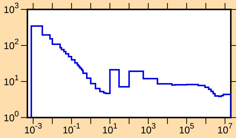
\sigma vs. E for ^{110}\text{Ag}(n,\text{tot.})
