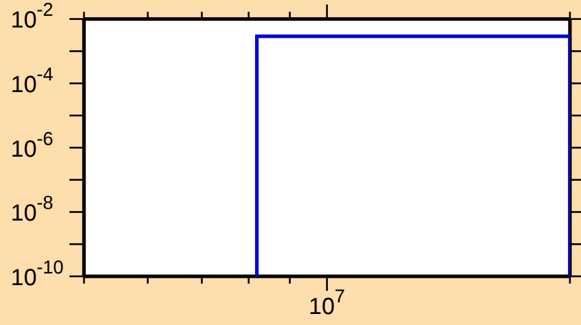
\sigma vs. E for ^{110}\text{Ag}(n,np)
