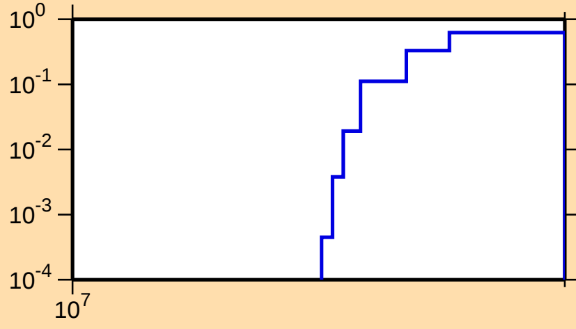
\sigma vs. E for ^{115}\text{Ag}(n,3n)
