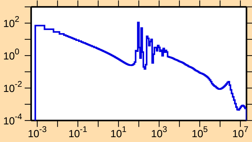
\sigma vs. E for ^{115}\text{Ag}(n,\gamma)
