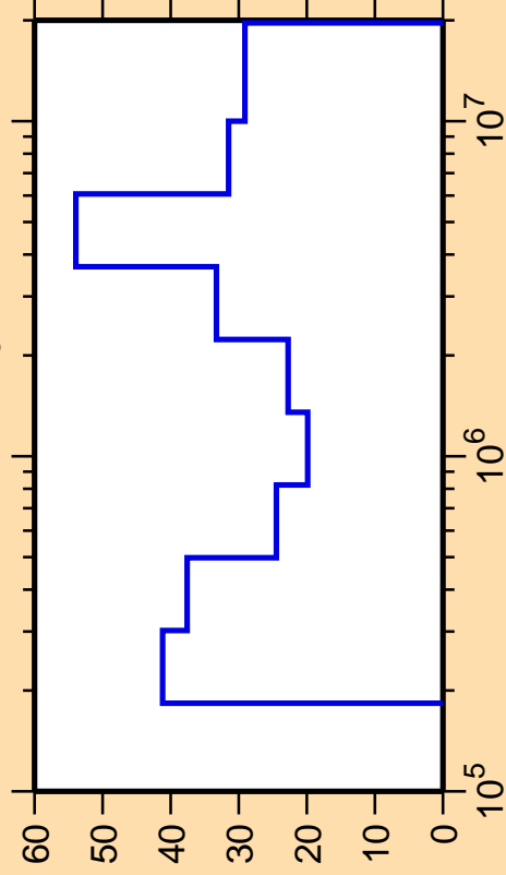
\Delta\sigma/\sigma vs. E for ^{115}\text{Ag}(n,n_3)
