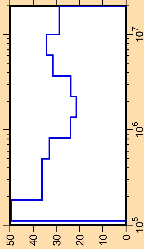
\Delta\sigma/\sigma vs. E for ^{115}\text{Ag}(n,n_2)
